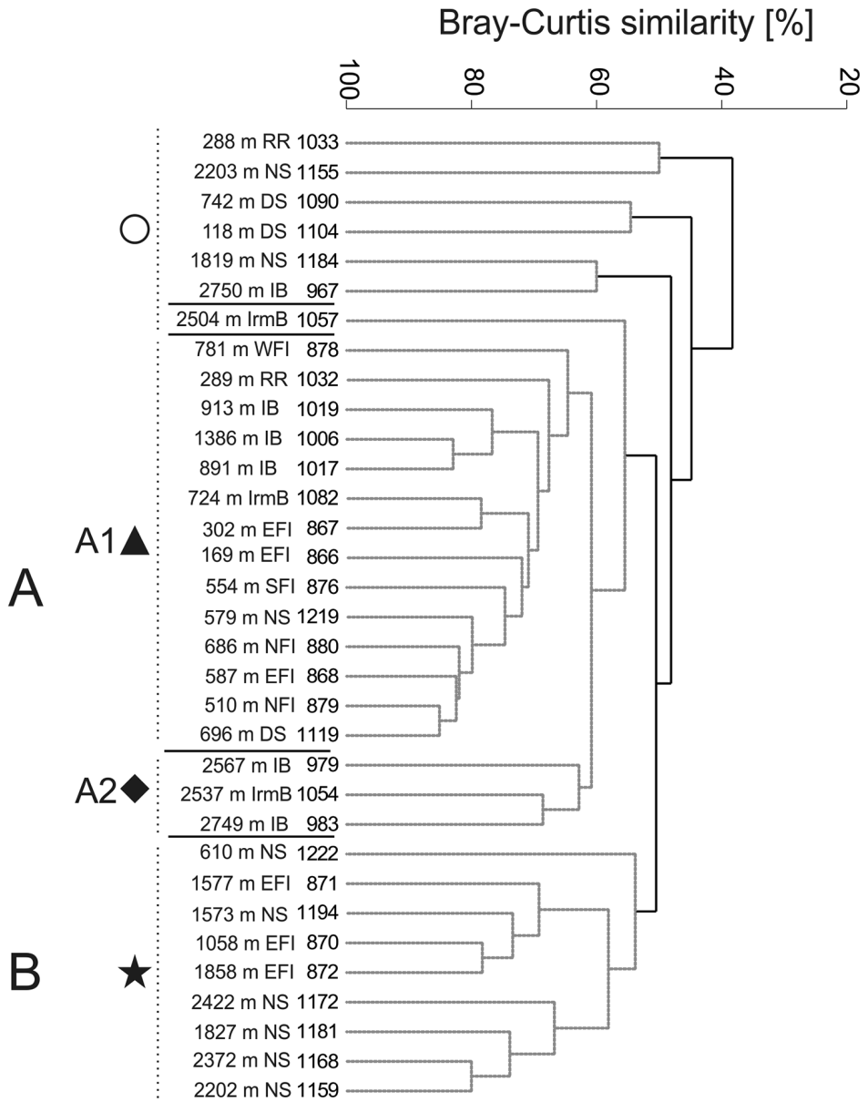
Figure 8. Dendrogram of samples for the family level data (Bray-Curtis similarity, group average grouping method and presence/absence transformed data). Abbreviations: RR - Reykjanes Ridge, NS - Norwegian Sea, DS - Denmark Strait, IB - Iceland Basin, IrmB - Irminger Basin, WFI - west off Faroe Islands, EFI - east off Faroe Islands, SFI - South of Faroe Islands, NFI - North of Faroe Islands. (Grey spotted lines indicate the samples that cannot be significantly differentiated by SIMPROF.) Regions are named based on the habitats defined by Meißner et al. (2014).
