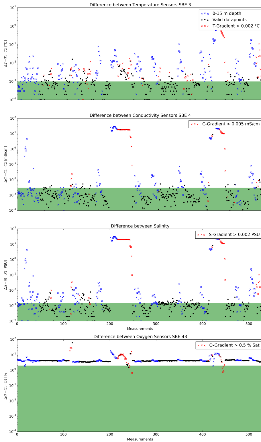
Figure 2: Data accuracy of sensor pairs HE508
