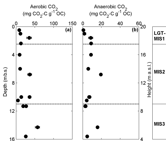
Figure 3. Depth profiles of total aerobic (a) and anaerobic (b) \text{CO}_2 production per gram of organic carbon ( \text{g}^{-1}\text{OC} ) in sediment samples from the MUO12 sequence after 134 incubation days at 4^\circ\text{C} for deposits from the Holocene interglacial (MIS 1), including the late glacial transition (LGT), the Sartan stadial (MIS 2), and the Kargin interstadial (MIS 3). Data are mean values ( n = 3 ) and error bars represent 1 standard deviation. Note the different scales. No \text{CH}_4 production was observed during the 134-day incubation period.
