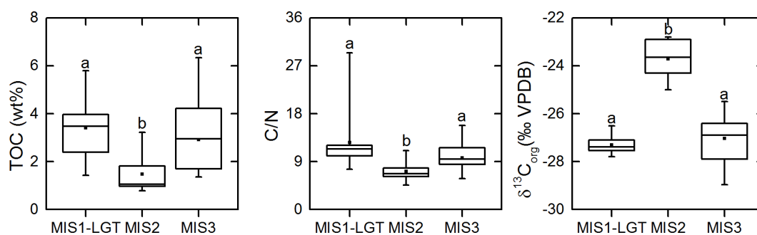
Figure 2. Box plot of total organic carbon (TOC), total organic carbon to total nitrogen ratio (C/N), and \delta^{13}\text{C}_{\text{org}} values of permafrost deposits from the MUO12 sequence, the BK8 core, and the two L14 cores from the Holocene interglacial (MIS 1), including the late glacial transition (LGT) ( n = 12 ), the Sartan stadial (MIS 2) ( n = 6 ), and the Kargin interstadial (MIS 3) ( n = 27 ). The whiskers show the data range and the box indicates the interquartile range. The vertical line and square inside the boxes show the median and mean, respectively. The letters above the whiskers indicate statistically significant differences in geochemical characteristics between the deposits of different ages (Mann–Whitney test, p < 0.016 for TOC and C/N, p < 0.001 for \delta^{13}\text{C}_{\text{org}} ).
