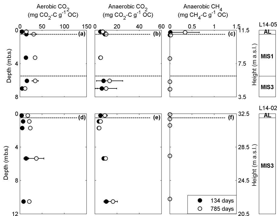
Figure 5. Depth profiles of total aerobic CO 2 (a), anaerobic CO 2 (b), and anaerobic CH 4 (c) production per gram of organic carbon (g -1 OC) in sediment samples from the L14-05 (a–c), and L14-02 cores (d–f) after 134 (closed symbols) and 785 (open symbols) incubation days at 4 °C for the active layer (AL), which is considered to be 0.5 m thick, and permafrost deposits from the Holocene interglacial (MIS 1) and the Kargin interstadial (MIS 3). Data are mean values ( n = 3) and error bars represent 1 standard deviation. Note the different scales.
