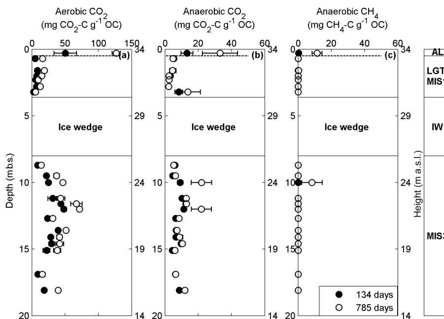
Figure 4. Depth profiles of total aerobic CO 2 (a), anaerobic CO 2 (b), and anaerobic CH 4 (c) production per gram of organic carbon (g -1 OC) in sediment samples from the BK8 core after 134 (closed symbols) and 785 (open symbols) incubation days at 4 °C for the active layer (AL), which is considered to be 0.5 m thick, and permafrost deposits from the Holocene interglacial (MIS 1), including the late glacial transition (LGT) and the Kargin interstadial (MIS 3). Data are mean values ( n = 3 ) and error bars represent 1 standard deviation. Note the different scales.
