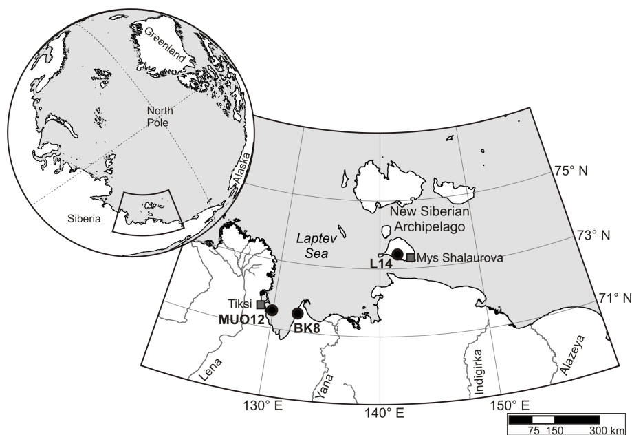
Figure 1. Overview of the Laptev Sea region with the study locations at Muostakh Island (sample code MUO12), the Buor Khaya Peninsula (BK8) and Bol'shoi Lyakhovskiy Island (L14).
