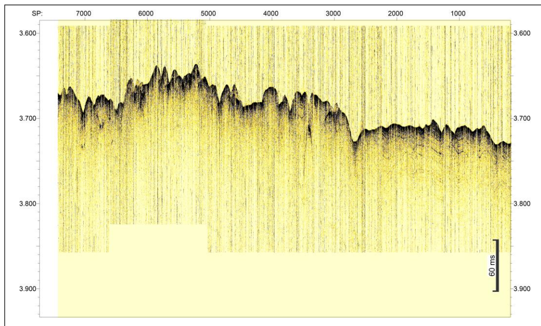
Fig. 5.8 Facies type one: hummocky surface with up to 15 m of penetration on Falkland Plateau. Shown is the SLF on seismic line AWI20190009 acquired on the 25 th of February 2019 between 20:45 to 24:00 UTC (SP=shotpoint).
