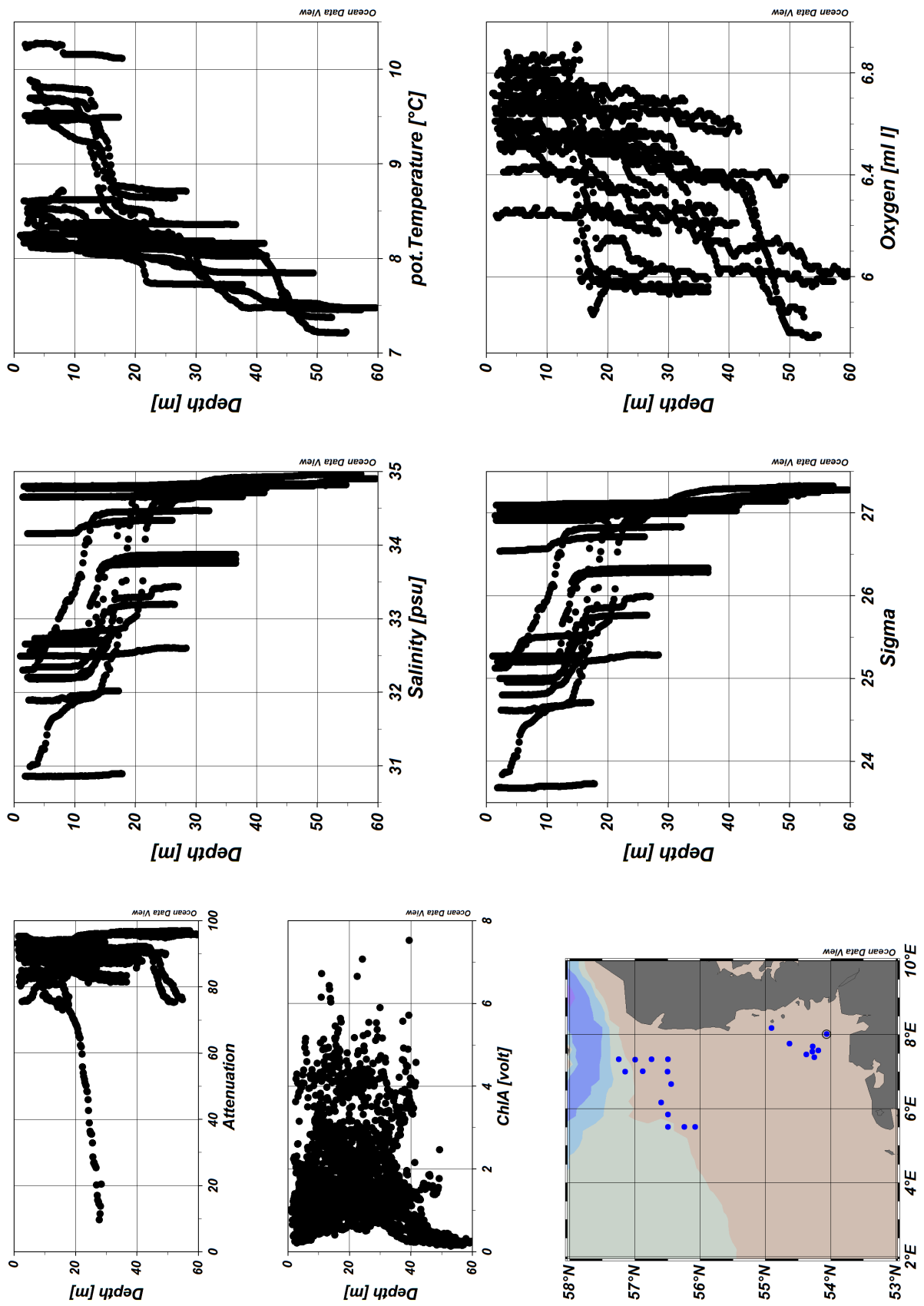
Figure 4: ODV Screenshot of HE532 CTD data
