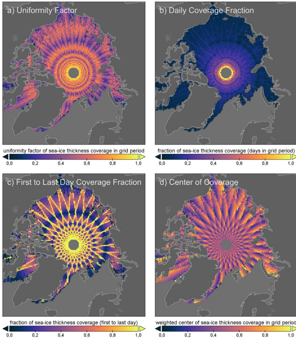
Figure 10: Temporal coverage statistics of sea-ice thickness per grid cell.
