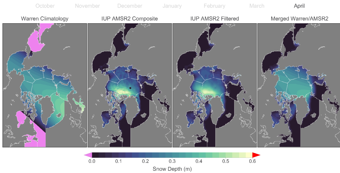
Figure 6: Steps to create a monthly merged snow depth climatology from the Warren snow climatology and monthly composites of snow depth fields derived from AMSR2 brightness temperatures by IUP Bremen. Example April, from left to right: 1) Warren snow climatology, 2) Monthly IUP snow composite from daily data, 3) Low-pass filtered IUP data and 4) merged Warren/AMSR2 with regional weighting factor
