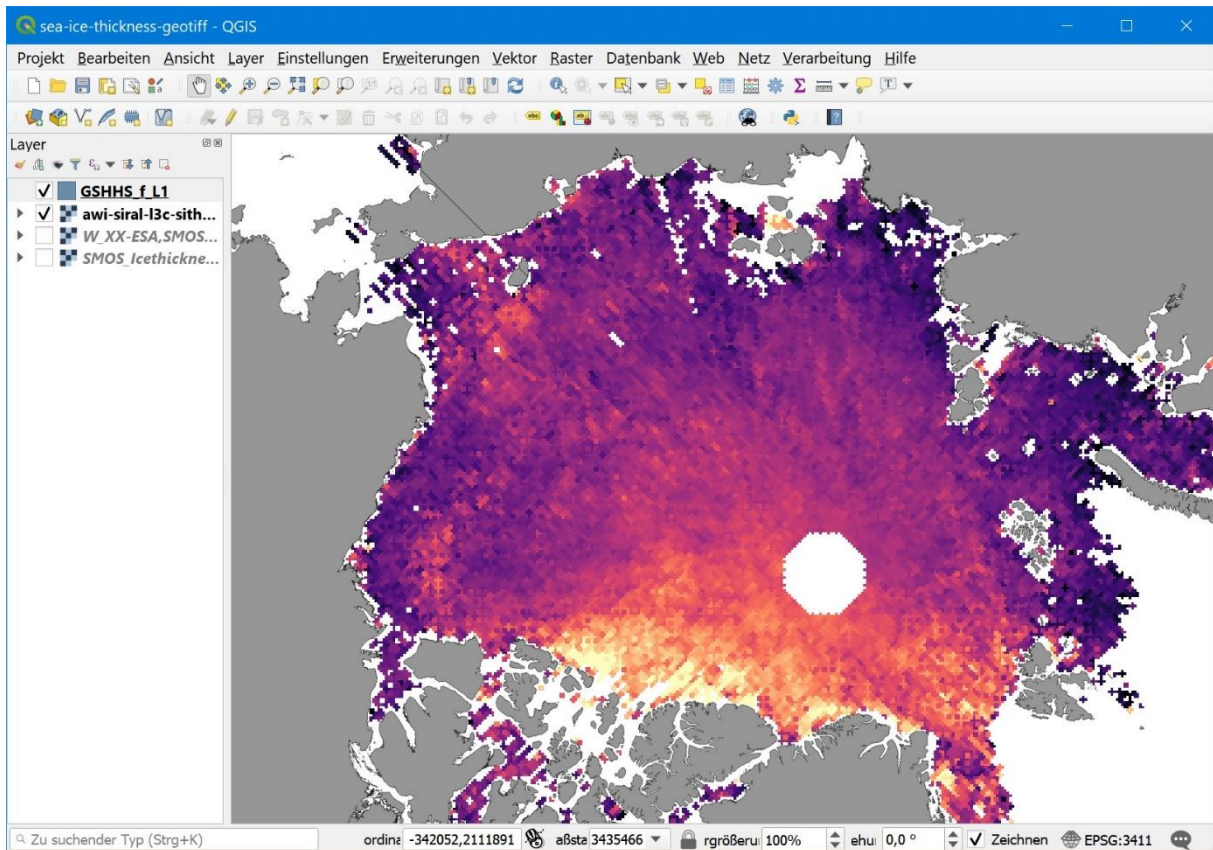
Figure 13: Visualization of sea-ice thickness geotiff file in a geographic information system (GIS)
