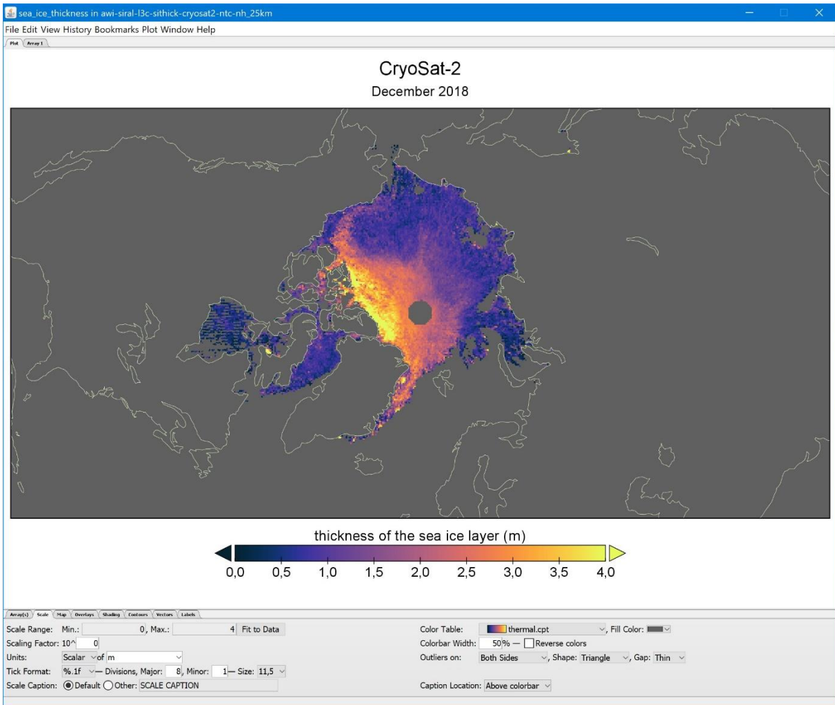
Figure 12: Visualization of a monthly gridded (l3c) sea-ice thickness field with panoply.
