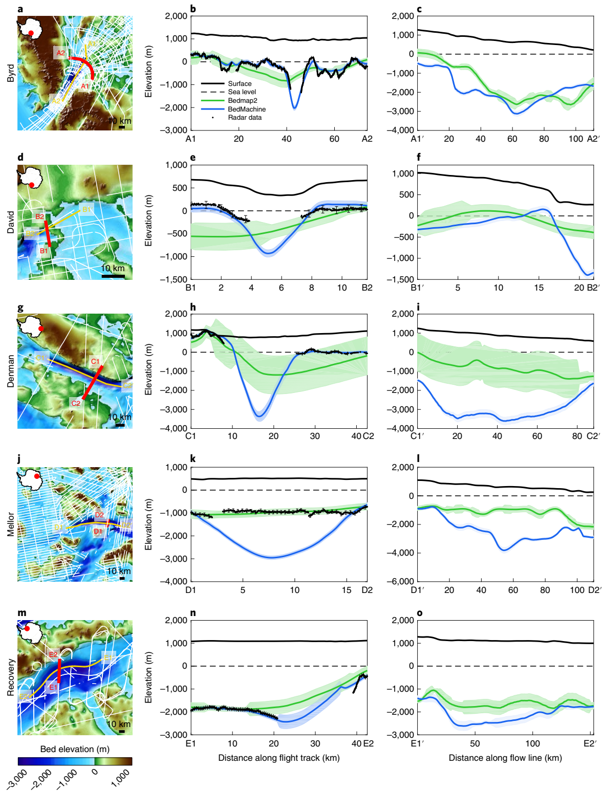
Fig. 3 | Comparison with previous datasets and radar data. a,d,g,j,m , Bed elevations of Byrd ( a ), David ( d ), Denman ( g ), Mellor ( j ) and Recovery ( m ) glaciers, colour coded between -3,000 m and 1,500 m above sea level, with radar profiles shown as white lines where bed reflections were detected. The yellow and red lines (for example, A1–A2 and A1'–A2' in a , and so on) show the locations where the profiles in the middle ( b,e,h,k,n ) and right ( c,f,i,l,o ) columns are extracted. The second column shows the profiles along the red line, which corresponds to a flight line, and the third column shows profiles along the yellow line (along flow). The solid black line shows the surface elevation along the transect, the dashed black line is sea level, the solid blue line is the bed elevation from BedMachine (with the associated uncertainty in light blue) and the green line is the bed topography from Bedmap2 (with the associated uncertainty in light green). The black dots and black error bars in the panels of the second column show the radar-derived bed elevation and associated uncertainty, respectively.
