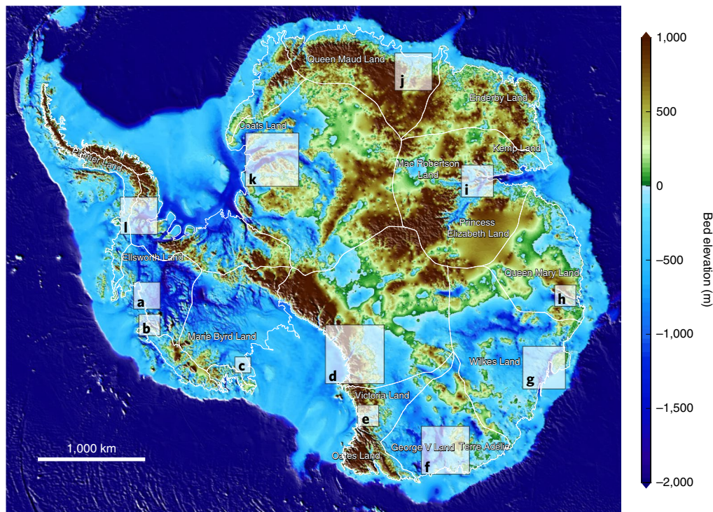
Fig. 1 | Bed elevation of the Antarctic ice sheet colour coded between -2,000 and 1,000 m above sea level. The white lines delineate the basins 15 from the ice sheet mass balance inter-comparison exercise (IMBIE). Regions marked a–l are explored in Fig. 2.
