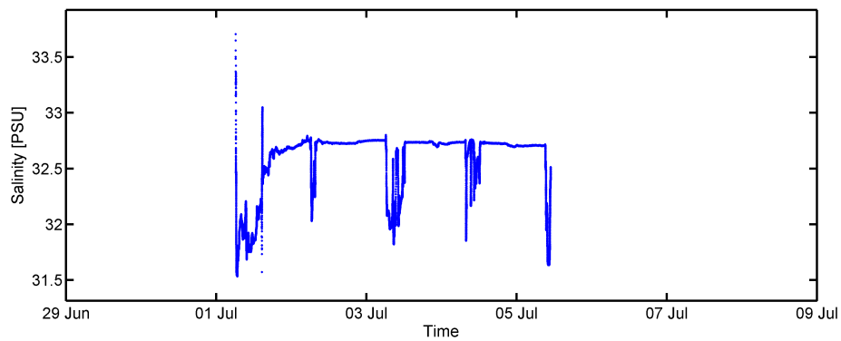
Figure 3: Raw salinity data.
