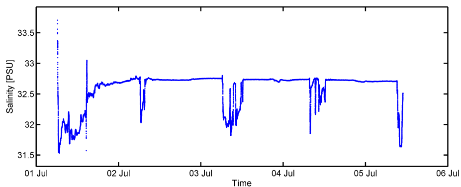
Figure 5: Salinity after flow rate filter.
