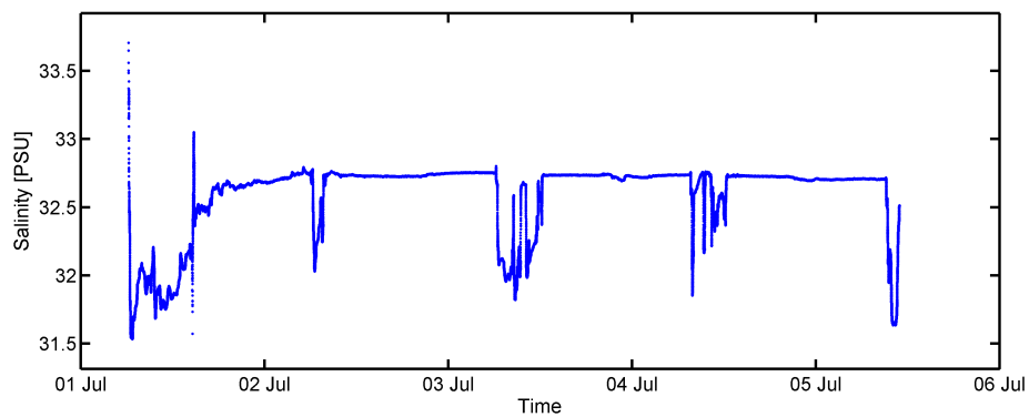
Figure 4: Salinity after basic filter.
