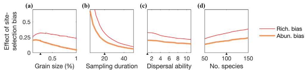
Figure 5. Impact of site-selection bias over a gradient in (a) grain size (i.e., size of sampling unit as percentage of total landscape area, based on the same data as for Fig. 4c), (b) sampling duration (i.e., number of sampling time points), (c) species' dispersal ability (maximum number of cells crossed by individuals between sampling events), and (d) total number of species in the landscape (i.e., size of regional species pool) (lines, median of 10,000 independent simulations; black triangle, default value).
