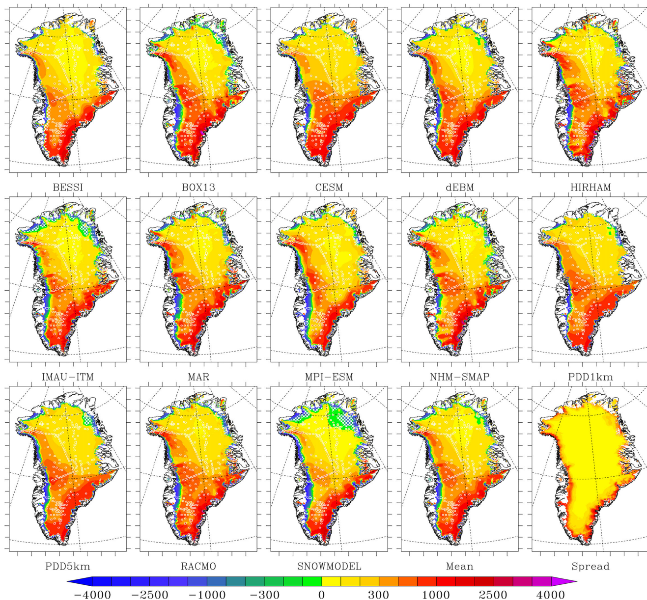
Figure 1. Mean SMB (in \text{mm w.e. yr}^{-1} ) over 1980–2012 simulated by the 13 models as well as the ensemble model mean and the spread around this mean. The SMB measurements (ice cores + PROMICE) used to evaluate the models are represented as white circles. The areas listed in Table 4 where SMB disagree with the satellite-derived bare ice area are shown in a hatched area. Finally, it is important to note that for better visibility, the scale is not linear as it uses a step of 100 for absolute values lower than 500 \text{ mm w.e. yr}^{-1} and a step of 500 above.
