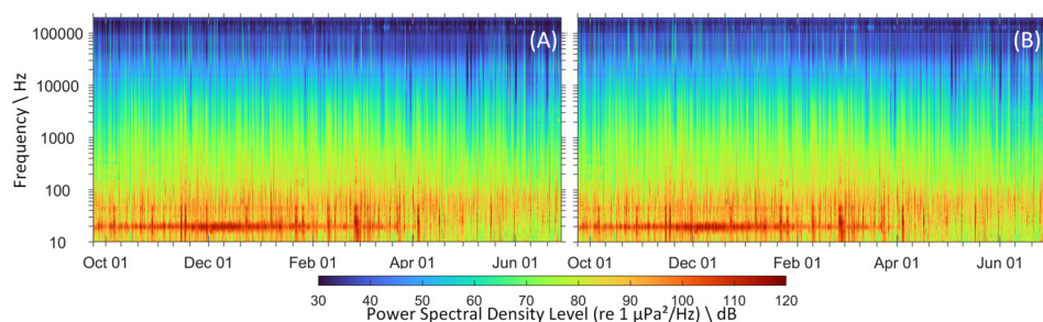
Fig. 1. Long-term spectral average for the Emerald Basin data from (A) millidecade, 1-min, power spectral density data, and (B) 1 Hz, 1-min, power spectral density data. The energy around 20 Hz from October to April is from fin whale choruses.
