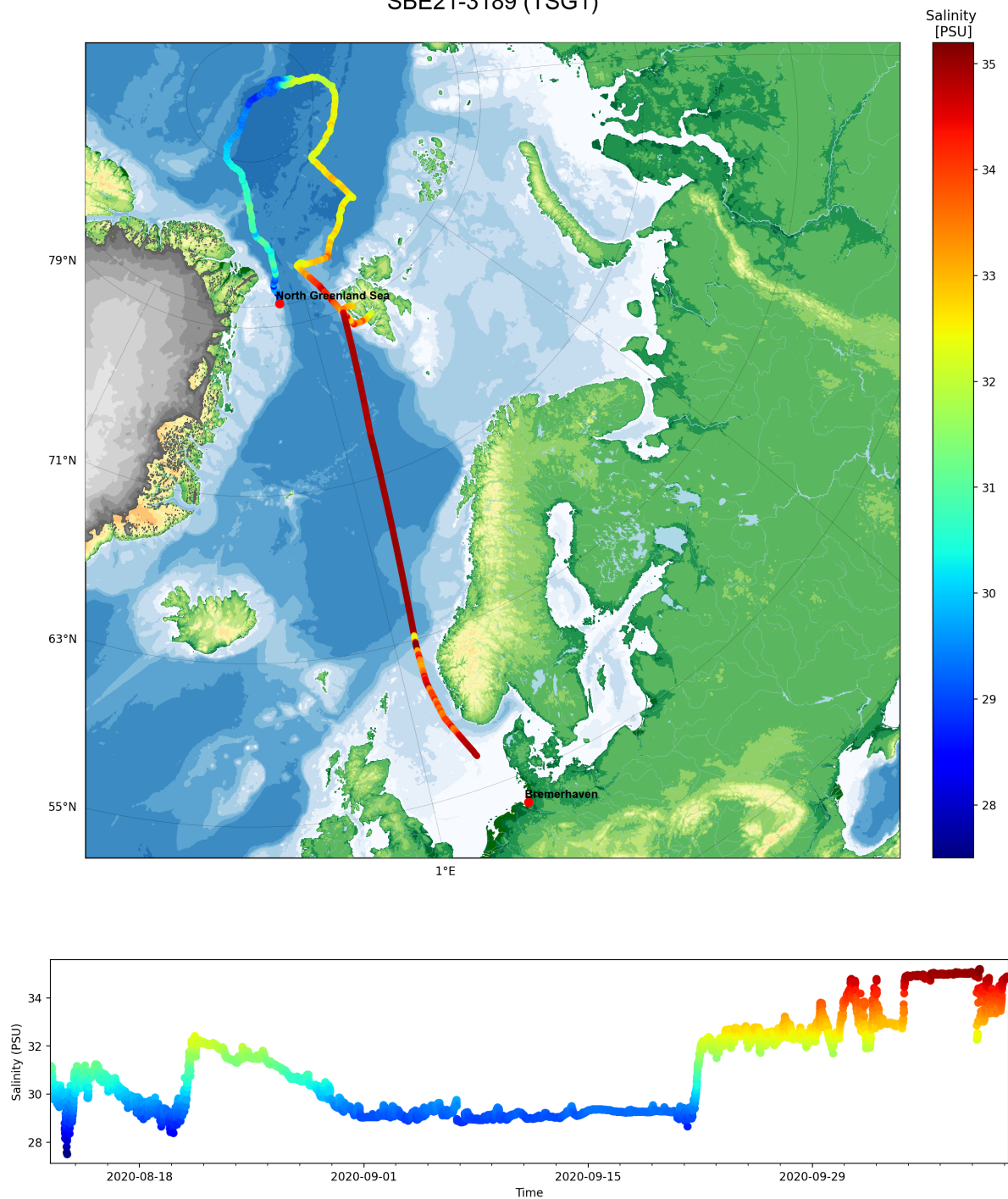
Salinity data from Polarstern cruise PS122_5 SBE21-3189 (TSG1)
