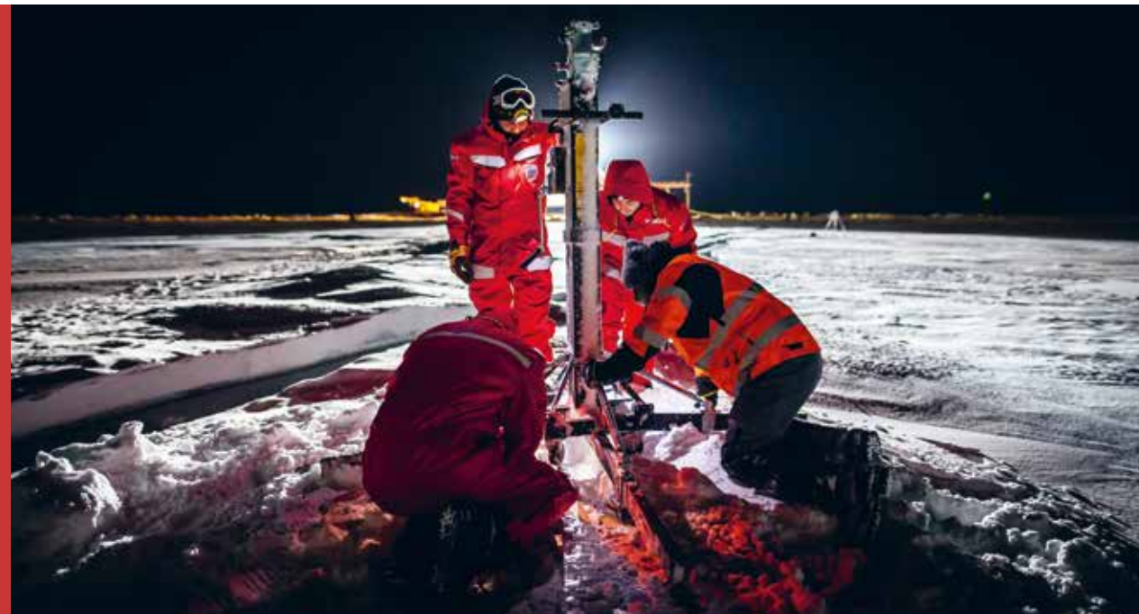
Relocating the equipment: While one of the instruments was being dismantled, the lead in the ice was less than two metres away. The instruments are mounted on sledges, which means moving them across the ice is strenuous but not impossible.
