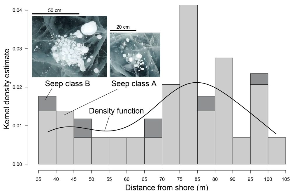
Figure 3. Distribution of CH 4 seeps of class A and B (Walter Anthony and Anthony, 2013) in Goltsovoye Lake (LK) perpendicular to the northwestern shore in a snow-cleared area of 70 × 1.4 m. Bars represent the frequency of seeps A and B given as probability. The black line shows the kernel density function (Gaussian kernel performed on distances to shore; width is 34 data points).
