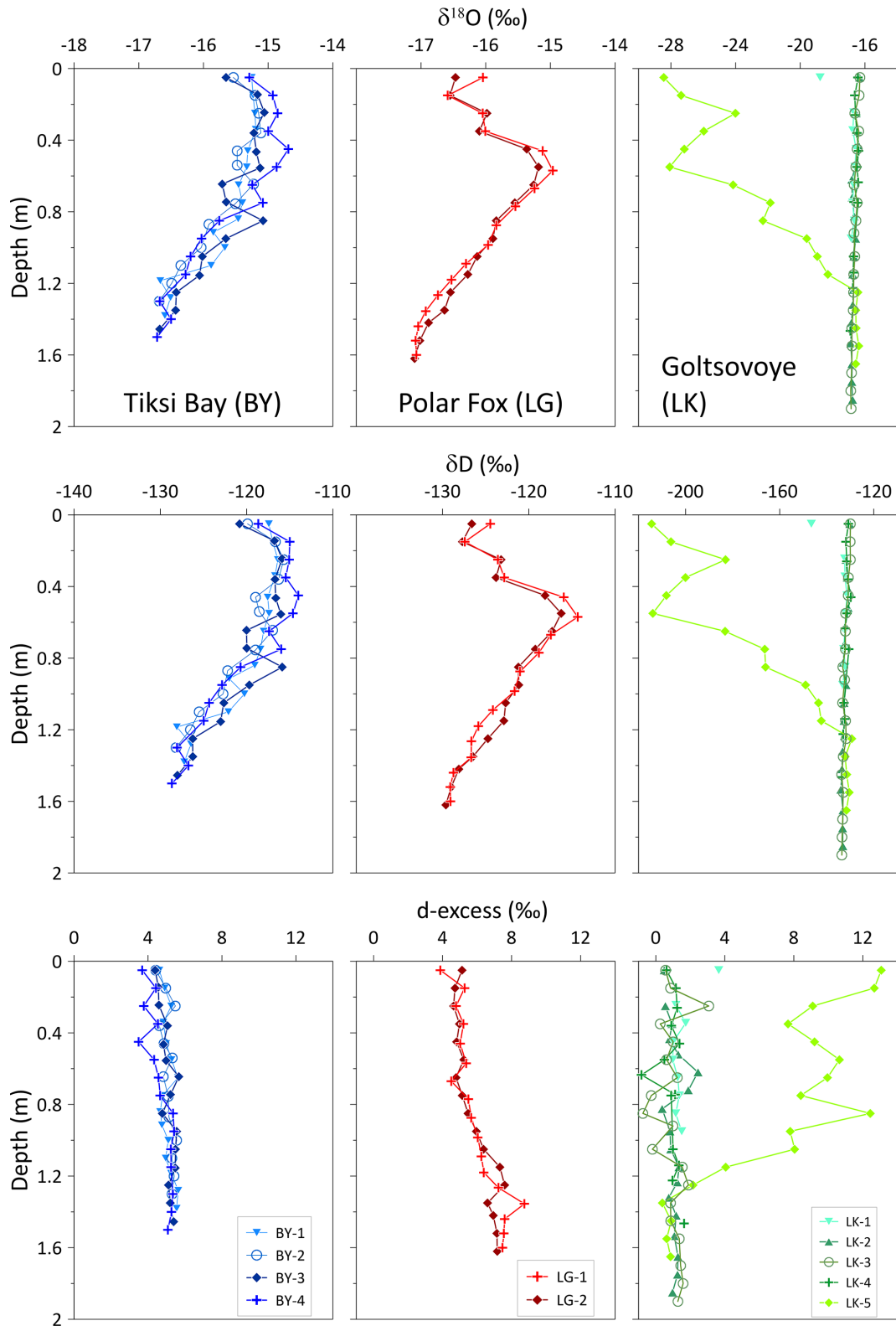
Figure 5. Vertical distribution of the stable water isotopic compositions ( \delta^{18}\text{O} , \delta\text{D} and d-excess) in ice cores with depth. Note that the isotopic composition scales for Goltsovoye Lake (LK, at right) differ from the other two sites to accommodate the values observed in core LK-5.
