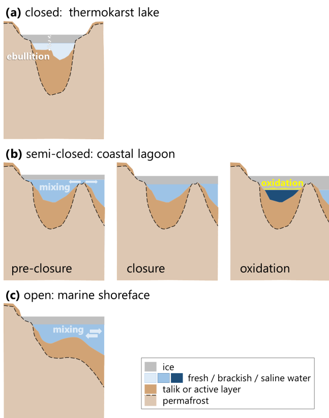
Figure 7. Schematics of geomorphological differences between the three aquatic systems under investigation: (a) the closed system represents a typical thermokarst lake, such as LK, with a closed talik and a complete winter ice cover over fresh water; (b) the semi-closed system is a brackish to highly saline water body (LG), whose ice cover separates it from the marine system at some point during the winter and for which continued ice growth can lead to hypersalinity; and (c) the open system (BY), where ice cover growth does not prevent mixing with marine and/or fluvial waters beneath the ice.
