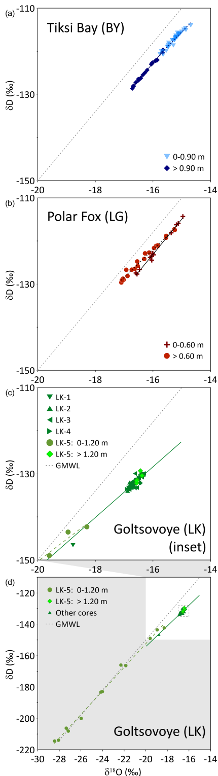
Figure 8. Isotope composition and linear regressions for Tiksi Bay (BY, a ), Polar Fox Lagoon (LG, b ) and Goltsovoye Lake (LK, c , d ) ice cores. For comparison, the global meteoric water line (GMWL, \delta D = 8 \times \delta^{18}O + 10 ; Craig, 1961, grey dotted line) is shown. The limits of the axes of the inset graph ( d ) differ from those above.
