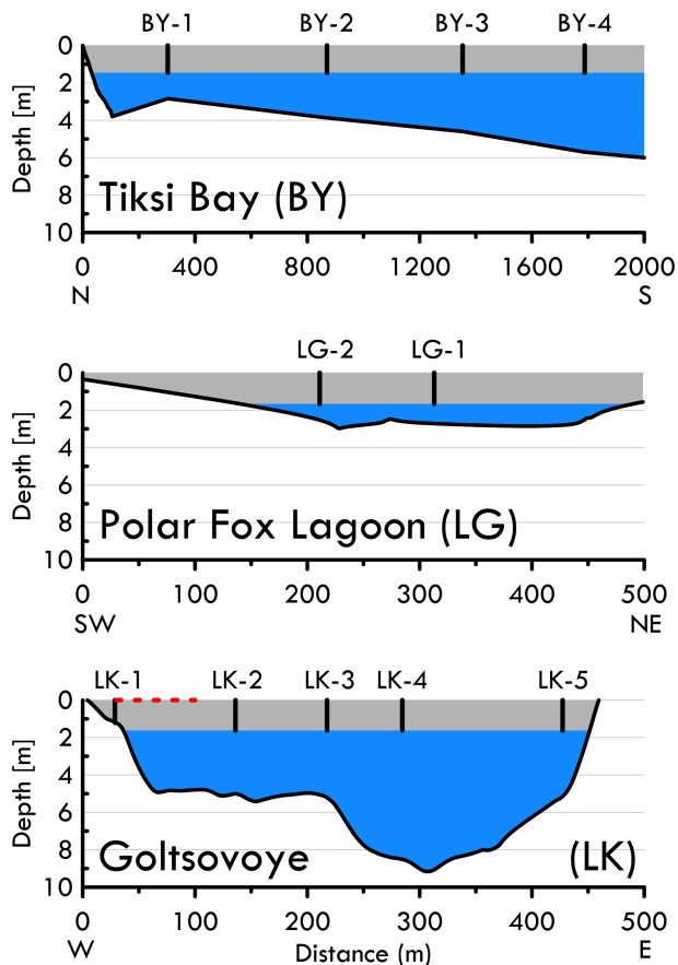
Figure 2. Cross sections of the bathymetry of the Tiksi Bay (BY) profile (N to S), Polar Fox Lagoon (LG) from southwest to northeast and Goltsovoye Lake (LK) along the coring transect (W to E). Positions of the ice cores are indicated as numbered vertical lines in the ice layer (grey shading shows mean water body ice thickness), and the water column below the ice is indicated in blue. The position of the bubble transect at Goltsovoye Lake is represented with a dashed red line.
