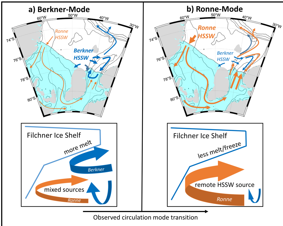
Figure 11. Schematic representation of the regional circulation and its impact on the northern FIS edge during (a) Berkner- and (b) Ronne-modes. The top panels indicate a map view of the circulation, while the bottom panels represent a meridional cross-section of the FIS edge. The Berkner-mode is dominated by Berkner-HSSW in Filchner Trough, associated with enhanced melt rates at the northern base of FIS. The Ronne-mode features an enhanced circulation in the cavity with an enhanced outflow of ISW from underneath FIS. Basal melting is reduced at northern FIS, but is enhanced inside the cavity. Circulation arrows are based on insights gained from the 2018 CTD survey and drill hole moorings (H2021) as well as from earlier literature-based findings.
