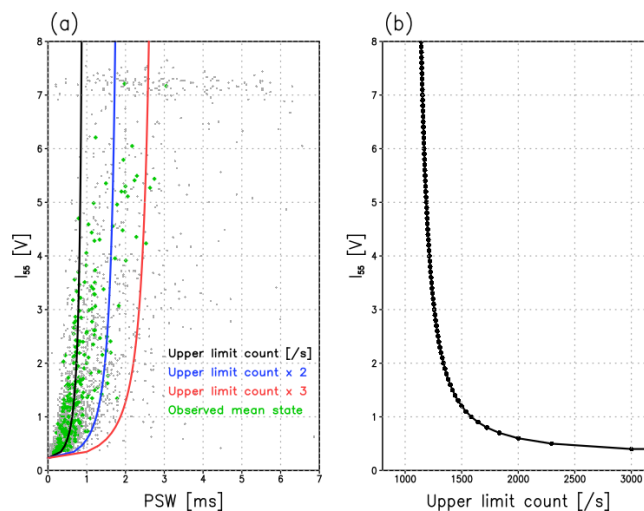
Figure 12. (a) Estimated relationship between PSW and I_{55} based on the upper limit of countable particle number (a black line) in the case of \text{PSW}_e = 1.0 . Blue and red lines indicate the doubled and tripled situations from the normal upper limit count. Gray dots are the same plot in Fig. 6a. Green dots indicate the mean state for each second after applying the cutoff value of PSW ( \text{PSW}_c ). (b) Upper limit of countable particle number as a function of I_{55} in case of \text{PSW}_e = 1.0 .
