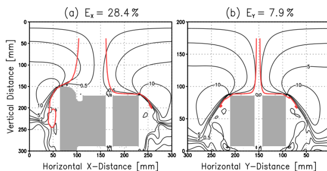
Figure 8. Innermost trajectories against the CPS housing (indicated by red lines) for the (a) horizontal x direction ( u component) and (b) horizontal y direction ( v component). E_x and E_y indicate the estimated collection efficiency (%) for each component. Black lines are absolute constants of hyperbolic flow.
