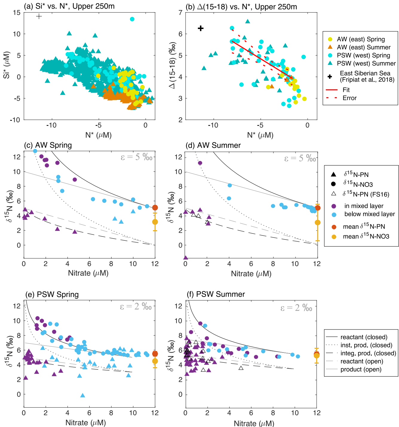
Figure 5. (a) N^* plotted against Si^* ( \mu\text{M} ) and (b) N^* plotted against \Delta(15-18) (‰). (c–f) Uptake fractionation of \delta^{15}\text{N}\text{-NO}_3 (circles) and \delta^{15}\text{N}\text{-PN} (triangles) from JR17005 and PS100. (c) Samples from Atlantic Water during May–June 2018 (JR17005). (d) Samples from Atlantic Water during July–August 2016 (PS100). (e) Samples from Polar Surface Water during May–June 2018 (JR17005). (f) Samples from Polar Surface Water during July–August 2016 (PS100). Additional black open triangles in panels (d) and (f) are \delta^{15}\text{N}\text{-PN} values in the mixed layer in August–September 2016 from cruise FS16. Black and gray lines describe the fractionation trends for an isotopic effect of 5‰ (AW) and 2‰ (PSW).
