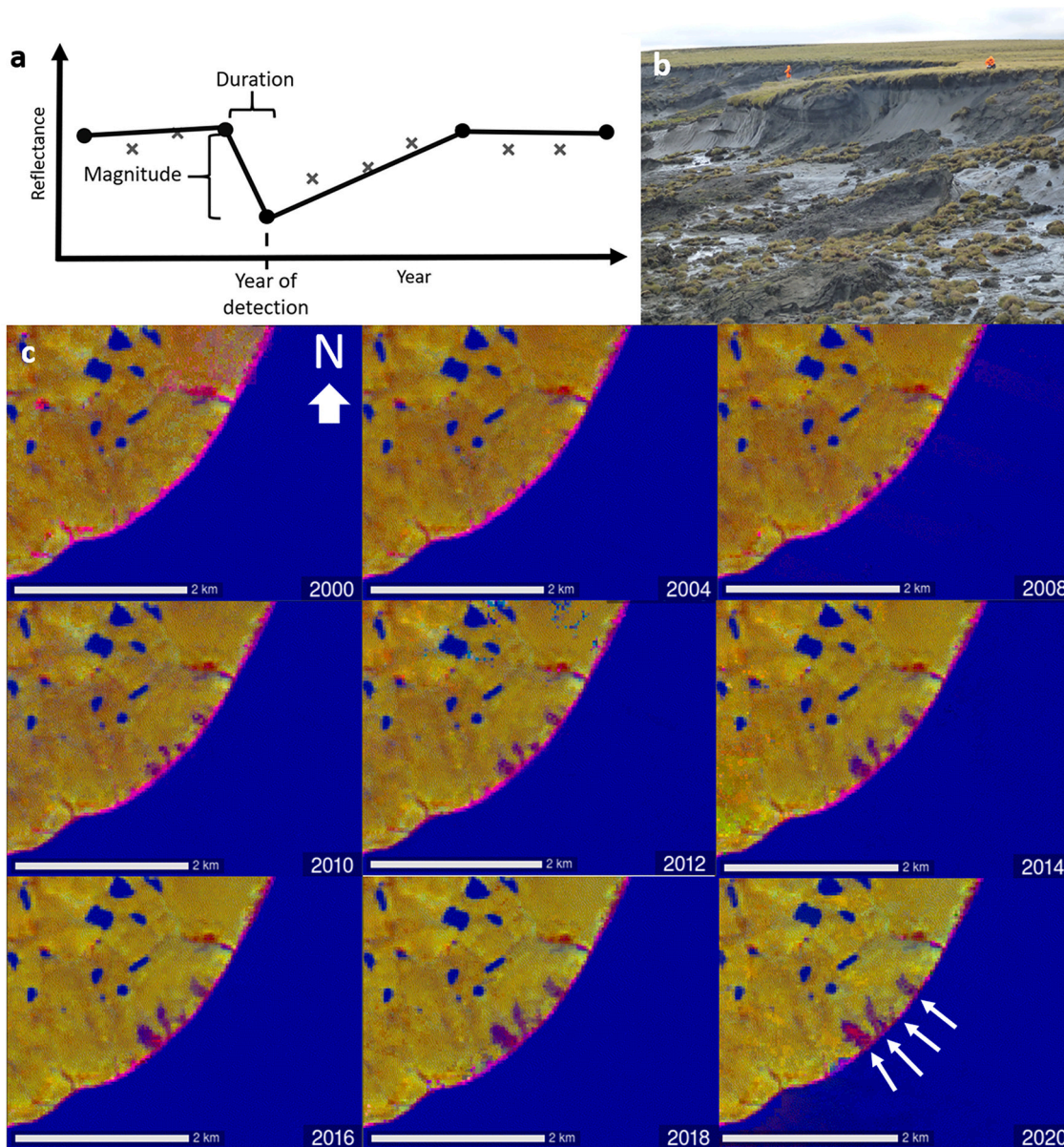
Fig. 3. Retrogressive thaw slump detection by LandTrendr. a. LandTrendr temporal segmentation schematic, indicating the year of detected disturbance from change in spectral magnitude and disturbance duration. b. Picture of coastal thaw slumping at Bykovsky Peninsula (129.2° E, 71.5° N) in 2014 (G. Grosse). Note persons for scale. c. Thumbnails indicating the development of RTS (white arrows in 2020) at the coast of Chukotka (172.2° W, 64.6° N) 2000–2020. Illustration based on a TCB/TCG/TCW visualisation in the LT-GEE Time Series Animator App (Justin, 2020).
