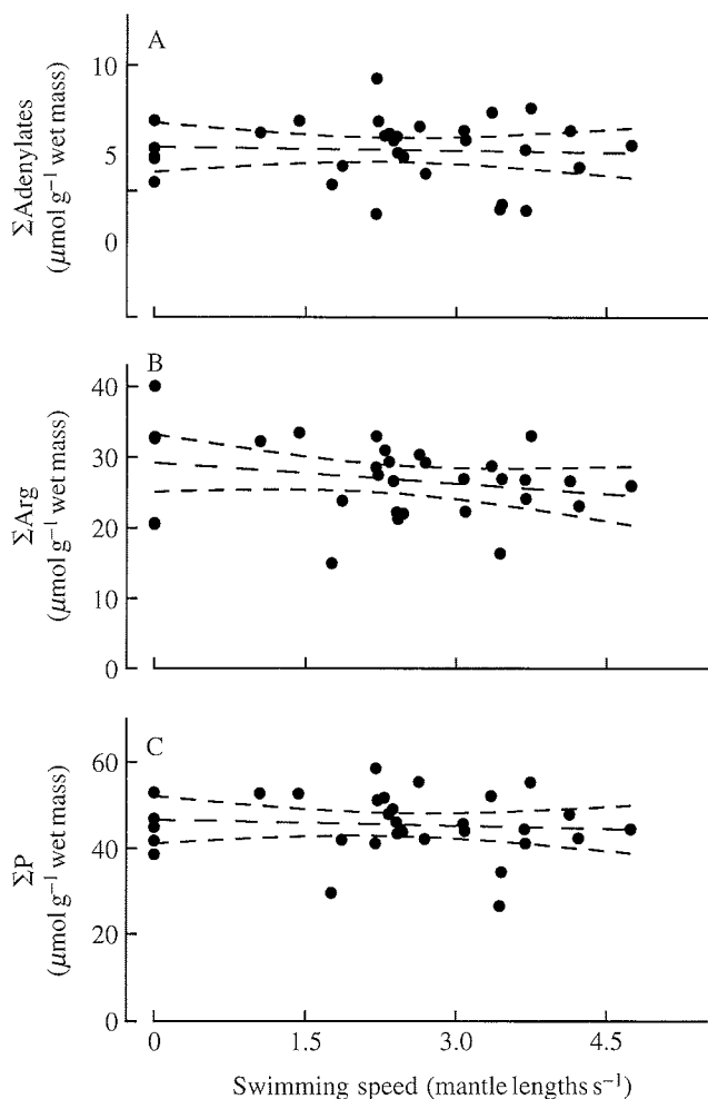
Fig. 8. Summed concentrations of (A) all adenylates ( \Sigma\text{Adenylylates} = [\text{ATP}] + [\text{ADP}] + [\text{AMP}] , r=0.05 , linear regression), (B) L-arginine metabolites ( \Sigma\text{Arg} = [\text{phospho-L-arginine}] + [\text{L-arginine}] + [\text{octopine}] , r=0.24 , linear regression) and (C) inorganic and organic phosphates ( \Sigma\text{P} = [\text{phospho-L-arginine}] + 3[\text{ATP}] + 2[\text{ADP}] + [\text{AMP}] + [\text{glucose 6-phosphate}] + [\alpha\text{-glycerophosphate}] + [\text{P}_i] ; r=0.09 , linear regression) in the mantle musculature of the squid Lolliguncula brevis at different swimming speeds.
