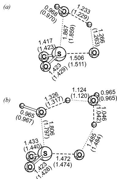
Figure 1. B3LYP/3df and MP2/2df (in parentheses) optimized structural parameters of transition states of \text{SO}_3 hydration: (a) TS1a; (b) TS1b. Hereafter, the dashed line marks a formed bond; the dotted line a breaking bond.
