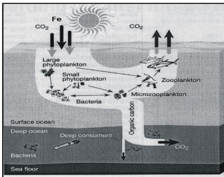
Fig. 1. The complex phytoplankton-based food web.
