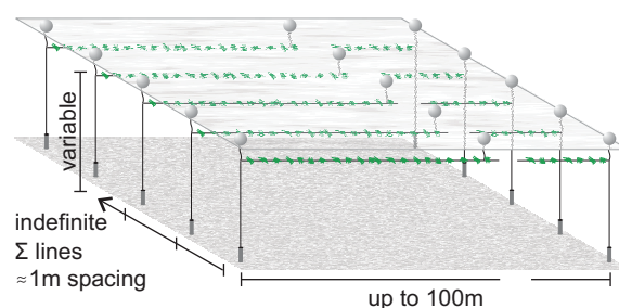
Figure 11. Schematic drawing of the floating long-line method
