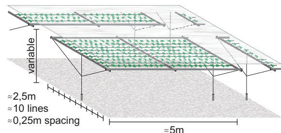
Figure 10. Schematic drawing of the floating raft method
