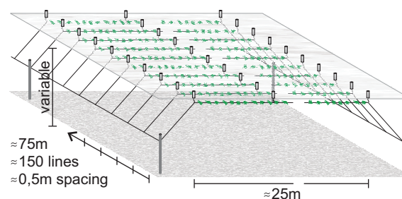
Figure 3. Commonly used farming method in Puntondo, cultivation lines are kept afloat by empty water bottles
