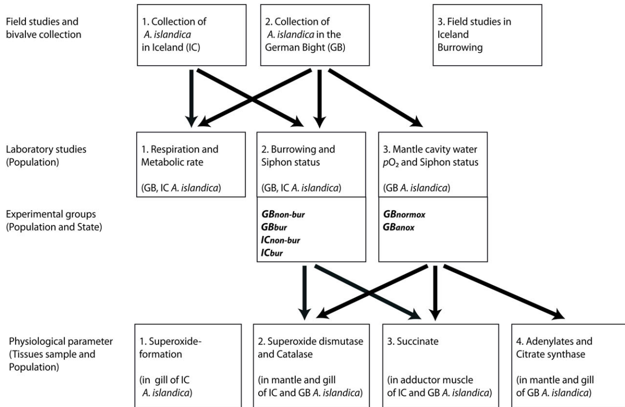
Fig. 1. Flow diagram of fieldwork, laboratory experiments and measurements of the physiological parameters in Arctica islandica from Iceland (IC) and the German Bight (GB). Experimental bivalves were either non-burrowed ( GB non-bur , IC non-bur ) or burrowed for 3.5 days ( GB bur , IC bur ), and in a second experimental approach of changing the partial pressure of oxygen ( P_{O_2} ) in the mantle cavity water ( GB normox ) or for \geq 24 h of 0% O_2 in the mantle cavity water ( GB anox ), N=9-11 .
