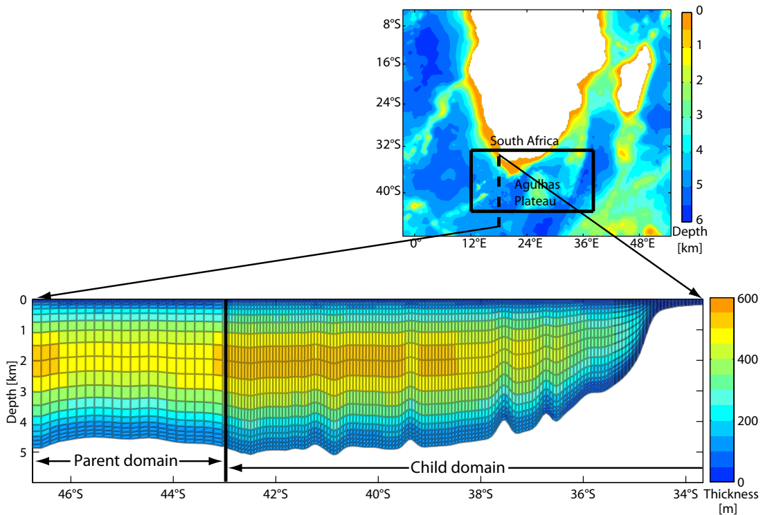
Figure 3.5.: Top: Map of the whole model domain and the nested child model domain (black frame). Bottom: Vertical structure of parent model and child model along 18^\circ\text{E} .
