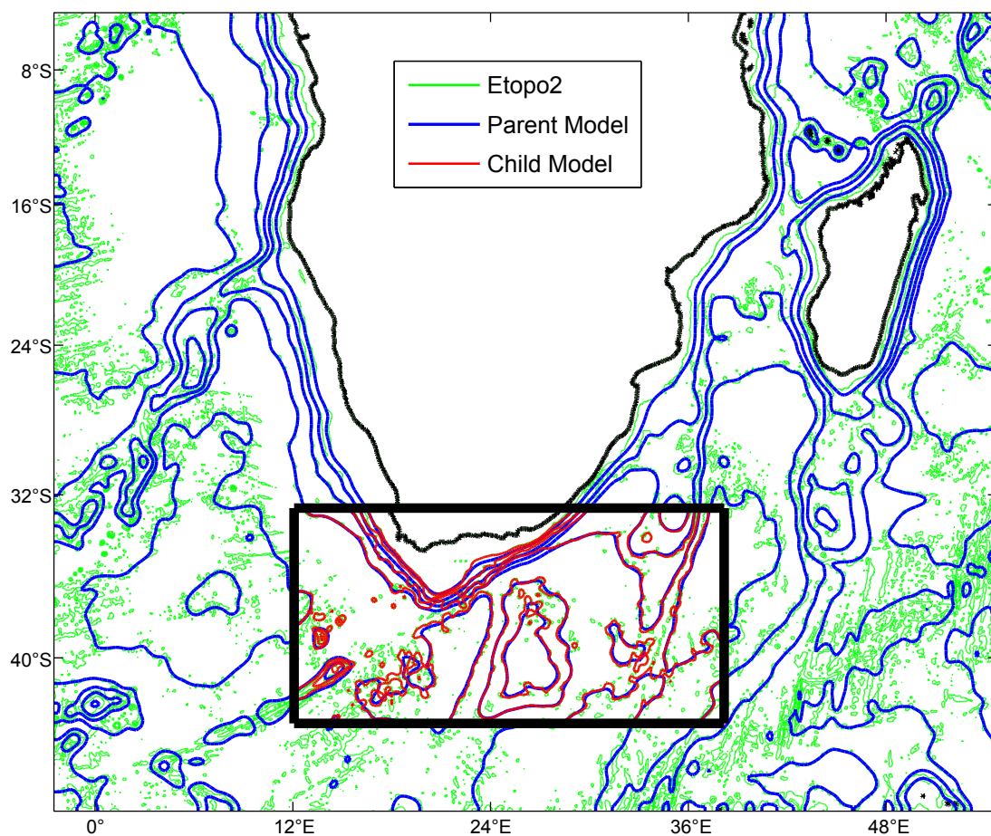
Figure 3.6.: Comparisons of isobaths from the raw Etopo2 data set with those from models after smoothing. The interval between the isobaths is 1000 m.
