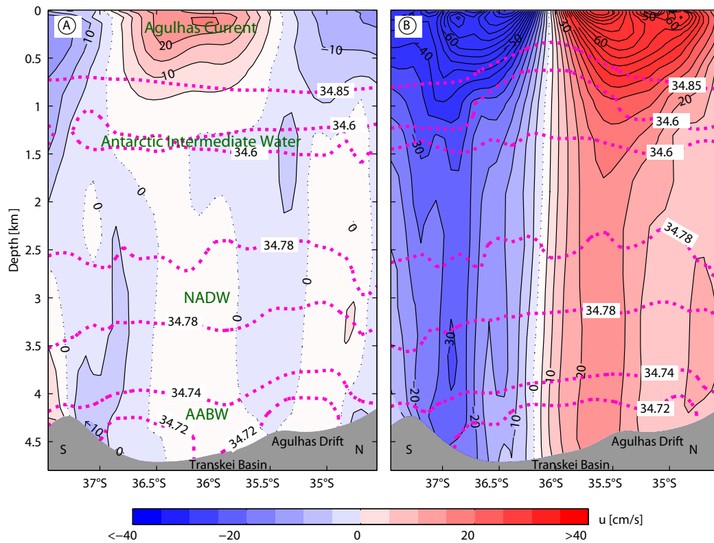
Figure 5.5.: Velocity section along 29.25^\circ\text{E} (a) for a ‘no eddy’ event on the 20th March, and (b) for an eddy event on the 12th April in the 4th model year. Location of these sections is depicted in Figure 5.1. Velocities are positive (red) in the eastward direction. In both plots, the black dotted lines denote zero velocity, and the magenta dashed lines mark the salinity surfaces indicating the different water masses.
