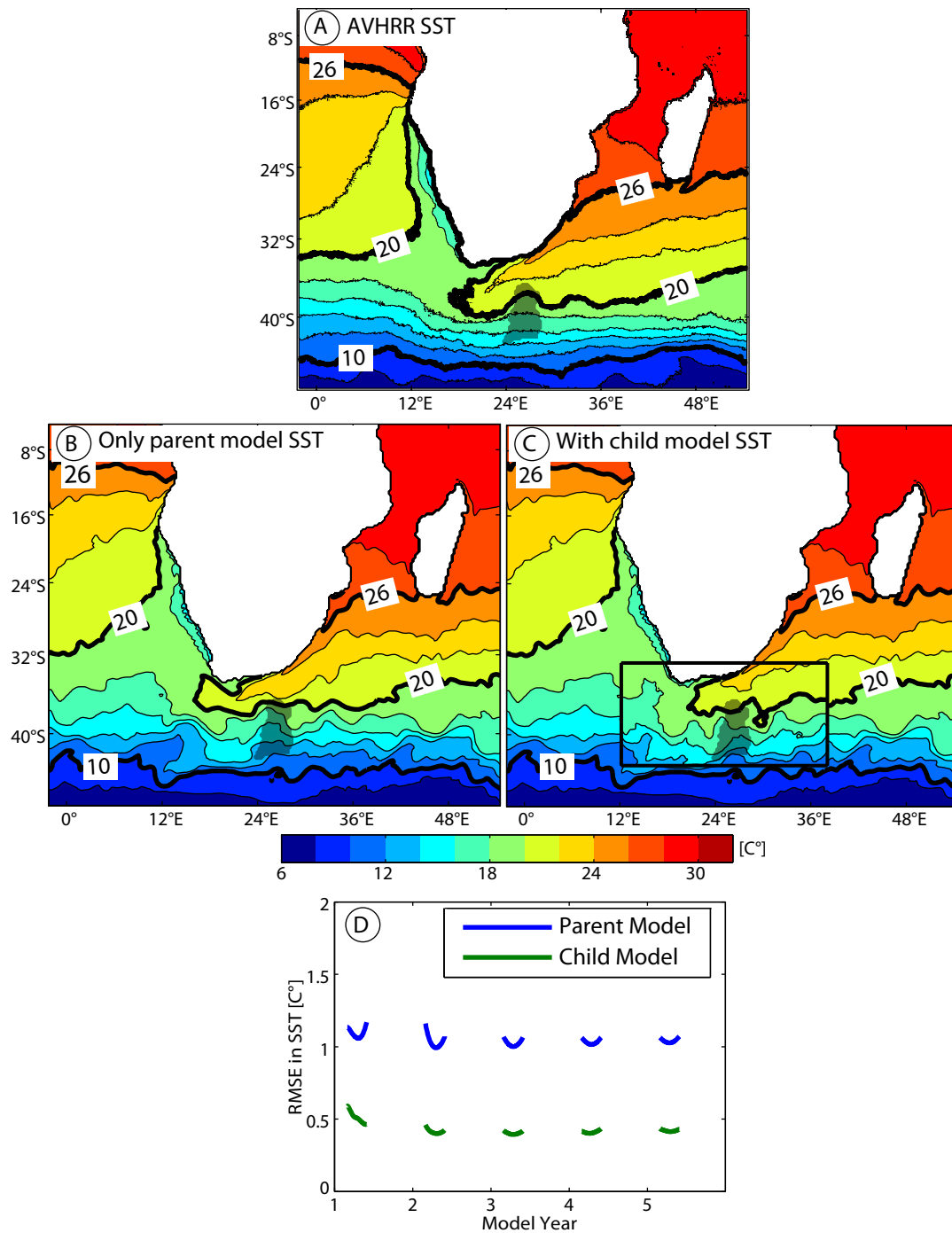
Figure 4.2.: Observations/model comparisons of averaged SST (a–c) and time evolution of RMSE in SST(d). The SST satellite image is derived from the AVHRR Pathfinder Version 5.0 data. In Figures a–c, grey shadow indicates the position of the Agulhas Plateau.
