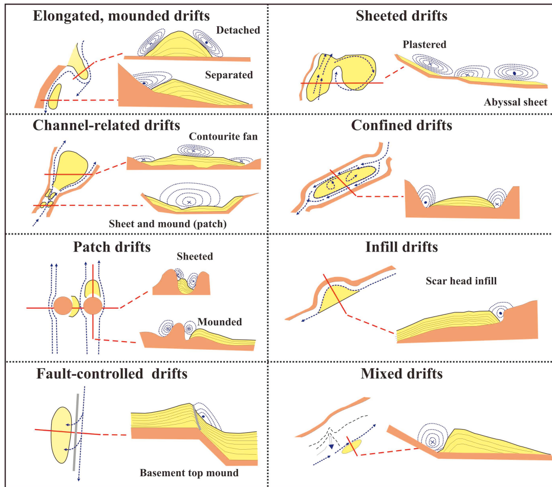
Figure 2.1.: Up and lateral view of sediment drift types and inferred bottom current paths (after Rebesco and Stow , 2001; Rebesco , 2005; Rebesco et al. , 2008). The large-scale geometry of contourites is represented by the seismic expression. Red lines on up views indicate the location of the lateral view. The axis of bottom-currents is marked as black dashed lines in up view and as black dashed arches in lateral view.
