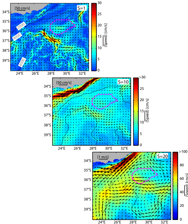
Figure 5.2.: The averaged velocity fields in the layers s_1 , s_{10} and s_{20} from the 3rd to 5th model years. The positions of these layers are marked in Figure 5.1. 1 vector is portrayed every 4 vectors. The grey lines mark the isobaths. Computed boundary of the Agulhas Drift ( Schlüter and Uenzelmann-Neben, 2008 ) is marked as in Figure 5.1.
