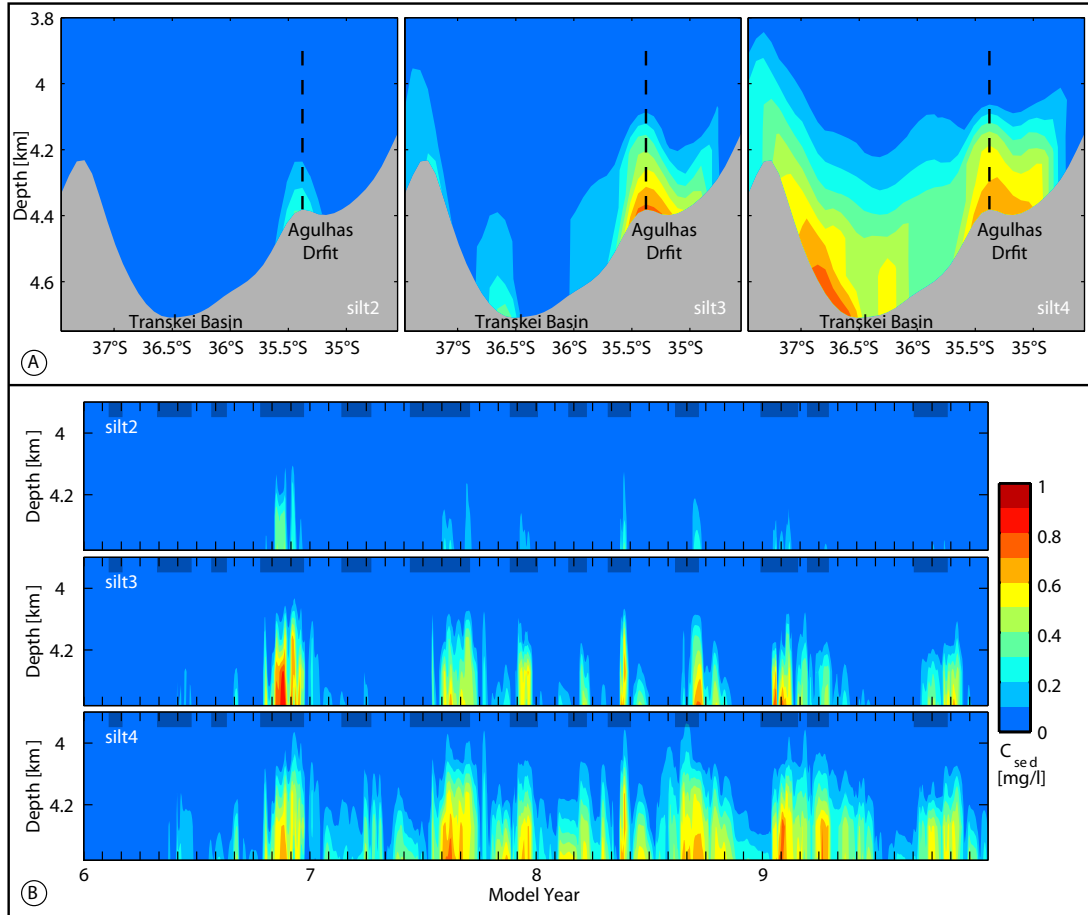
Figure 6.11.: Vertical sediment concentration sections along 29.25^{\circ}\text{E} (P1 in Figure 6.1) on 28 May in the 7th model year. The black dashed lines label the section position of Figure 6.11b. (b) Hovmöller diagrams for the vertical concentration section at 29.25^{\circ}\text{E} , 35.38^{\circ}\text{S} (intersection of two sections P1 and P2 in Figure 6.1). The thick grey transparent lines on the upper axis mark the eddy periods.
