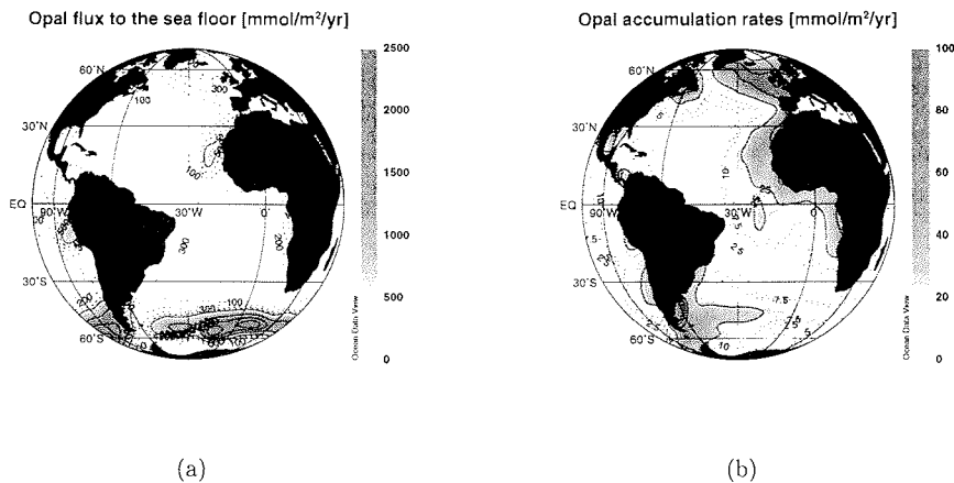
Figure 5.3: Opal flux to the sea floor (a) and accumulation rates (b) from experiment HANT
