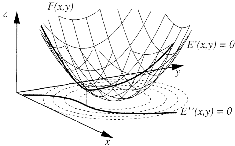
Figure 2.2: Example functions for constrained optimization
