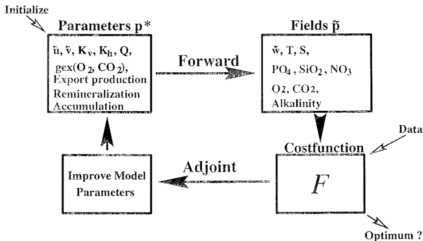
Figure 2.1: Schematic sketch of the adjoint model
