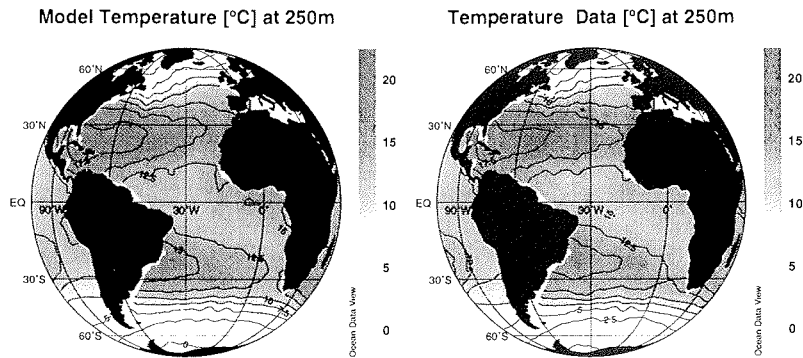
Figure 3.4: Model temperatures (left) and data (right)
