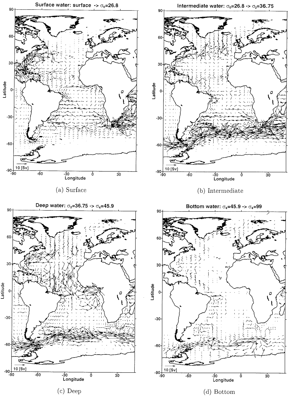
Figure 3.2: Horizontal current field from experiment REF
