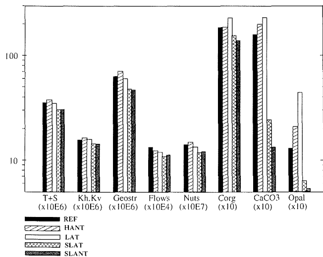
Figure 3.1: Absolute values of terms of costfunction after termination of the optimization. For explanation, see text
