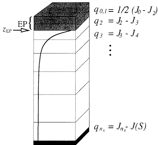
Figure 2.6: Water column with sources and sinks
