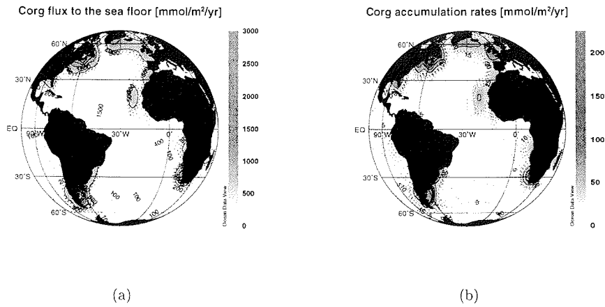
Figure 5.1: C_{org} flux to the sea floor (a) and accumulation rates (b) from experiment HANT
