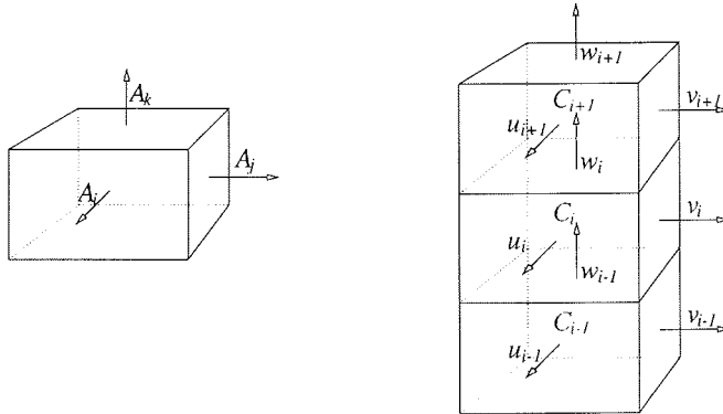
Figure 2.5: Definitions within the model grid
