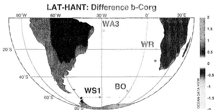
Figure 4.7: Differences of remineralization scale lengths between experiments HANT and LAT.
