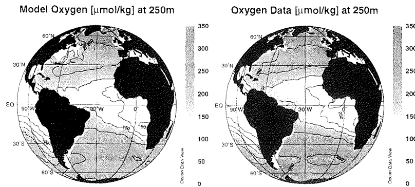
Figure 3.7: Model oxygen (left) and data (right)
