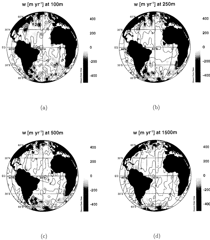
Figure 3.3: Vertical velocities in the Atlantic from experiment REF
