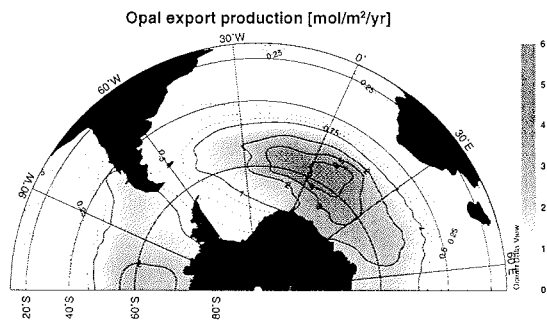
Figure 6.1: Opal export production
