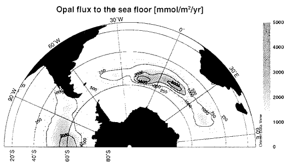
Figure 6.2: Opal flux to the sea floor
