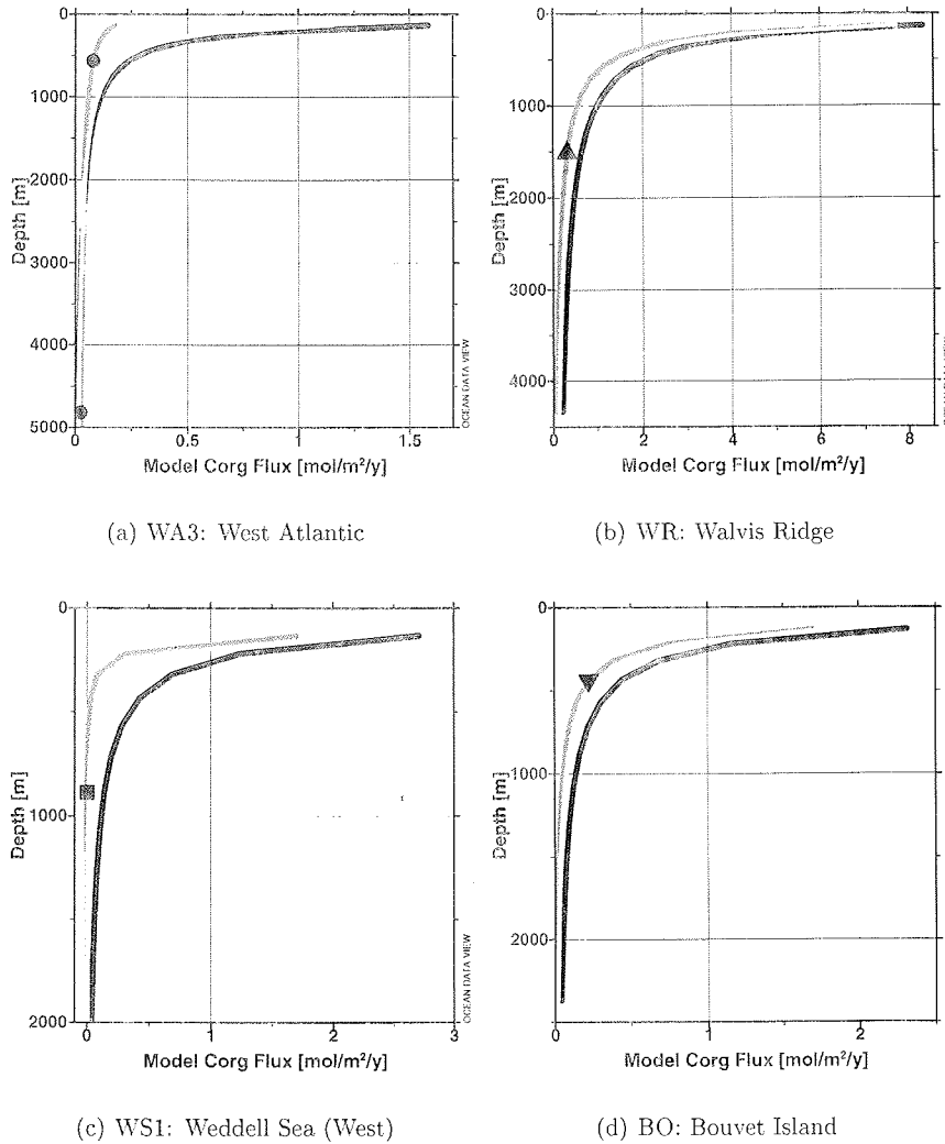
Figure 4.5: C_{org} model fluxes from experiment HANT (black) and LAT (grey). Sediment trap data are displayed as filled marks.
