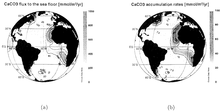
Figure 5.2: CaCO_3 flux to the sea floor (a) and accumulation rates (b) from experiment HANT
