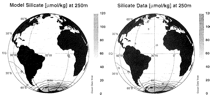
Figure 3.8: Model silicate (left) and data (right)
