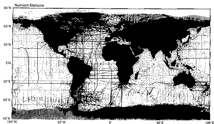
Figure 2.3: Global distribution of stations with nutrient data
