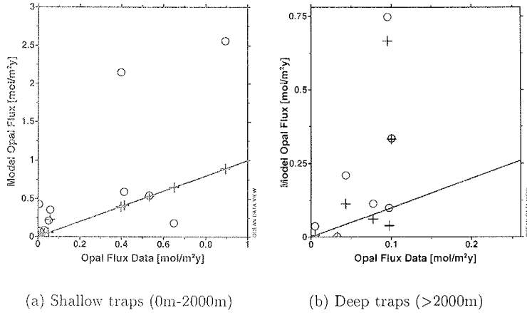
Figure 4.10: Opal model fluxes vs. sediment trap data for the unconstrained model HANT (circles) and the model constrained with sediment trap data LAT (crosses). Solid line: 1:1 relation
