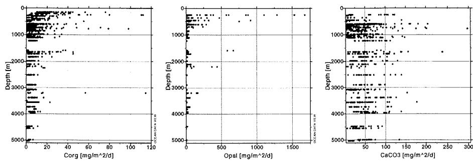
Figure 4.3: Fluxes of C_{org} , Opal and CaCO_3 vs. depth
