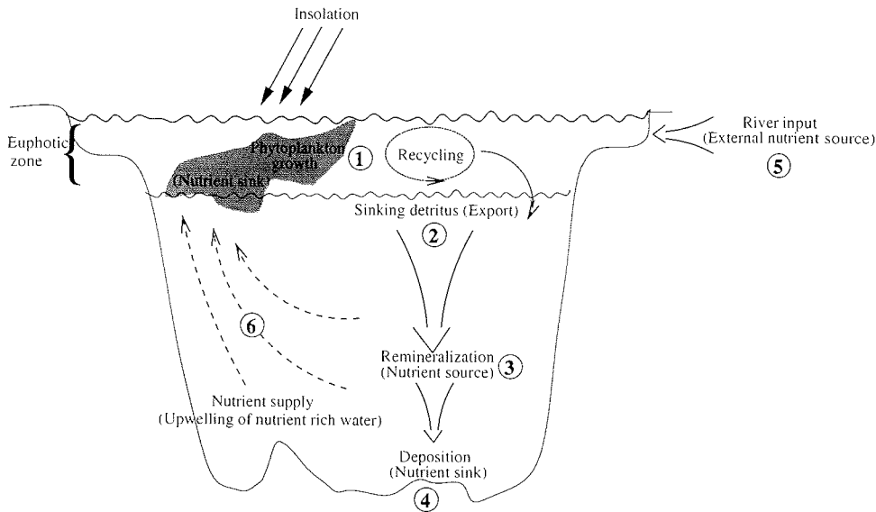
Figure 1.2: Schematic diagram of the biological pump in the ocean
