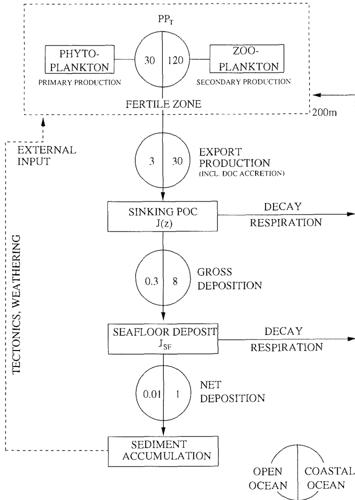
Figure 1.3: Fluxes of particular organic carbon in the world ocean from Berger et al. (1989b). Numbers denote fluxes in units [\frac{gC}{m^2y}]
