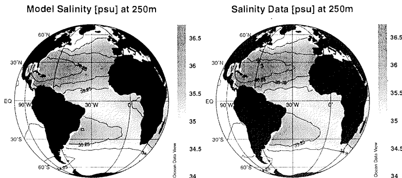
Figure 3.5: Model salinities (left) and data (right)
