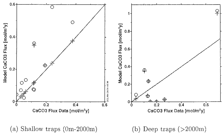
Figure 4.9: CaCO_3 model fluxes vs. sediment trap data for the unconstrained model HANT (circles) and the model constrained with sediment trap data LAT (crosses). Solid line: 1:1 relation
