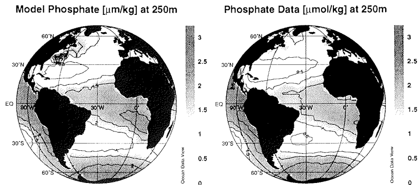
Figure 3.6: Model phosphate (left) and data (right)
