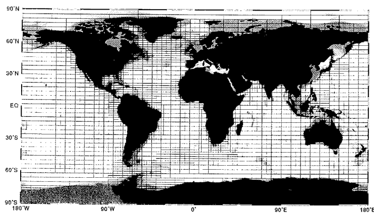
Figure 2.4: Model grid
