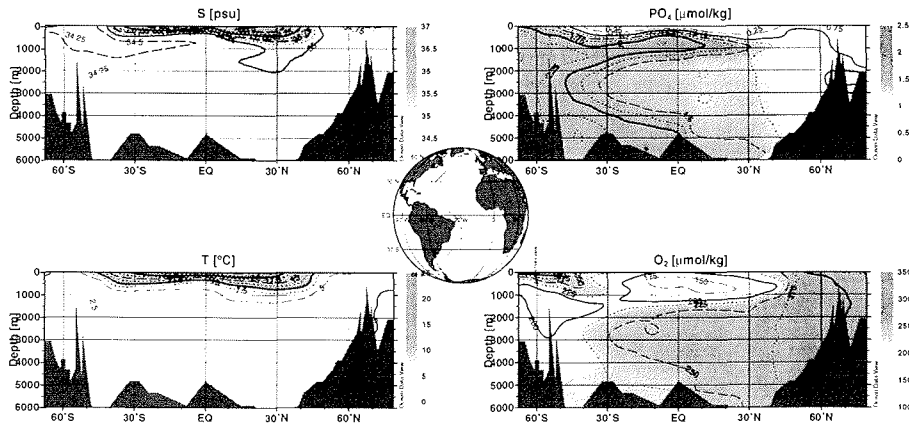
Figure 1.1: Temperature, salinity, phosphate, and oxygen concentrations along the west Atlantic GEOSECS (Geochemical Ocean Sections Study) section (Bainbridge, 1980)
