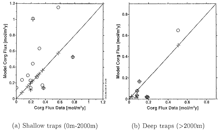
Figure 4.8: C_{org} model fluxes vs. sediment trap data for the unconstrained model HANT (circles) and the model constrained with sediment trap data LAT (crosses). Solid line: 1:1 relation
