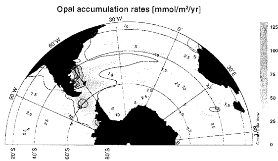
Figure 6.3: Opal accumulation rates
