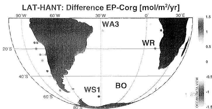
Figure 4.6: Differences of export production rates between experiments HANT and LAT.
