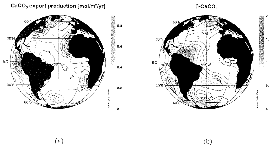
Figure 3.11: CaCO_3 export production (a) and remineralization scale length \beta (b)
