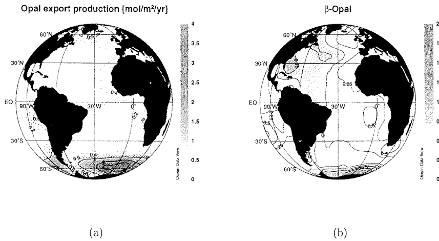
Figure 3.12: Opal export production (a) and remineralization scale length \beta (b)
