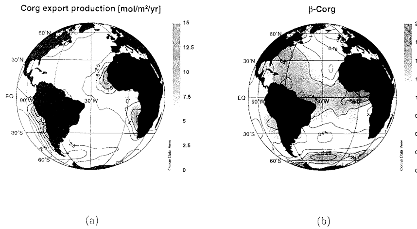
Figure 3.10: C_{org} export production (a) and remineralization scale length \beta (b)
