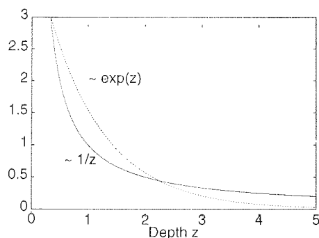
Figure 2.7: Functions describing particle fluxes decreasing with depth exponentially and \propto 1/z , respectively (arb. units)
