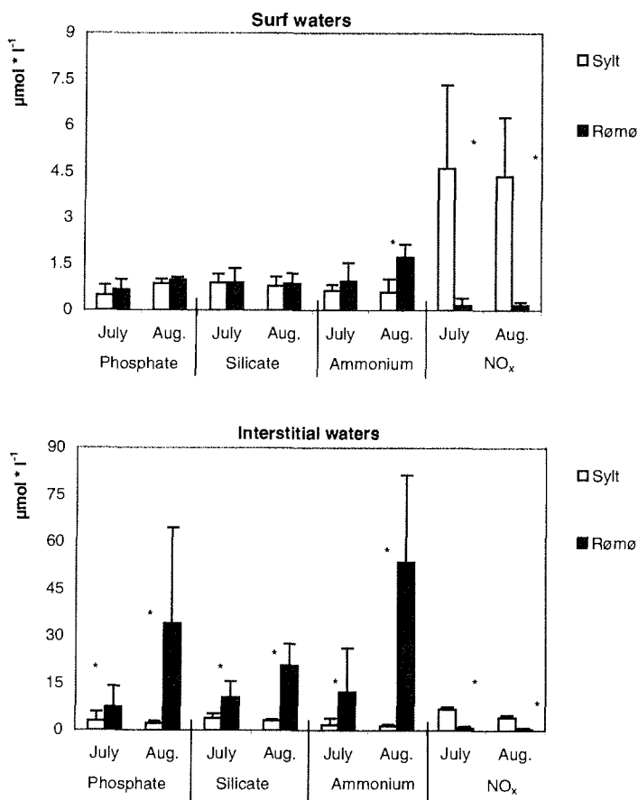
Fig. 5 Inorganic nutrient concentrations in surf and interstitial waters at Sylt in contrast to Rømø in July and August (Aug.) 1999. Arithmetic means with standard deviations calculated over replicates per sampling survey (July: surf water n = 15 , interstitial water n = 20 ; August: both n = 10 ). \text{NO}_x = nitrite plus nitrate. * = significant differences between shores within each sampling occasion; all U-Test, p < 0.025 , df = 1 . Note the difference in scale between surf and interstitial water.
