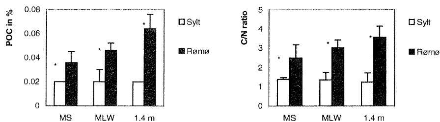
Fig. 4 Particulate organic carbon (POC) and C/N ratio of sediment on the Sylt and Rømø shore in August 1999. Arithmetic means with standard deviations calculated over 8 replicates per position. MS = mid shore; MLW = mean low water; 1.4 m depth line. * = significant differences between shores; all U-Test, p < 0.01 , df = 1 .
