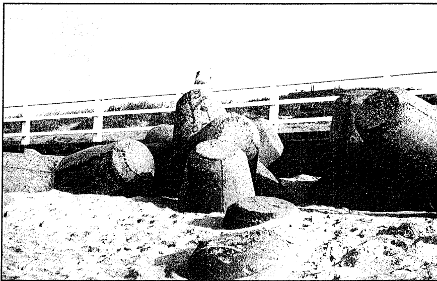
Fig. 8 Sea wall associated with tetrapods on the exposed shore on the island of Sylt (Germany) in the North Sea.
