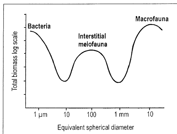
Fig. 5 Size spectrum of benthic biota on sandy beaches, based on Schwinghammer (1981) and Warwick (1984).
