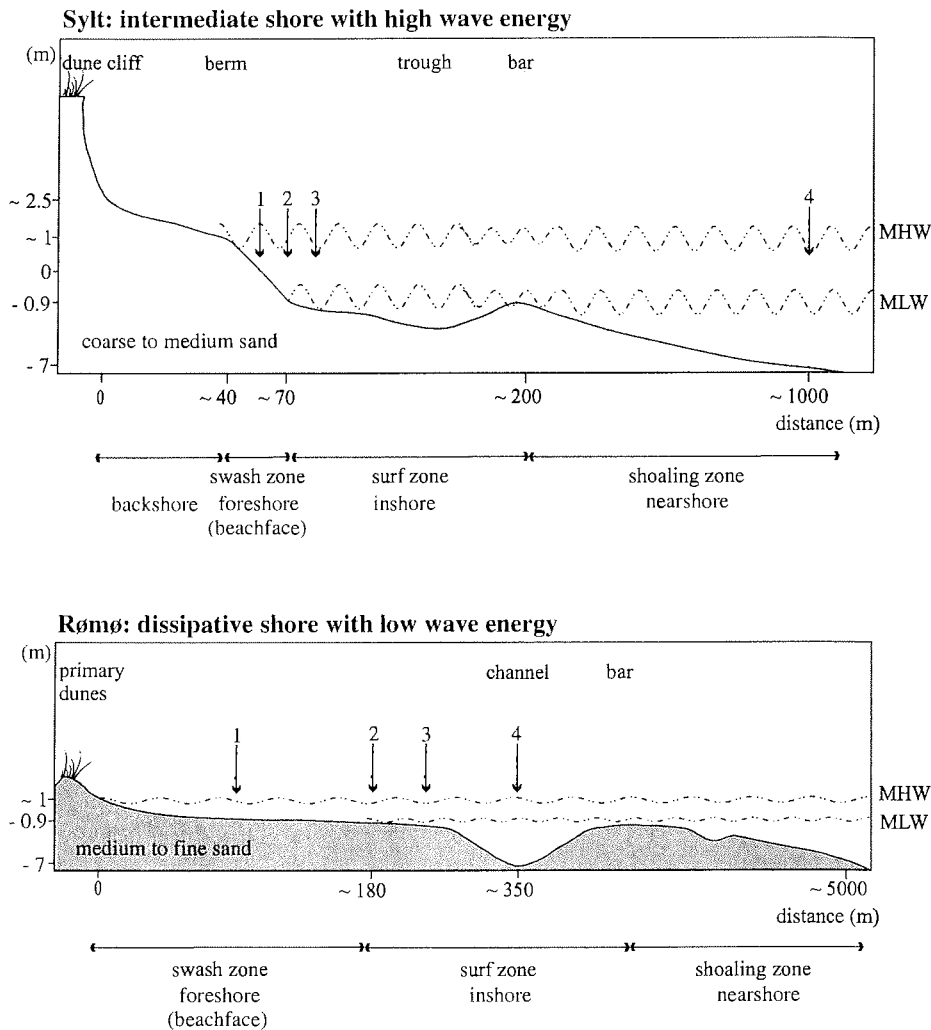
Fig. 2 Schematic illustration of profiles across the Sylt and Rømø shore including sample positions (→ 1-4) and terminology of zones across the shore according to Short (1999). 1 = mid shore (middle between mean high (MHW) and mean low water (MLW)) = 0 m depth, 2 = mean low water (0.9 m depth), 3 = 1.4 m depth, 4 = 7 m depth.
