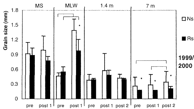
Fig. 3 Grain size at nourished (Ns) and reference site (Rs) across the shore in 1999/2000 presented as arithmetic means with standard deviations of 6 replicates per survey. Pre = pre-survey in April, 1 month before nourishment; post 1 + 2 = post-surveys in October 1999 and April 2000, 3 and 9 months after nourishment. MS = mid shore (0 m depth), MLW = mean low water (0.9 m depth), 1.4 m and 7 m depth line. * = significant differences between sites within surveys. — = significant differences between sampling dates within sites.
