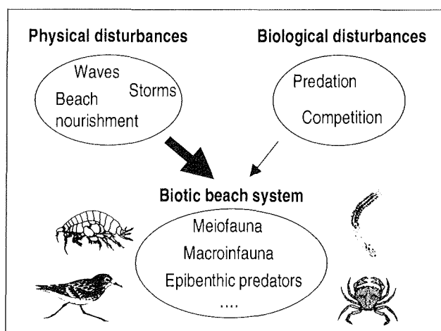
Fig. 4 Schematic model of the influence of physical and biological disturbances to the biotic beach system.
