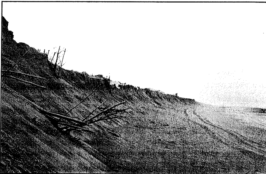
Fig. 4 Erosion of the exposed western side on the island of Sylt (Germany) in the North Sea after a winter storm 1998.
