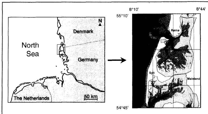
Fig. 1 Study sites (→) on the neighbouring barrier islands of Sylt and Rømø in the eastern North Sea. Average sea water temperature of this cold-temperate region is 4^{\circ}\text{C} in winter and 15^{\circ}\text{C} in summer. Water salinity is the range of 27 to 33 ‰ PSU. Tides are semidiurnal with a mean range of 1.8 m. Shading refers to water depths (> 10 m, > 6 m, > 0 m; intertidal flats).
