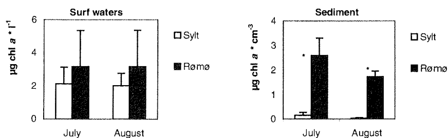
Fig. 3 Chlorophyll a concentrations of surf waters and sediment on the Sylt and Rømø shore in July and August 1999. Arithmetic means with standard deviations of 10 replicates per sampling occasion (with exception of sediment sampling in July; n = 20 ). * = significant differences between shores within each sampling survey; both U-Test, p < 0.001 , df (degree of freedom) = 1.
