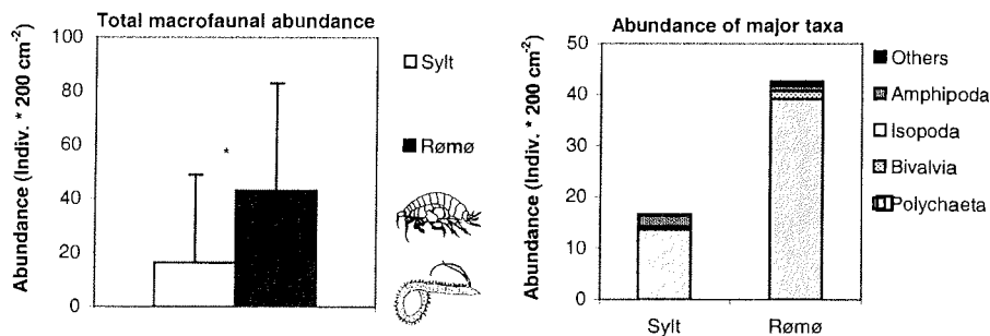
Fig. 5 Total macrofaunal abundance and abundance of major taxa per 200 cm 2 on the Sylt and Rømø shore. Arithmetic means with standard deviations of four transect positions, each six times replicated, and of four sampling surveys (n = 96). Others = decapods, nemerteans, cumaceans and gastropods. * = significant difference between the shores.
