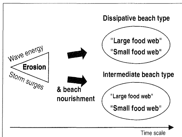
Fig. 5 Increasing erosion on sandy shores followed by an increasing use of beach nourishment to combat the erosion will result in highly dynamic intermediate shores away from equilibrium state. The biotic system of these shores may be characterized by an impoverished "large food web", while meiofauna is abundant, of high evenness between major taxa and of high diversity in interstitial plathelminths and polychaetes.
