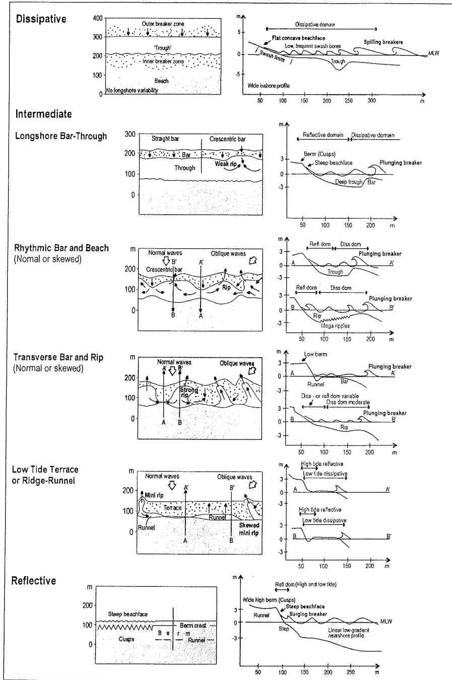
Fig. 3 Top view (left) and side profile (right) of wave-dominated beach types. Simplified from Short (1999). For more details see Short (1999). MLW = Mean low water.
