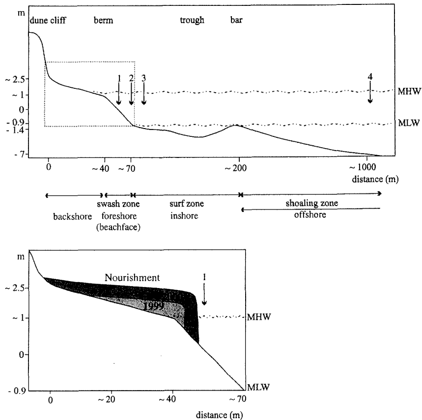
Fig. 2 Schematic profile across the Sylt shore with sampling sites (→ 1-4), and terminology for zones according to Short (1999). In the detail below, the amount of replenished sand and the resulting beach profiles in 1999 and 2000 are indicated. 1 = mid shore (middle between mean high (MHW) and mean low water line (MLW)) = 0 m depth; 2 = mean low water (0.9 m depth); 3 = 1.4 m depth; 4 = 7 m depth.
