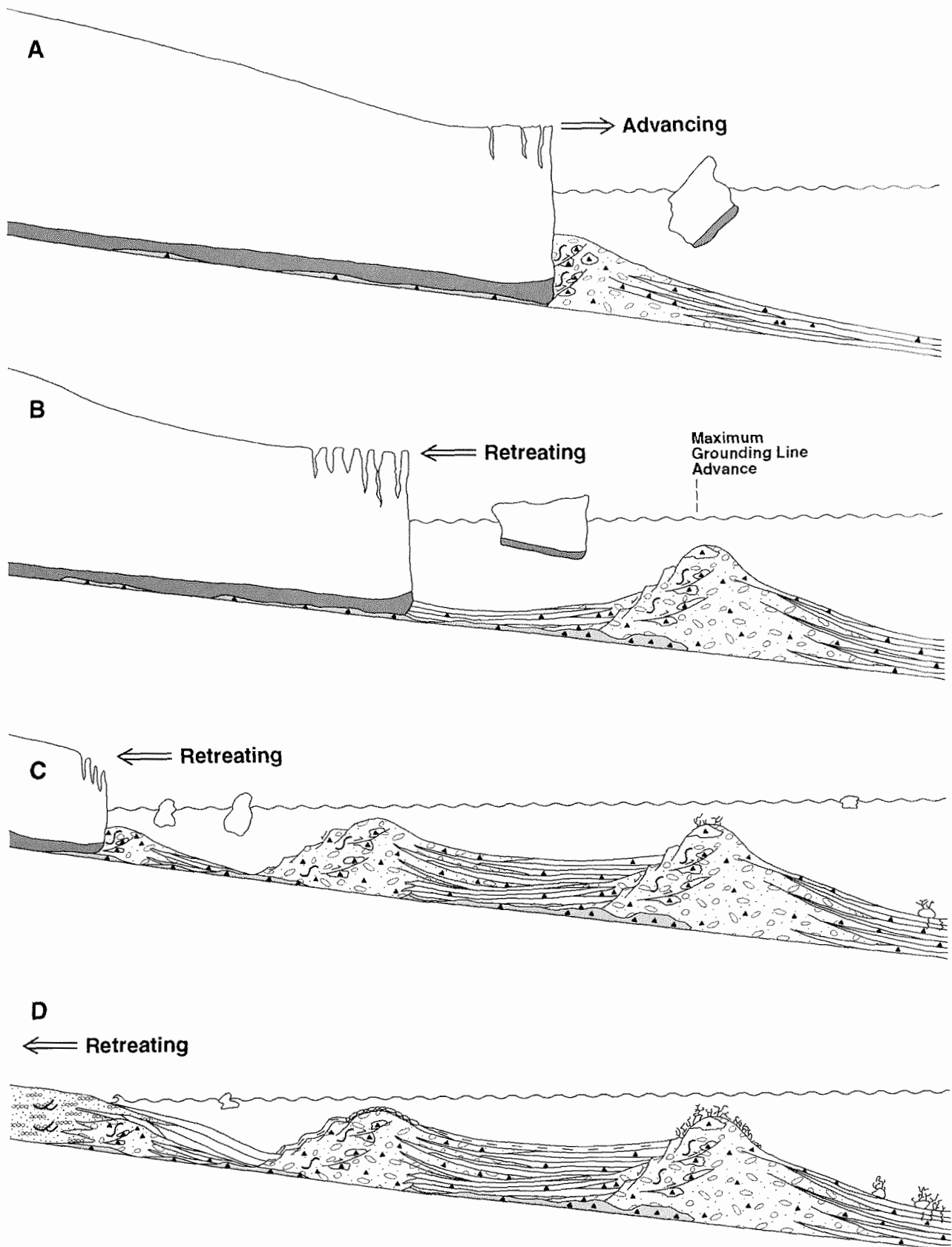
Fig. 2 - An hypothetical glacial advance, retreat and readvance sequence that depicts how facies associations and sequences are thought to have been generated to produce the CRP-2/2A succession. Scale varies in order to allow pertinent features to be shown: vertical scale is ca. 15 000 and the horizontal scale varies between morainal banks ( ca. 140 000) and non-bank areas ( \geq ca. 40 000). The facies sequences are constructed to emphasise variations relative to glacial activity, so water depth does not vary; that is, effects of sea level, isostasy and tectonics are not considered. However, a particular preserved stratigraphic record will vary depending on relative lengths of time a glacier spends within different stages of its advance and retreat modes, the amount of erosion (glacial mainly) and the other variables not considered in relative water depth changes, and their rates and timing relative to the glacial advance and retreat cycle.
