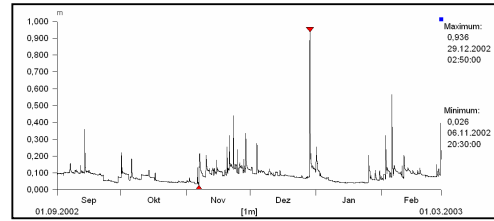
Figure 8. Observed stage (10 min res.) Takkelemo.
