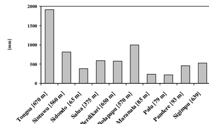
Figure 5. Total precipitation at IMPENSO / STORMA stations, September 2002 – March 2003.
