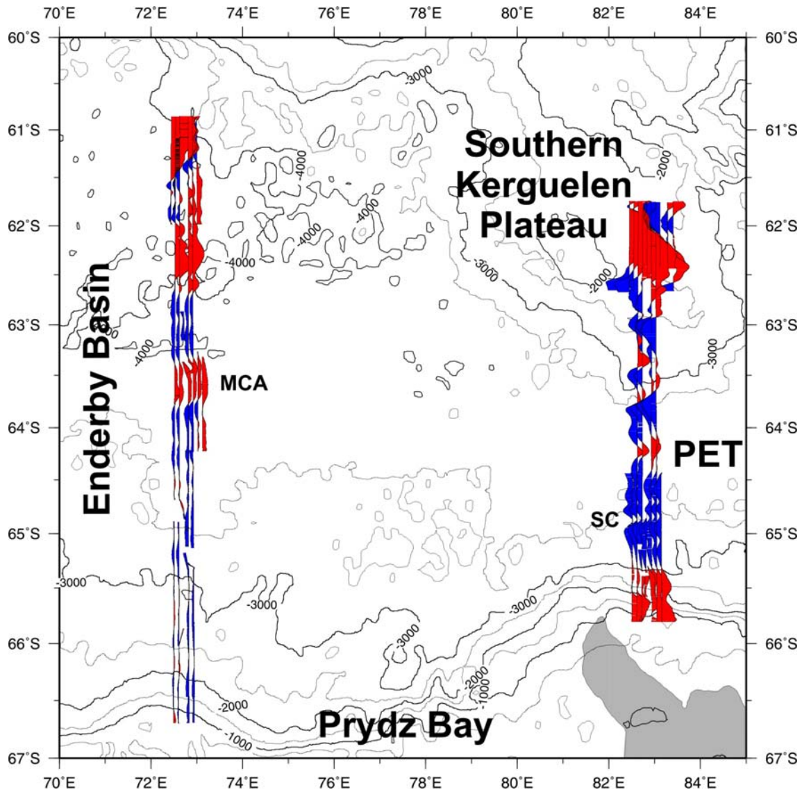
Fig. 3.9: Map with amplitude wiggle-tracks of the heli-magnetic surveys parallel to profiles AWI-20070100 (west) and AWI-20070200 (east). Negative amplitudes of total intensity anomalies are in blue and positive amplitudes are in red. PET = Princess Elizabeth Trough, MCA = Magnetic Coastal Anomaly, SC = former spreading centre
