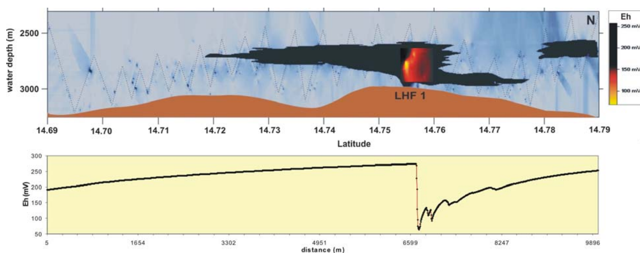
Fig. 1.4.2.3: Anomalies of turbidity and Eh along a south-north orientated tow-yo track (08 MAPR) across the LHF3 and LHF1 and the recorded Eh measurements over the distance of the track.
