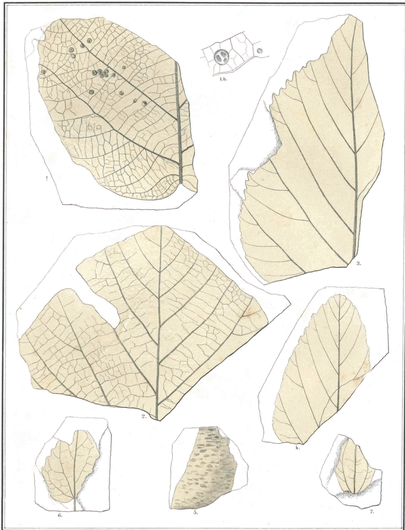
Fig. 1, 2. Pterospermites spectabilis . 3-5. Betula macrophylla . 6, 7. Populus arctica .
