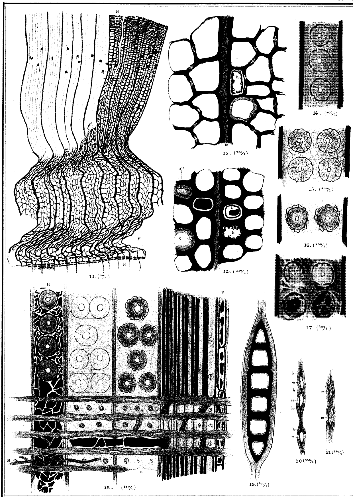
Sequoia canadensis Schröter.
