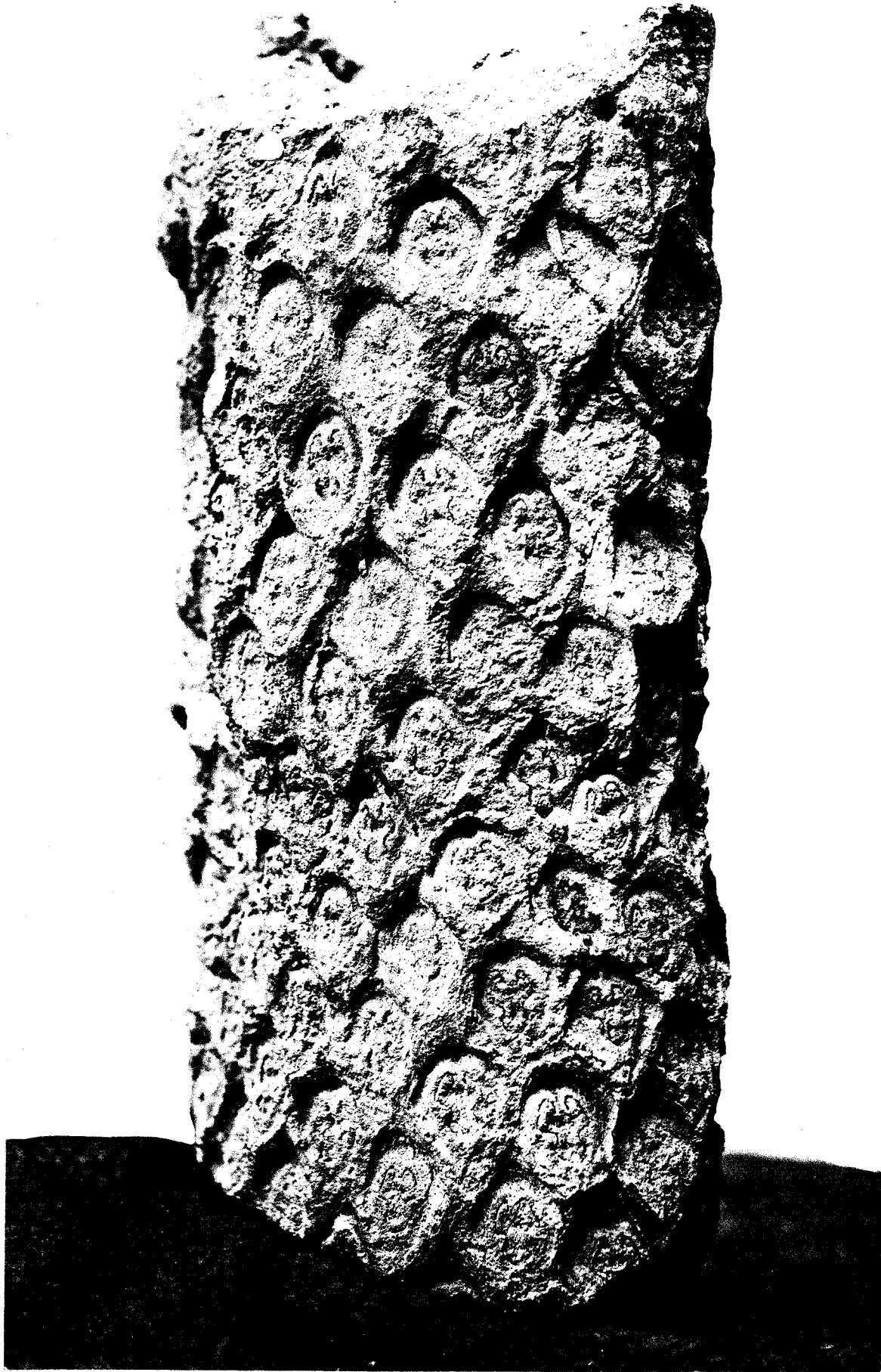
Dicksonia punctata Sternb. sp.
