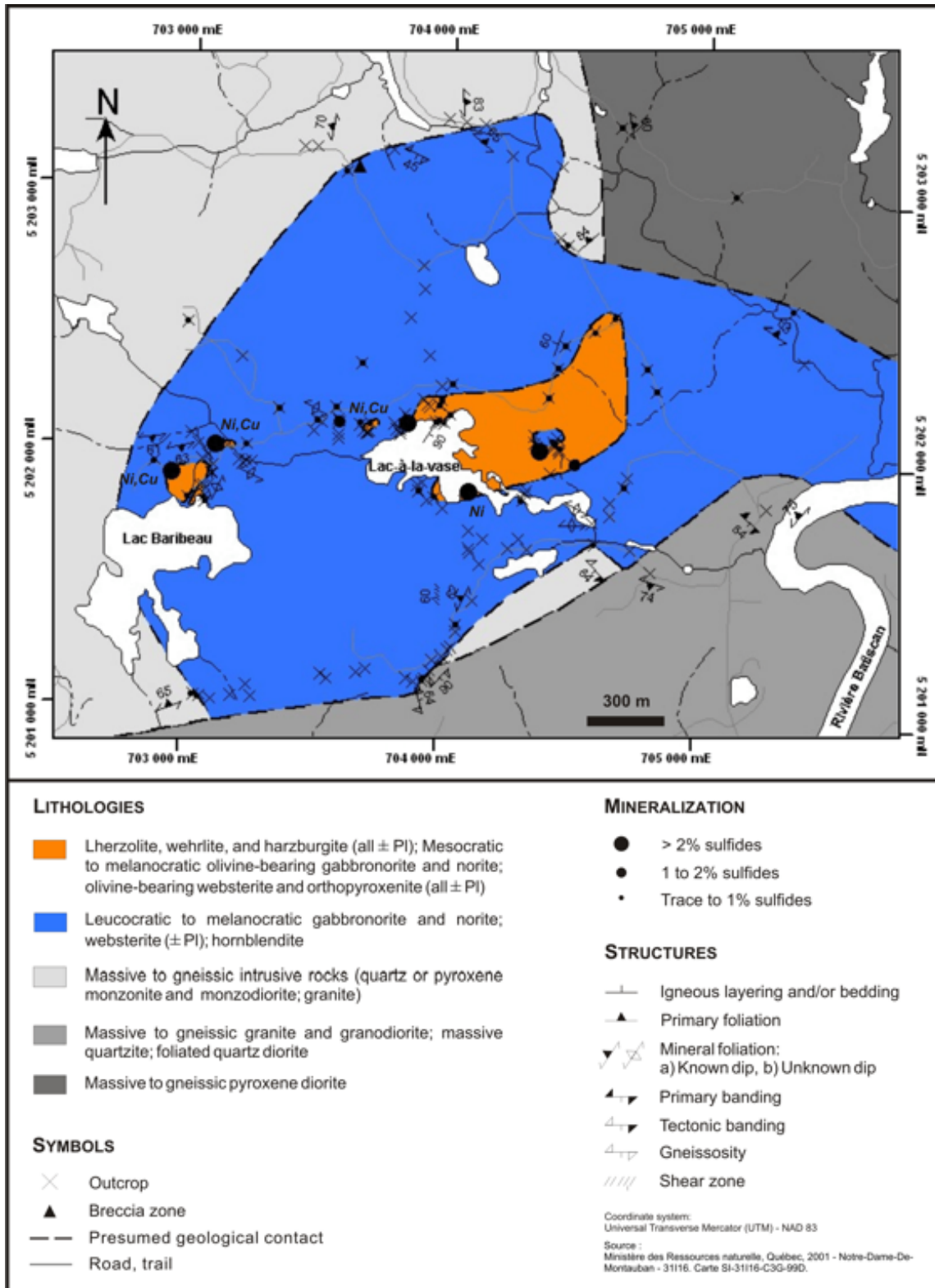
FIG. S3 Geology of the Rousseau prospect (hosted by the Lac à la Vase intrusion) area
