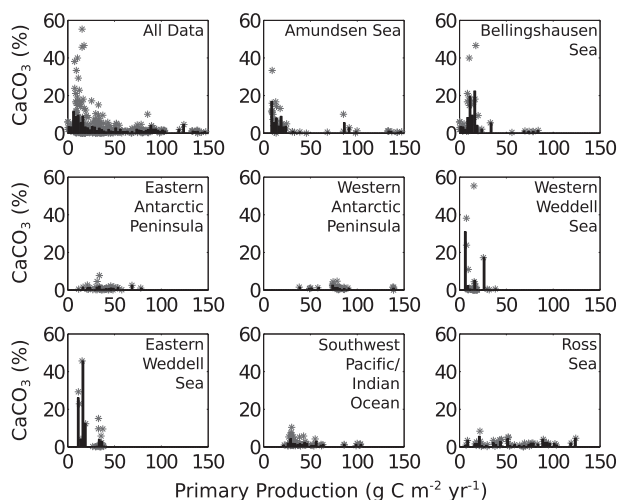
Figure 1. \text{CaCO}_3 versus primary production data for all shelf regions together (upper left) and the different shelf regions separately (name of region indicated in the diagram). Asterisks are original data; bars show means within 2.5 \text{ g C m}^{-2} \text{ yr}^{-1} bins.
