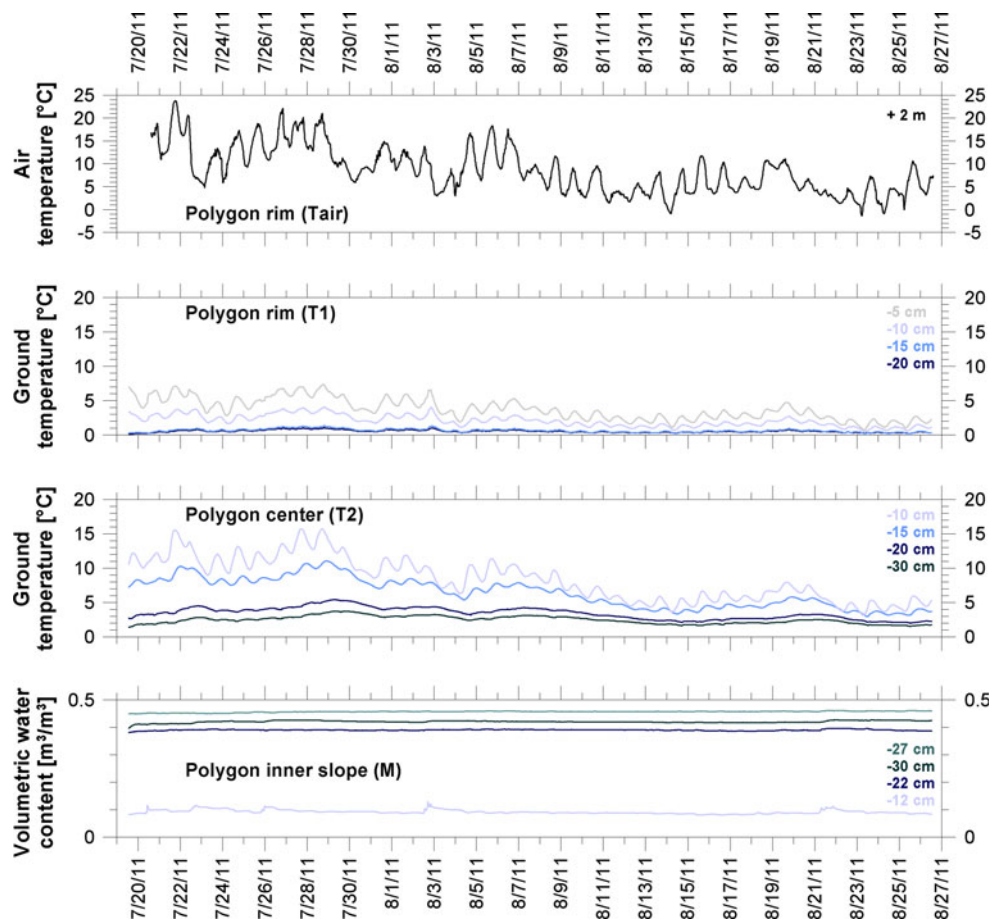
Fig. 4 Air and ground temperatures and soil moisture (volumetric water content) measured in the KYT-1 polygon wall and in the polygon center from July 19 until August 26, 2011
