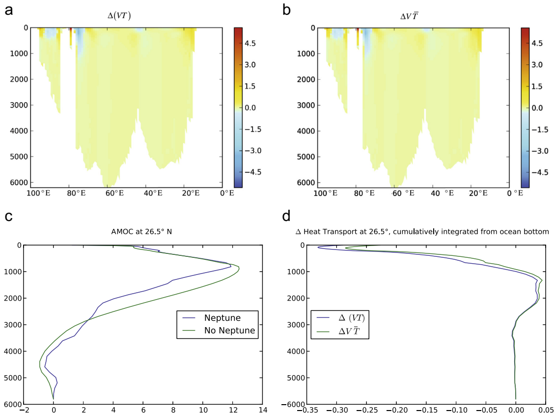
Fig. 22. (a) Difference (Neptune-standard) in northward annual-mean temperature flux along a quasi-zonal section at 26.5°N in ^{\circ}\text{C m s}^{-1} . (b) Difference in velocity times mean of the temperatures from the two runs in ^{\circ}\text{C m s}^{-1} . (c) Zonally integrated meridional flow cumulatively integrated up from the bottom in Sv for the Neptune run (blue line) and standard run (green line). (d) Difference in zonally integrated heat transport cumulatively integrated up from the bottom in PW, calculated using the full temperature flux (blue line) and the approximation, using only the difference in velocities (green line). All plots are for year 2007 of the last forcing cycle.
