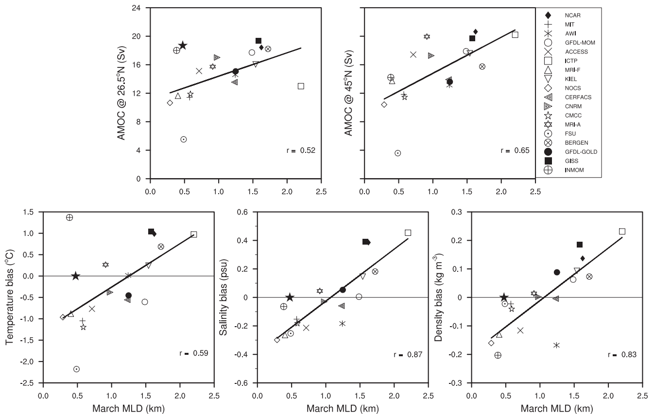
Fig. 18. Scatter plots of the LS March-mean MLD against the AMOC maximum transports at 26.5°N and 45°N (top panels) and against the LS upper-ocean (0–700 m average) potential temperature, salinity, and density biases (bottom panels). Each panel contains the corresponding regression line along with the correlation coefficient. Except for MLD, the model data are for the time-mean. The solid stars in the top left and bottom panels represent the observationally-based March-mean MLD estimate plotted against the 4-year mean RAPID data (April 2004–March 2008) and against no bias, respectively.
