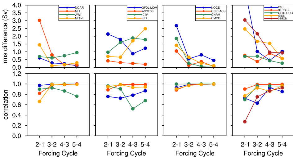
Fig. 2. Root-mean-square (rms) differences (top panels) and correlations (bottom panels) for the AMOC annual-mean maximum transport time series at 26.5°N between consecutive forcing cycles. The first ten years of each cycle are excluded from the analysis to avoid large adjustments associated with the jump in forcing from 2007 back to 1948. The MRI-A data assimilation simulation is not included because it is integrated only for one 60-year cycle.
