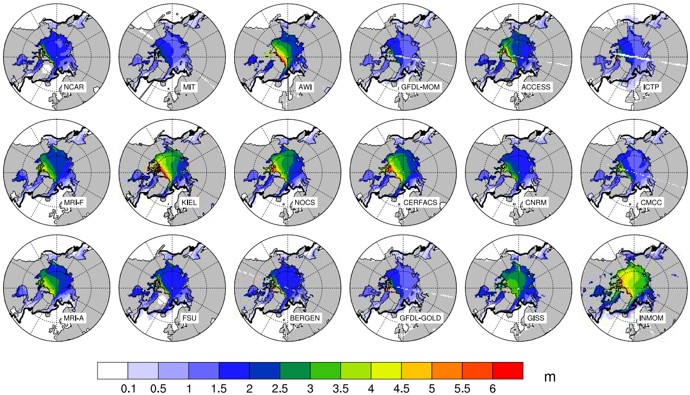
Fig. 15. March-mean sea-ice thickness. The black contour line denotes the 15% observed sea-ice extent from the updated NSIDC data (Cavaliere et al., 1996).
