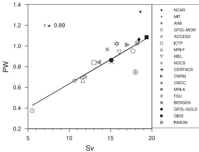
Fig. 7. Scatter plot of the maximum AMOC transport against meridional heat transport (MHT), both evaluated at 26.5°N. The model data are for the time-mean. The solid star denotes the observational AMOC and MHT estimates from the RAPID data. The regression line and correlation coefficient are also shown.
