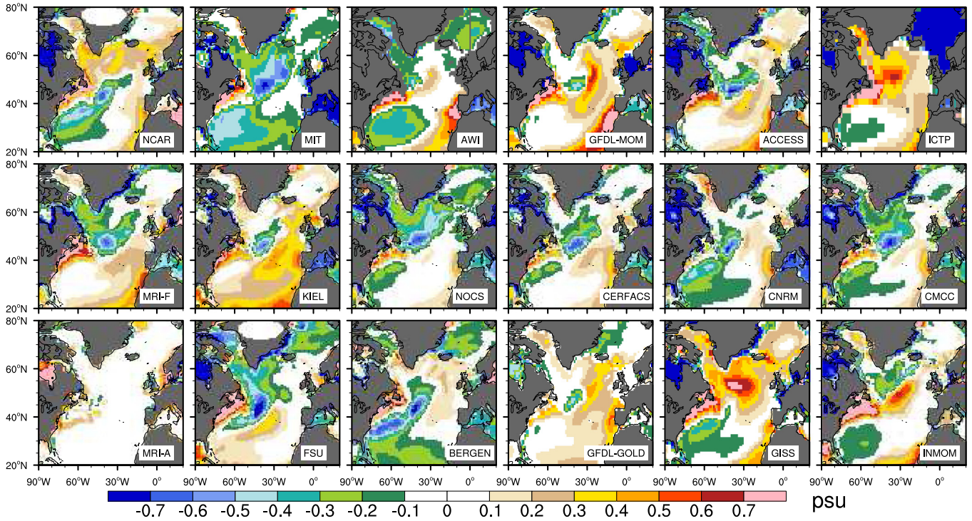
Fig. 9. Time-mean, 0–700 m average salinity model minus observations (Antonov et al., 2010) difference distributions.
