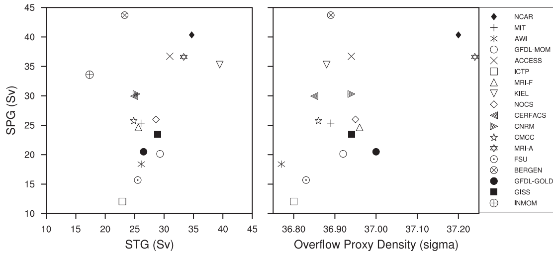
Fig. 16. Scatter plots of the North Atlantic subtropical gyre (SPG) maximum transports against the North Atlantic subtropical gyre (STG) maximum transports (left) and against the overflow proxy density (right). All data are time-mean. Overflow proxy density is not available for INMOM. See text for details of how STG and SPG transports are determined. The overflow proxy density is calculated as the time-mean density of the densest outflow (or southward flow) at 60°N as represented by approximately 1 Sv AMOC transport in density ( \sigma_2 ) space, using Fig. 4.
