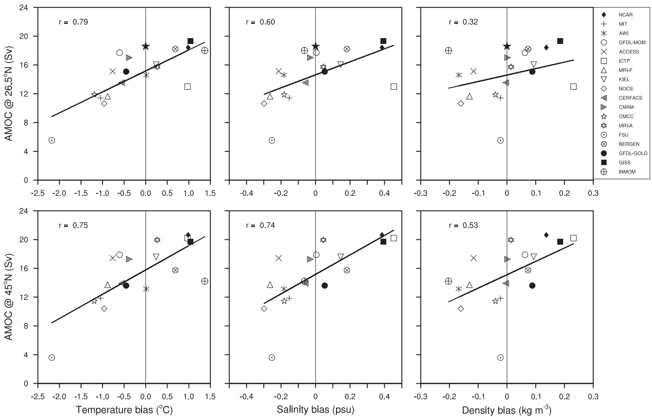
Fig. 17. Scatter plots of the Labrador Sea (LS) upper-ocean (0–700 m average) potential temperature (left), salinity (middle), and density (right) biases against the AMOC maximum transports at 26.5°N (top) and 45°N (bottom). Each panel contains the corresponding regression line along with the correlation coefficient. The model data are for the time-mean. The solid stars in the top panels show the 4-year mean RAPID data (April 2004–March 2008) plotted against no bias. The LS region is bounded by 60°–45°W and 50°–65°N and is indicated in Fig. 8.
