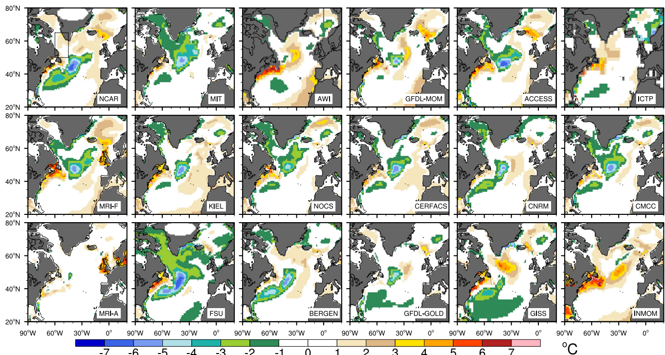
Fig. 8. Time-mean, 0–700 m average potential temperature model minus observations (Locarnini et al., 2010) difference distributions. The boxed area in the NCAR panel indicates the Labrador Sea analysis region.
