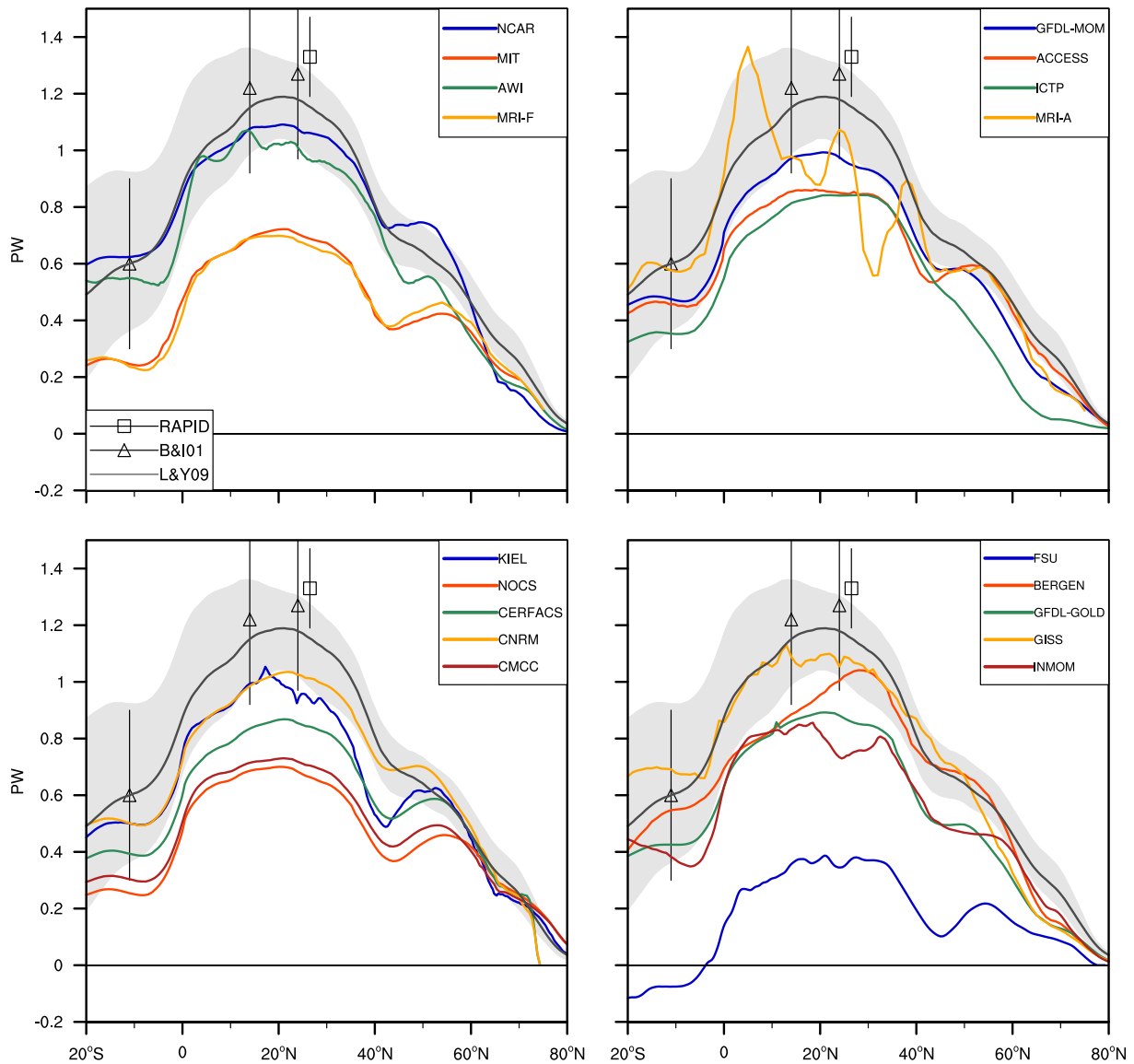
Fig. 6. Time-mean meridional heat transports for the Atlantic Ocean. The black lines denoted by L&Y09 represent implied time-mean transport calculated by Large and Yeager, 2009 with shading showing the implied transport range in individual years for the 1984–2006 period. Direct estimates with their uncertainty ranges from the RAPID data (square; Johns et al., 2011) and from Bryden and Imawaki, 2001 (triangle; B&I01) are also shown.
