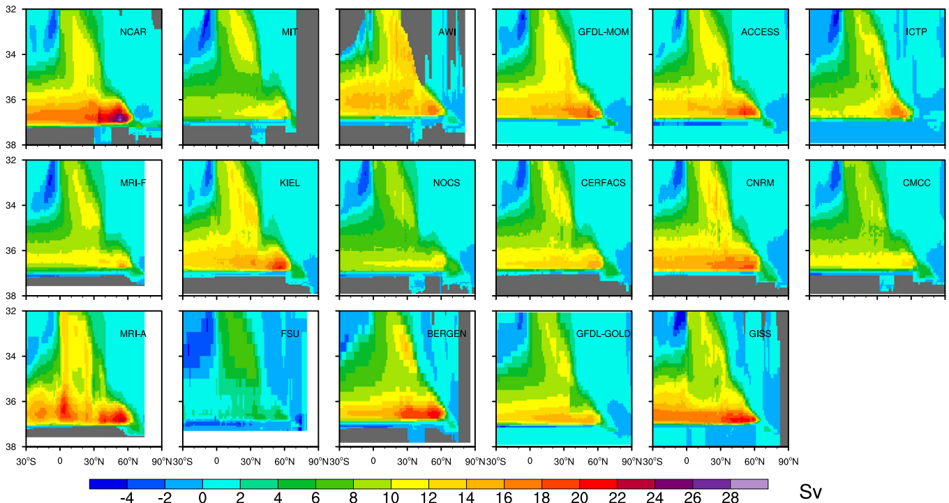
Fig. 4. Same as in Fig. 3 except for AMOC plotted in \sigma_2 density ( \text{kg m}^{-3} ) and latitude space. INMOM distribution is not available.
