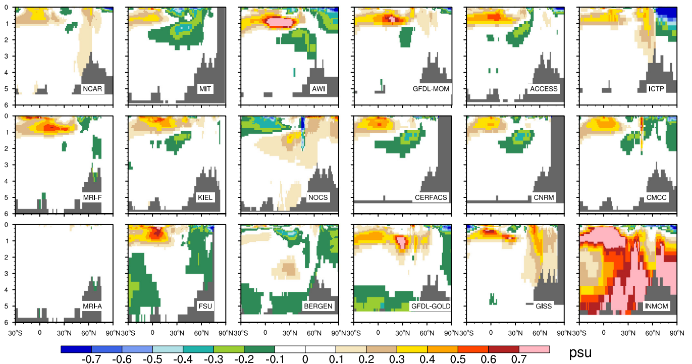
Fig. 12. Same as in Fig. 11 except for salinity, and observations are from Antonov et al., 2010.
