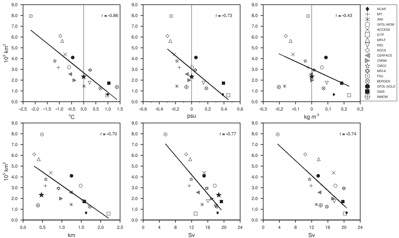
Fig. 20. Scatter plots of the LS March-mean sea-ice area against the LS upper-ocean (0–700 m average) potential temperature (top left), salinity (top middle), and density (top right) biases, and against the LS March-mean MLD (bottom left), AMOC maximum transport at 26.5°N (bottom middle), and AMOC maximum transport at 45°N (bottom right). Each panel contains the corresponding regression line along with the correlation coefficient. Except MLD and sea-ice area, the model data are for the time-mean. The solid stars in the top panels show observational March-mean sea-ice area plotted against no bias. The solid stars in the lower left and middle panels are for the observational March-mean sea-ice area plotted against the observationally-based March-mean MLD and the 4-year mean RAPID data (April 2004–March 2008), respectively.
