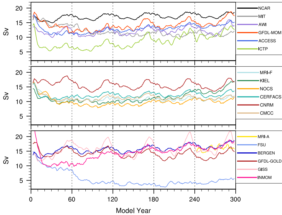
Fig. 1. AMOC annual-mean maximum transport time series at 26.5°N for the entire 300-year integration length. The time series are smoothed using a five-point box car filter. The repeating 60-year forcing cycle, corresponding to calendar years 1948–2007, is indicated by the dashed lines in each panel.
