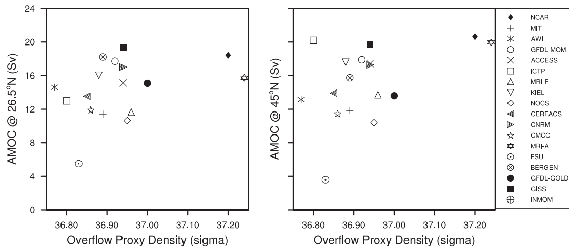
Fig. 19. Scatter plots of the AMOC maximum transports at 26.5°N (left) and 45°N (right) against the overflow proxy density described in Fig. 16. All data are time-mean. Overflow proxy density is not available from INMOM.
