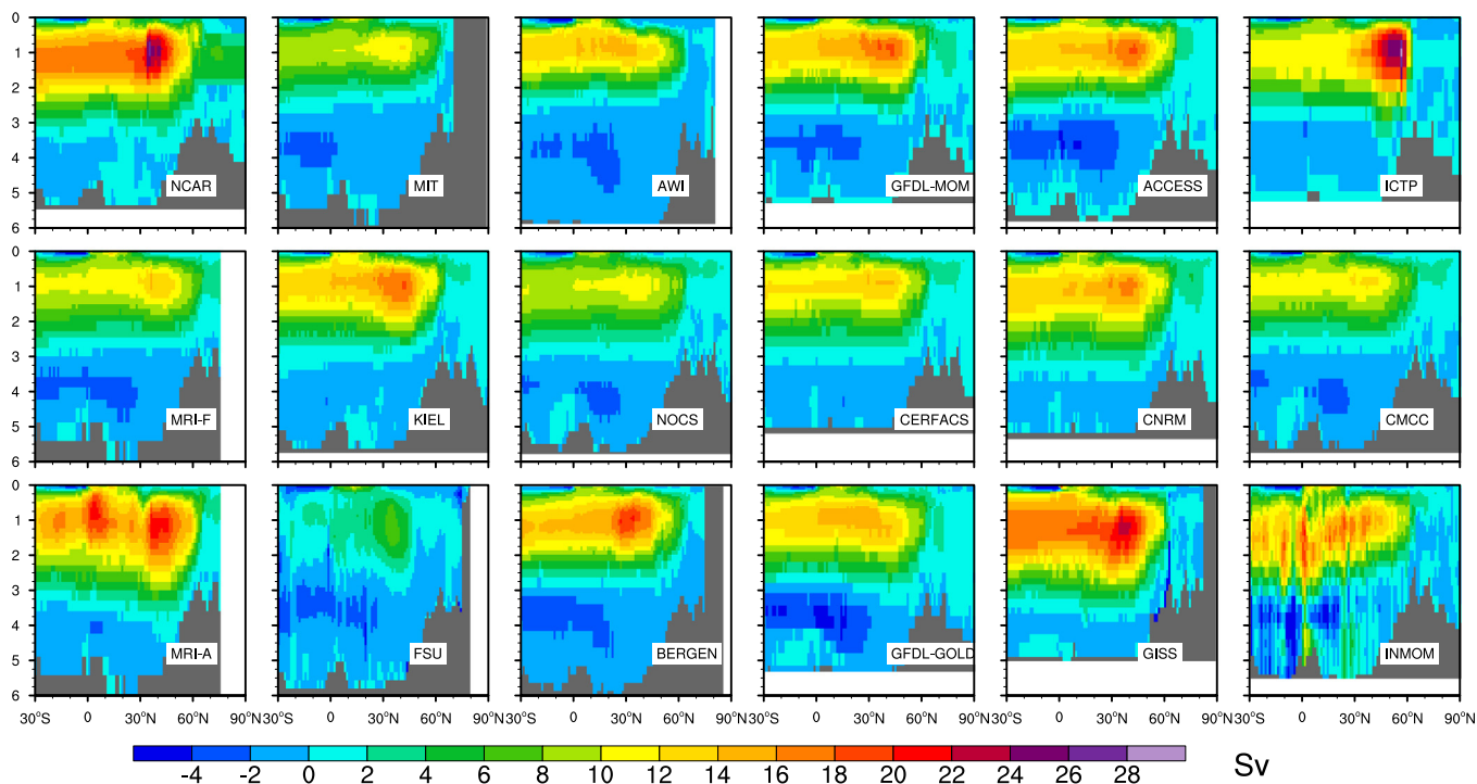
Fig. 3. Time-mean AMOC plotted in depth (km) and latitude space. The positive and negative contours indicate clockwise and counter-clockwise circulations, respectively. In MIT, AWI, MRI-F, MRI-A, FSU, BERGEN, and GISS, the AMOC distributions do not include the high latitude North Atlantic and/or Arctic Oceans, and hence are masked. Unless otherwise noted, the time-mean refers to the 20-year means for years 1988–2007, corresponding to simulation years 281–300, in all the figures.
