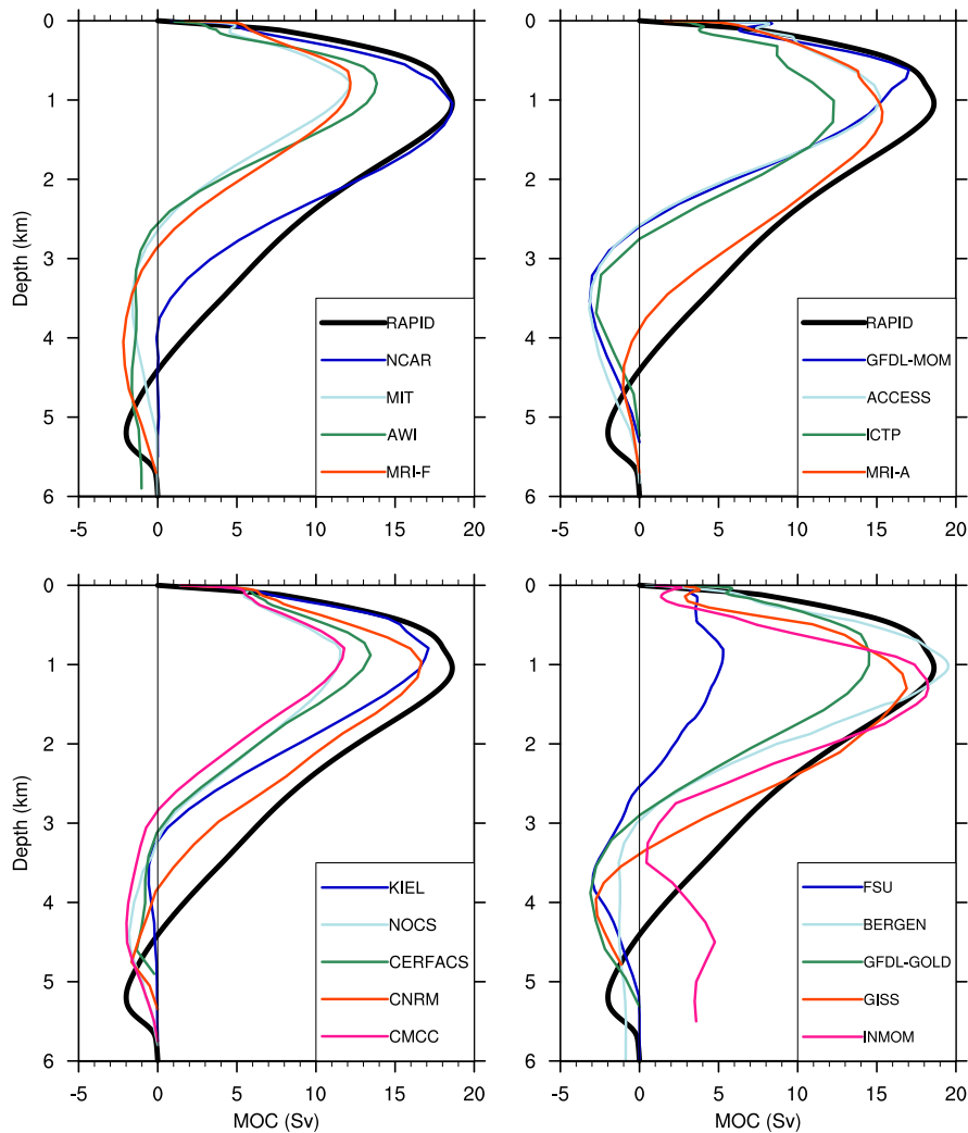
Fig. 5. Years 2004–2007 mean AMOC depth profiles at 26.5°N from model solutions in comparison with the 4-year mean (April 2004–March 2008) RAPID data (thick black lines plotted in each panel).
