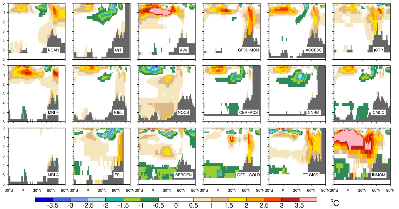
Fig. 11. Time-mean and zonal-mean potential temperature model minus observations (Locarnini et al., 2010) difference distributions for the Atlantic Ocean. In MIT, MRI-F, KIEL, CERFACS, CNRM, MRI-A, FSU, and GISS, the difference distributions do not include the high latitude North Atlantic and/or Arctic Oceans, and hence are masked. The left axis represents depth in km in each panel.
