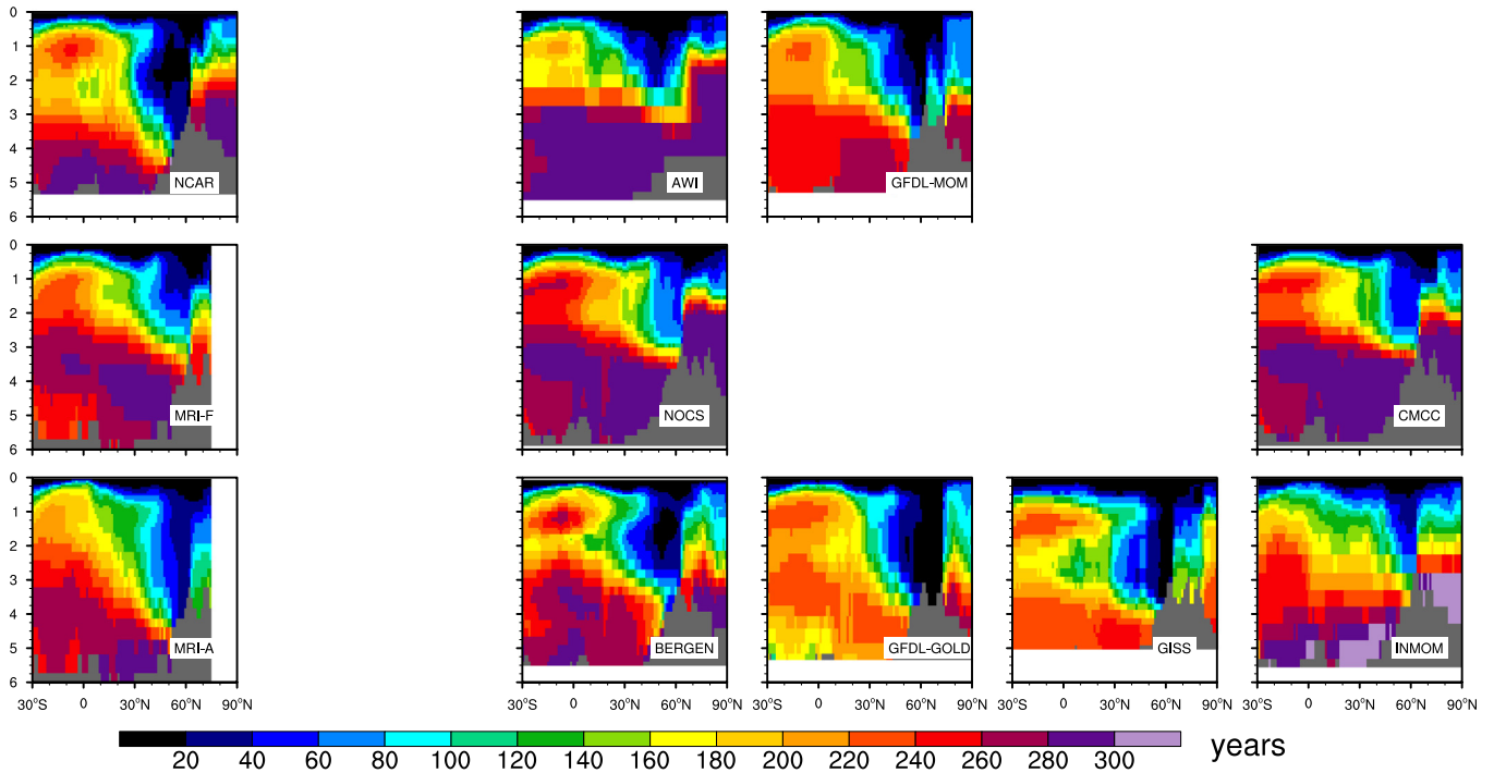
Fig. 14. Time-mean and zonal-mean ideal age distributions for the Atlantic Ocean. Ideal age is not available from MIT, ACCESS, ICTP, KIEL, CERFACS, CNRM, and FSU. In MRI-F and MRI-A, the distributions do not include the Arctic Ocean, and hence are masked. The left axis represents depth in km in each panel.
