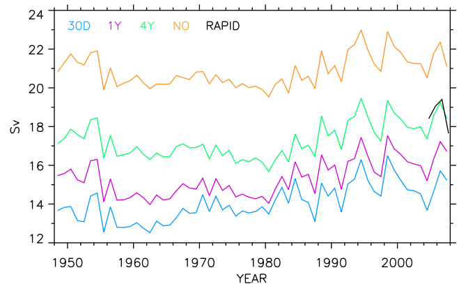
Fig. 21. AMOC annual-mean maximum transport time series at 26.5°N obtained with a preliminary version of the NCAR model using different SSS restoring time scales: 30 days (30D); 1 year (1Y); 4 years (4Y); and infinity (NO), i.e., no restoring. The associated length scale is 50 m. RAPID line represents the observational data from Cunningham et al., 2007. The time series are shown for one forcing cycle.
