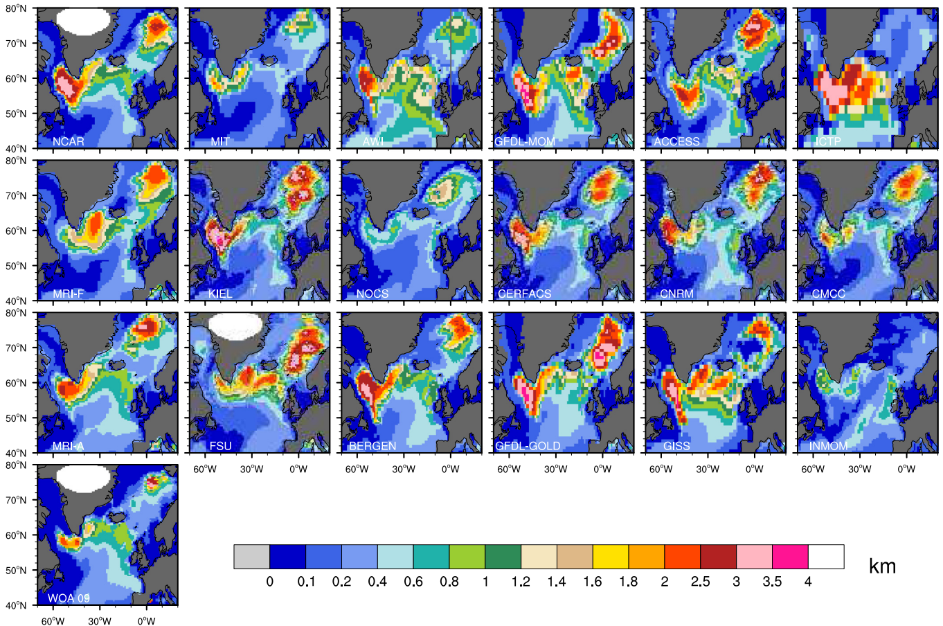
Fig. 13. March-mean mixed layer depth (MLD) based on a \Delta\rho = 0.125 \text{ kg m}^{-3} criterion for the Northern North Atlantic. The panel to the left of the color bar shows MLD calculated from the WOA09 potential temperature (Locarnini et al., 2010) and salinity (Antonov et al., 2010) data.
