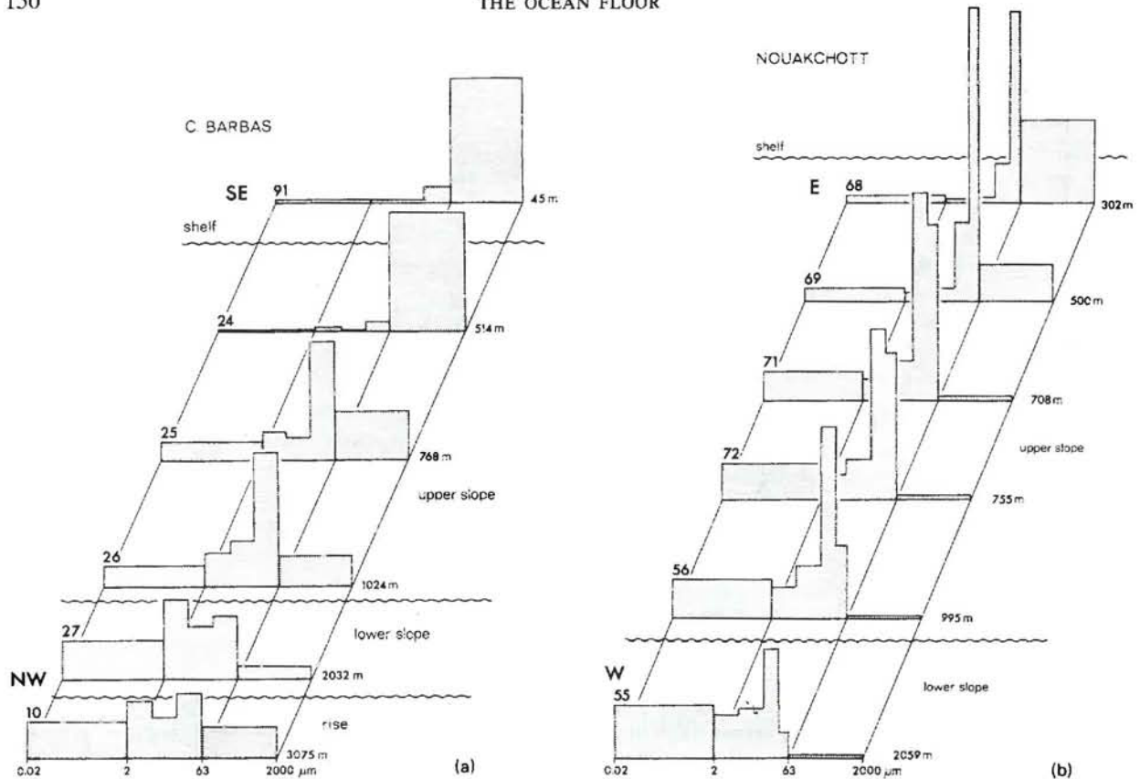
Figure 4 Grain size distribution of surface sediments off: (a) C. Barbass (Figure 1, profile C); and (b) Nouakchott (Figure 1, profile F). Station numbers: Geological Institute, Kiel University (profile C: 91 = 12,391 etc., profile F: 68 = 13,268 etc.). Silt fractions are 2–6, 6–20, and 20–63 \mu\text{m} . Coarse silt is separated in (b) into 20–40 and 40–63 \mu\text{m}
