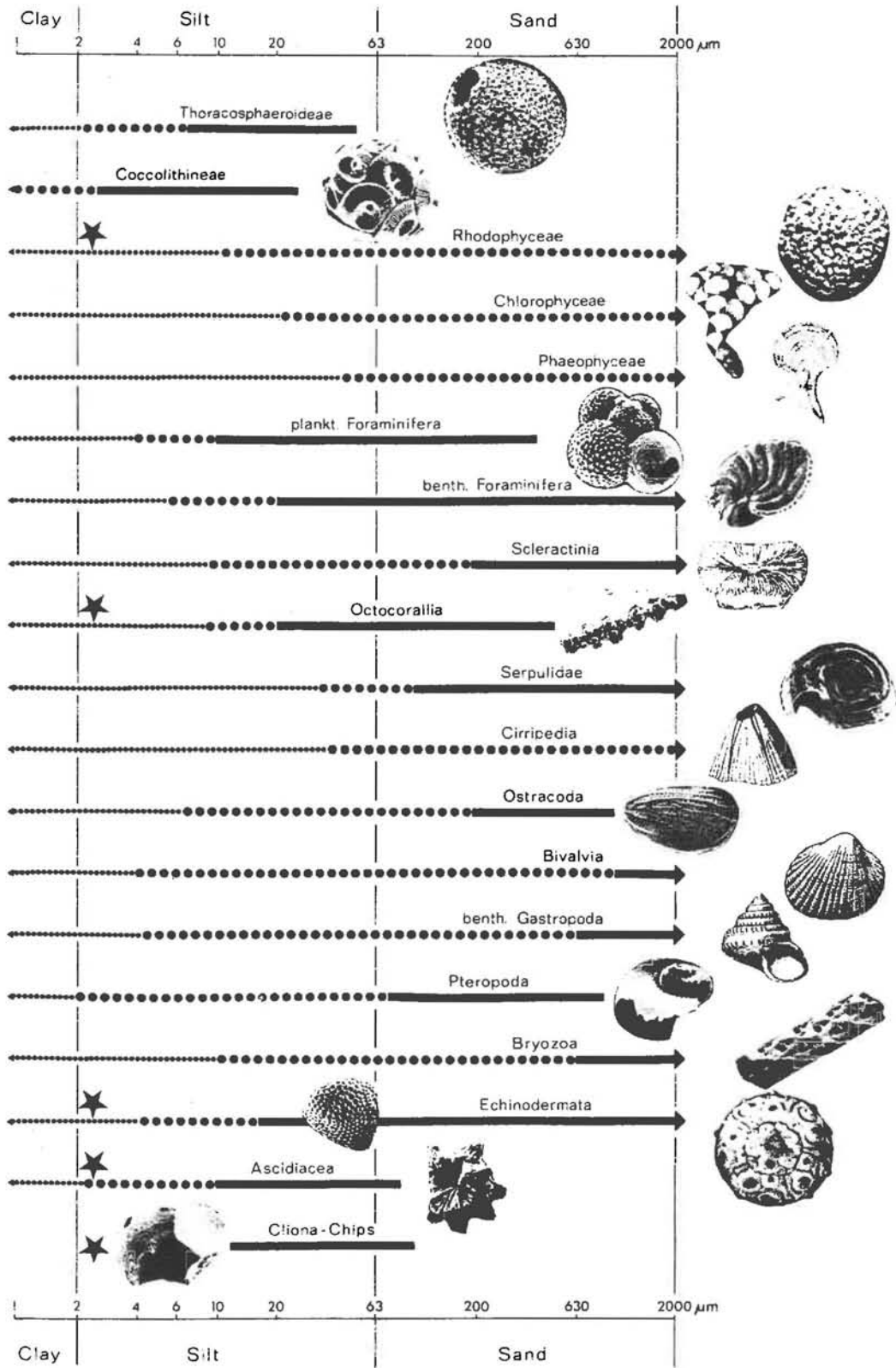
Figure 8 Grain sizes and identification limits of biogeneous carbonate skeletons or particles. Asterisks mark downslope transport indicators used off northwest Africa
