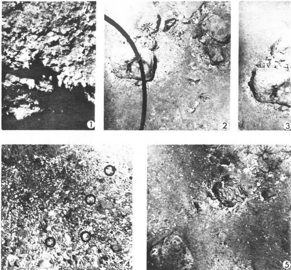
Figure 16 (1) Corals living in 170 m water depth. Cayar Canyon wall. 14^{\circ} 59'N , 17^{\circ} 18'W , Valdivia cruise 10, 1975, station 13303-1. (2,3) Rockfall blocks surrounded by mussel shell scour marks. Casamance Canyon, station 13316-1, 13^{\circ} 31'N , 17^{\circ} 45'W , 1760 m. (4) Same station: mussel shells, some of them hollow side up and filled with mud. (5) Same station: rockfall material with possible organic borings on blocks 1 and 2. Scale: heights about 1 m
