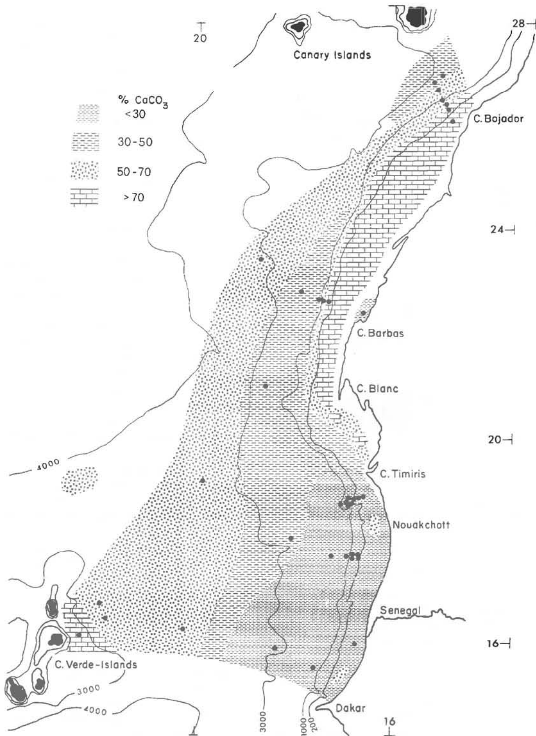
Figure 5 Carbonate content of surface sediments (weight % CaCO 3 )
