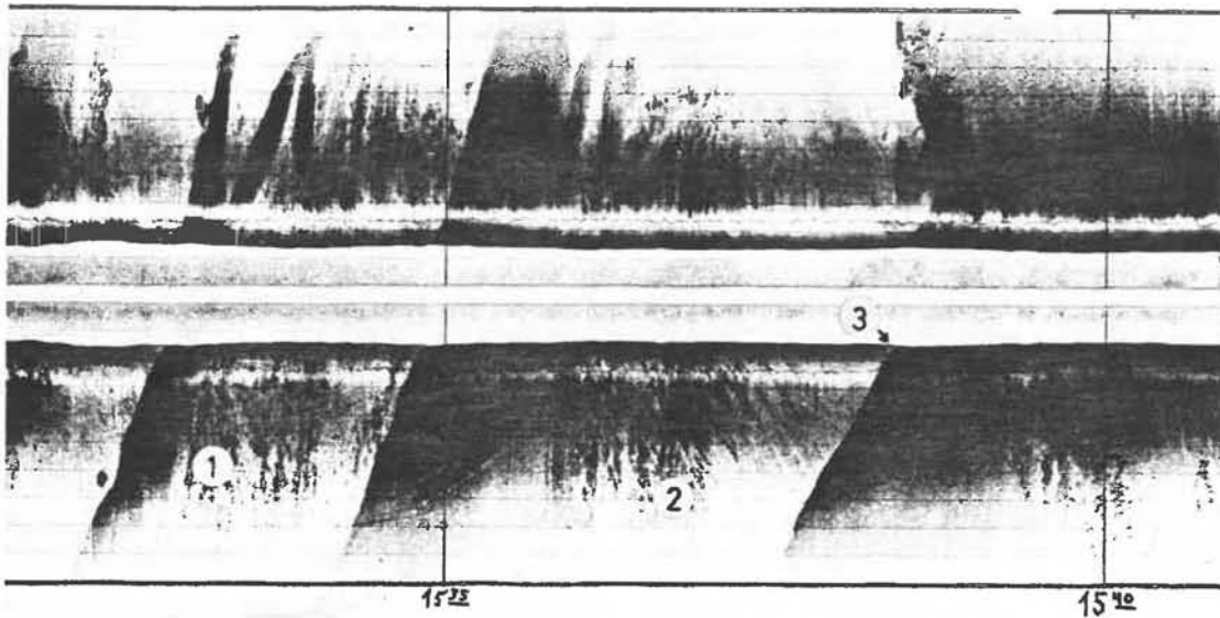
Figure 9 Shelf sediment patchiness off C. Barbas. Side scan sonograph from area X, Figure 1. Asymmetrical window cut through fine, upper sand layer (light) exposing coarse sand beneath (dark) fields of Pinna with lineations (1,2). At (3) sharp, roughly 1 m high, southeast-facing slope of window, approximately 56 m water depth. Sonograph is about 2 km long and each half about 170 m wide. (After Newton et al. (1973))
