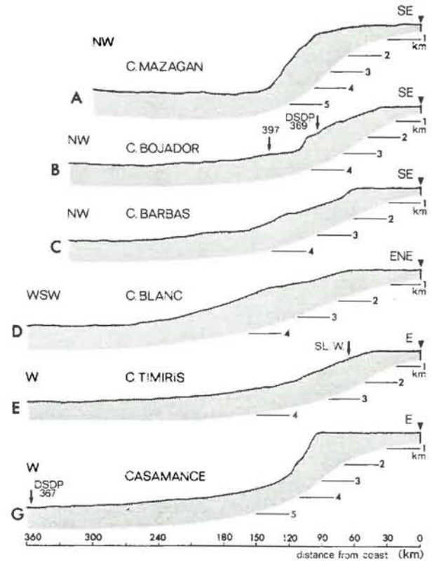
Figure 2 Continental margin profiles between Morocco and south Senegal. For location of profiles A–G see Figure 1; vertical exaggeration 15:1; SL. W., slope wall as mentioned on page 148
