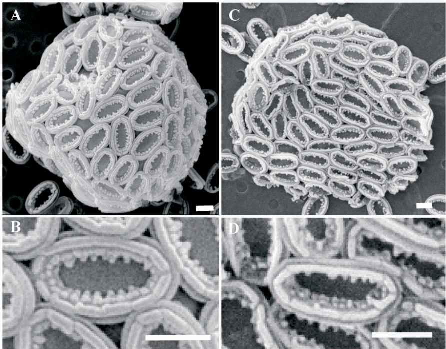
Fig. 1 Scanning electron micrographs of Pleurochysis cf. pseudoroscoffensis in the experiments with 1% CO 2 in the day 9. A and B: control; C and D: 1% CO 2 . Scale bar: 1 μm.
