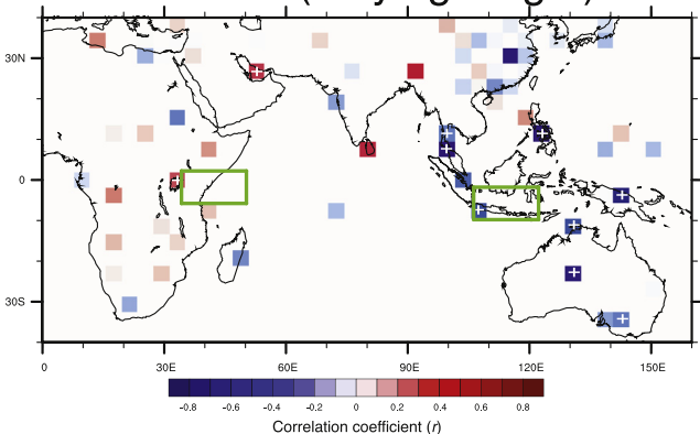
Fig. 2. Performance of ECHAM4 SWING S1B simulation (left) in simulating observed SOND precipitation (top) and isotopic (bottom) anomalies from 1958 to 2003. Shading represents the strength and sign of correlation, and black contours denote correlations where p < 0.05 . In the lower-right figure, box shading denotes the strength and sign of correlation, and correlations significant at p < 0.05 are marked with a +. Green boxes denote the locations of East Africa and Southwestern Indonesia boxes used throughout our analysis of the SWING simulation. Precipitation data are from the CPC Merged Analysis of Precipitation (CMAP; available at http://www.esrl.noaa.gov/psd/data/gridded/data.cmap.html ) from 1979 to 2003. Precipitation isotopic data are from the International Atomic Energy Agency-Global Network of Isotopes in Precipitation (GNIP; http://isohis.iaea.org ).
