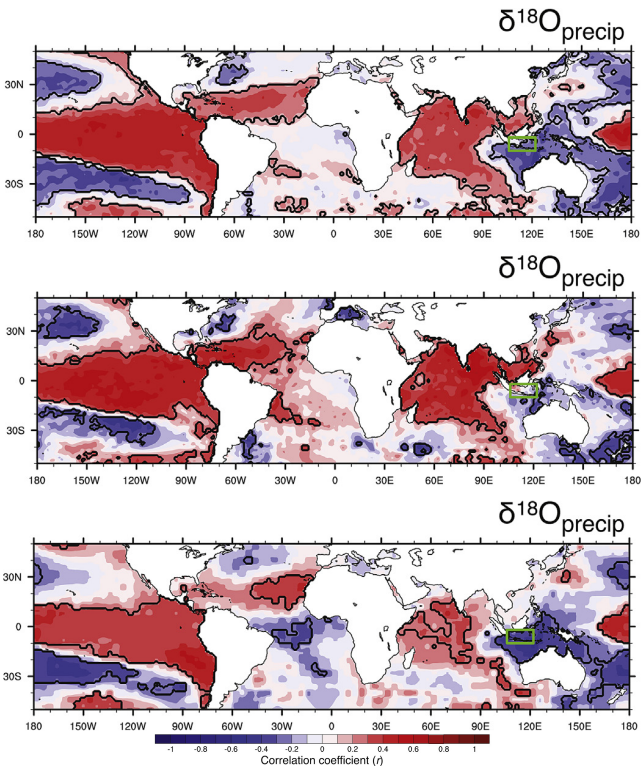
Fig. 8. Correlation between SW Indonesian P and \delta^{18}\text{O}_{\text{precip}} (SOND) and SST (SOND). Top: the full SWING simulation (1870–2003). Middle: the period of strong ZWI/ \delta^{18}\text{O}_{\text{precip}} correlation in SW Indonesia (1945–1980). Bottom: the period of weak ZWI/ \delta^{18}\text{O}_{\text{precip}} correlation in SW Indonesia (1895–1930). Shading, black contours, and green box are as in Fig. 2. All data have been high-pass filtered to preserve interannual and subdecadal variability.
