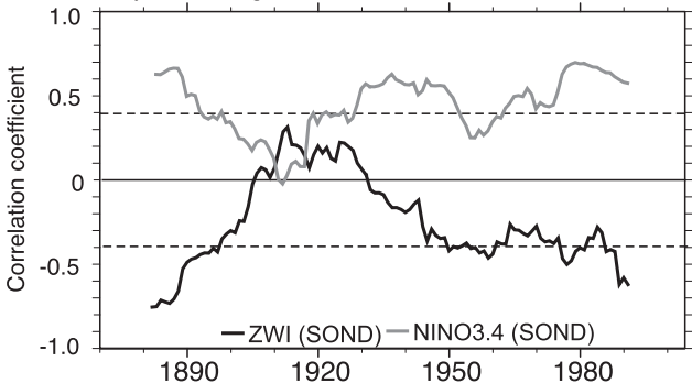
Fig. 7. Top: 25-year running correlations between SW Indonesian P (SOND), ZWI (SOND), and NINO3.4 (SOND) during the SWING simulation. Bottom: As in top, but for SW Indonesian \delta^{18}\text{O}_{\text{precip}} . Dashed lines denote the 95% significance level.
