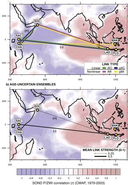
Fig. 12. Map showing the locations of the 6 isotopic proxy records used in our synthesis. Yellow circles, site locations of Socotra Island (SOC), Sacred Lake (SAC), Lake Challa (CHA), Lake Lading (LAD), Flores (FLO), and the Makassar Strait (MAK). Shaded regions represent the correlation between ZWI and precipitation amount during the SON season using NCEP Reanalysis winds and CMAP precipitation, 1979–2003. Bold contours indicate correlation is significant at p < 0.05 . a) Results of similarity tests using each site's published age model and a ~400 year detrend to remove long-term variability. Significant linear links are shown in blue (iXCF) and green (gXCF) lines, and nonlinear links are shown in pink (IMI) and yellow (gMI) lines. For the linear links, (+) and (-) symbols indicate the sign of the correlation using the gXCF estimator. b) Results of similarity tests using ensembles of 100 perturbed age models for each site (see text). Only links that attained a mean link strength of 0.25 or 0.5 within the multi-centennial timescale are shown. The (+) and (-) symbols indicate the sign of the correlation when only the gXCF is considered.
