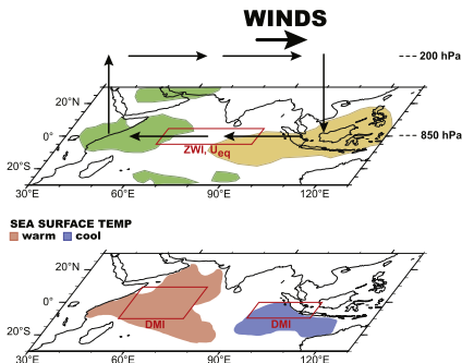
Fig. 1. Schematic illustration of the anomalous components of wind, precipitation, and sea surface temperature observed during an IOZM positive event. Adapted from Saji et al. (1999), Saji et al. (2006), and Schott et al. (2009). Red boxes outline the regions used to calculate the Zonal Wind Index, U_{eq} , and the Dipole Mode Index, discussed in text.
