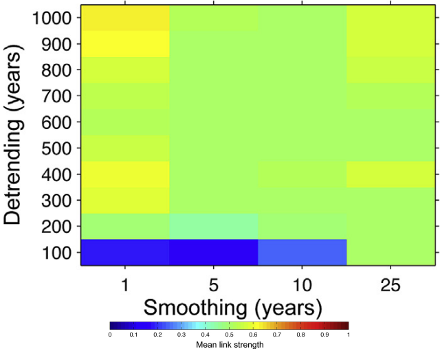
Fig. 13. Mean link strengths of age-perturbed ensembles using all similarity estimators (gXCF, iXCF, gMI, iMI) under combinations of smoothing (x-axes) and detrending (y-axes). In each plot, the quadrants correspond to the following: upper-left, sub-decadal variability with long-term trends preserved; lower-left, sub-decadal variability with long-term trends removed; upper-right, multi-decadal variability with long-term trends preserved; lower-right, multi-decadal variability with long-term trends removed. Centennial and multi-centennial variability are best preserved between 100–300 and 400–600 years, respectively (see text and table of defined timescales). Note that most analyses fail when the detrending window is too small (<100 years).
