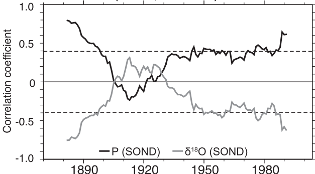
Fig. 4. Top: 25-year running correlations between SOND ZWI, precipitation, and \delta^{18}\text{O}_{\text{precip}} during the SWING simulation for East Africa (top) and SW Indonesia (bottom). Refer to Fig. 2 for locations of East Africa and SW Indonesia boxes. Dashed lines denote the 95% significance level.
