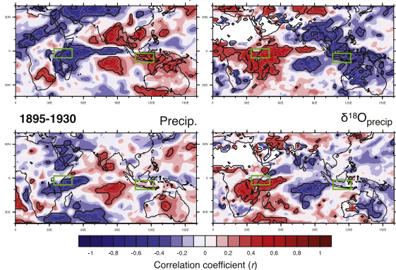
Fig. 5. Correlations between ZWI, P, and \delta^{18}\text{O}_{\text{precip}} in the ECHAM4 SWING simulation. Top, full simulation (1870-2003). Middle, period of strong ZWI/ \delta^{18}\text{O}_{\text{precip}} correlation (1945-1980). Bottom, period of weak ZWI/ \delta^{18}\text{O}_{\text{precip}} correlation (1895-1930). Shading, black contours, and green boxes are as in Fig. 2.
