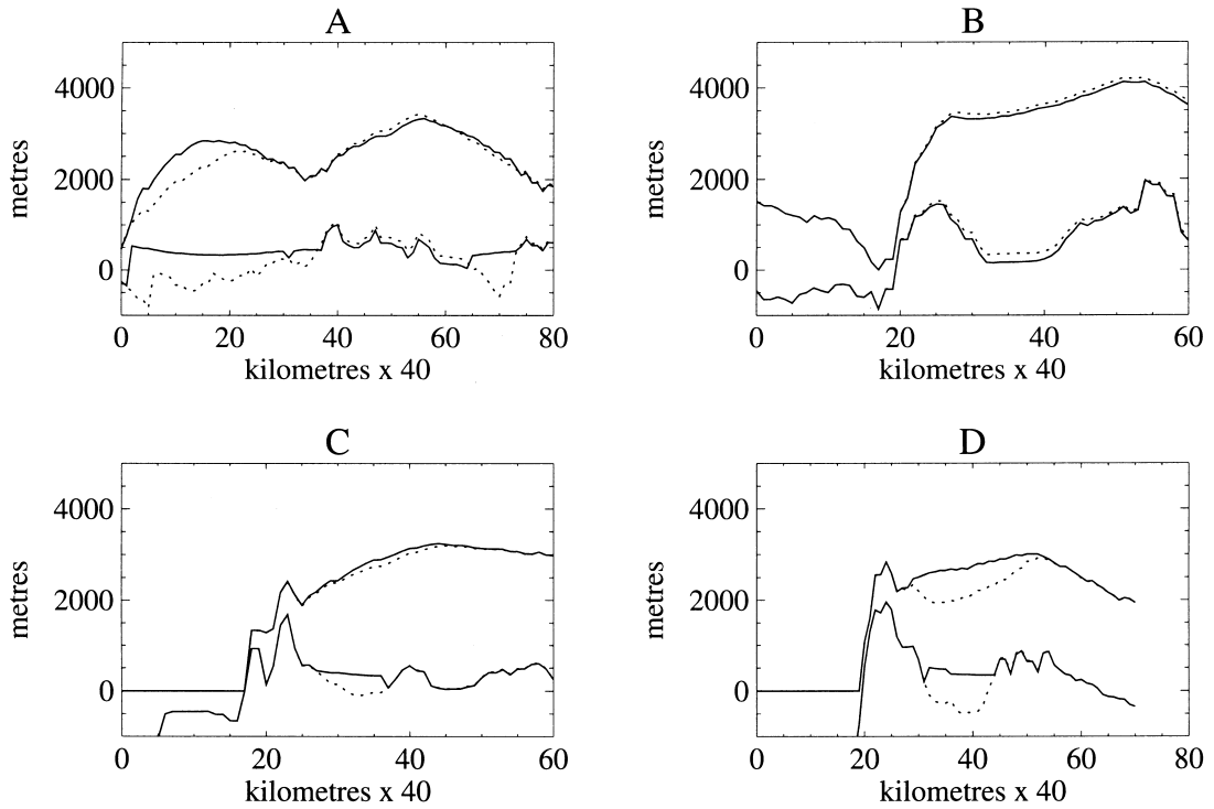
Fig. 9. The impact on ice surface and bedrock elevations of lowering the sub-glacial troughs in the Wilkes–Pensacola Basin. Bedrock elevations changes can be seen in all the transects. Transects A–D as in Fig. 3.
