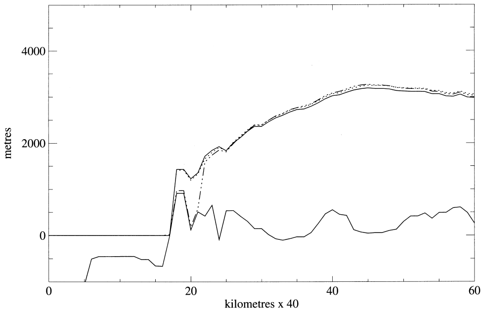
Fig. 6. As in Fig. 5C, but showing the change in ice-surface elevations across the Dry Valleys region resulting from applying different climate profiles. Again, present day ice elevations are displayed with a continuous line, ice surfaces resulting from a +5°C temperature profile is shown with a dotted line, and the ice surface resulting from a +10°C temperature profile is shown with a dash/dot line. When the latter climate is applied, the ice-sheet margin retreats to the Wilkes–Pensacola Basin away from the lowered Dry Valleys block.
