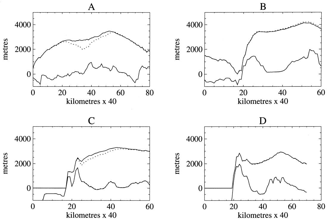
Fig. 10. The impact on ice surface and bedrock elevations of lowering five troughs through the Transantarctic Mountains between the central ranges and the Dry Valleys region. The transects are the same as those used in Fig. 3. These transects do not cross-cut the mountains by the infilled troughs, so the change in bedrock is not apparent, but do show the change in ice surface elevations resulting from the infilling of the troughs.
