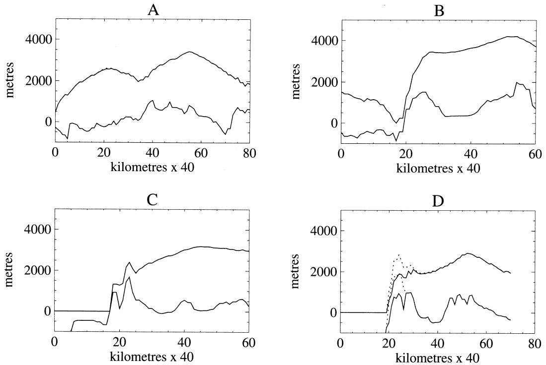
Fig. 7. The impact on the ice surface and bedrock elevations of lowering Victoria Land by 1 km, shown using the same four transects as Fig. 3. The change in bed elevations can be seen in (D), which shows the transect across the Victoria Land region. Lowering the bedrock elevation leads to the loss of the present ice centre over that region.
