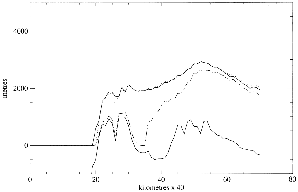
Fig. 8. As in Fig. 7C, but showing the change in ice surface elevations over Victoria Land resulting from applying different climate profiles: present-day (continuous line), +5°C (dotted line), +10°C (dash/dot line).
