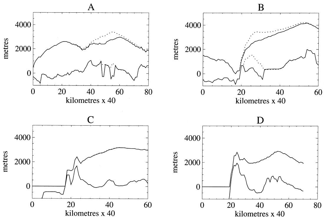
Fig. 3. The impact on ice-surface and bedrock elevations of lowering the central Transantarctic Mountain ranges by 1 km, using four transects cross-cutting the mountains and their hinterlands. (A) The profile along the Wilkes–Pensacola Basin showing the present-day ice-surface and bedrock (dotted lines) and the impact on the ice-surface and bedrock elevations resulting from lowering the bedrock of the central ranges by 1 km (continuous line). (B) As in (A), but the transect runs from the Ross Sea across the central ranges to the centre of the ice sheet. The lower dotted line shows clearly the effect of removing 1 km of bedrock from the rift margin upwarp. The upper two lines show the impact of the bedrock change on ice-surface elevations. (C) As in (A), but the transect runs from the Ross Sea across the Dry Valleys and Royal Society Range region and through the Wilkes–Pensacola Basin. (D) As in (A), but the transect runs from the Ross Sea across Victoria Land and the Wilkes–Pensacola Basin.
