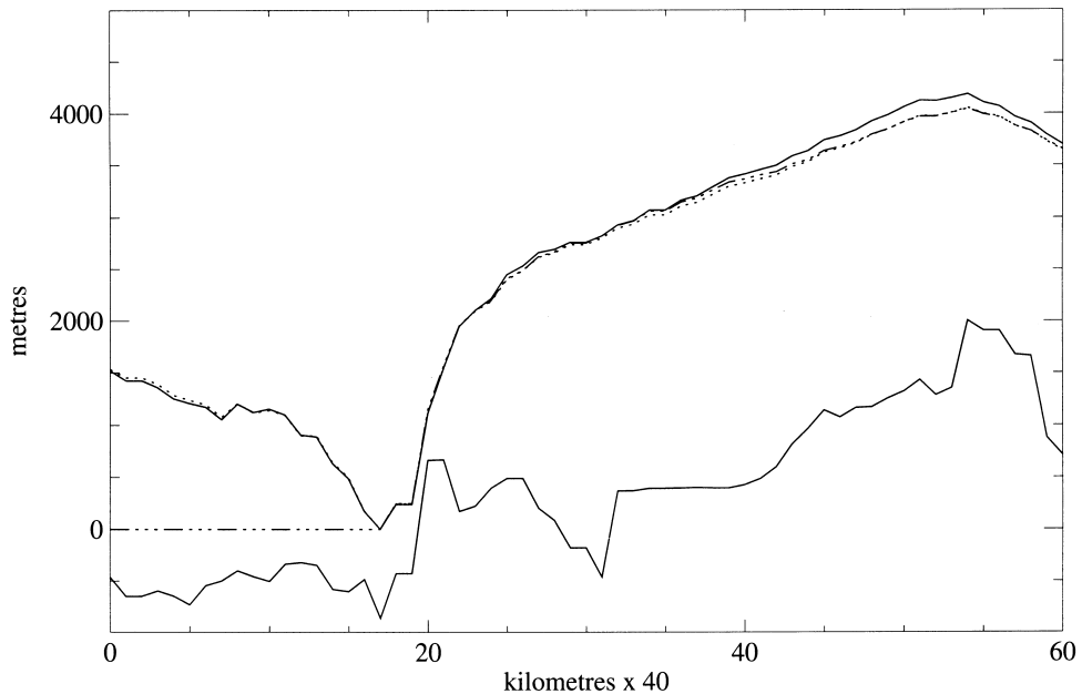
Fig. 4. The transect is the same as Fig. 3B, but this time showing the change in ice-surface elevation resulting from using different climate profiles across the central ranges: the present day (continuous line), +5°C (dotted line), and +10°C (dash/dotted line). The impact of the changing climate on the ice-surface over the lowered central ranges of the Transantarctic Mountains, in the centre of the profile, is negligible.
