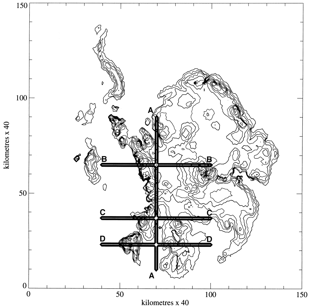
Fig. 2. The Antarctic bedrock, showing the position of the bedrock that was raised or lowered in the experiments and the transects shown in Figs. 3–10. Contours are every 500 m and the bold lines are every 1000 m.
