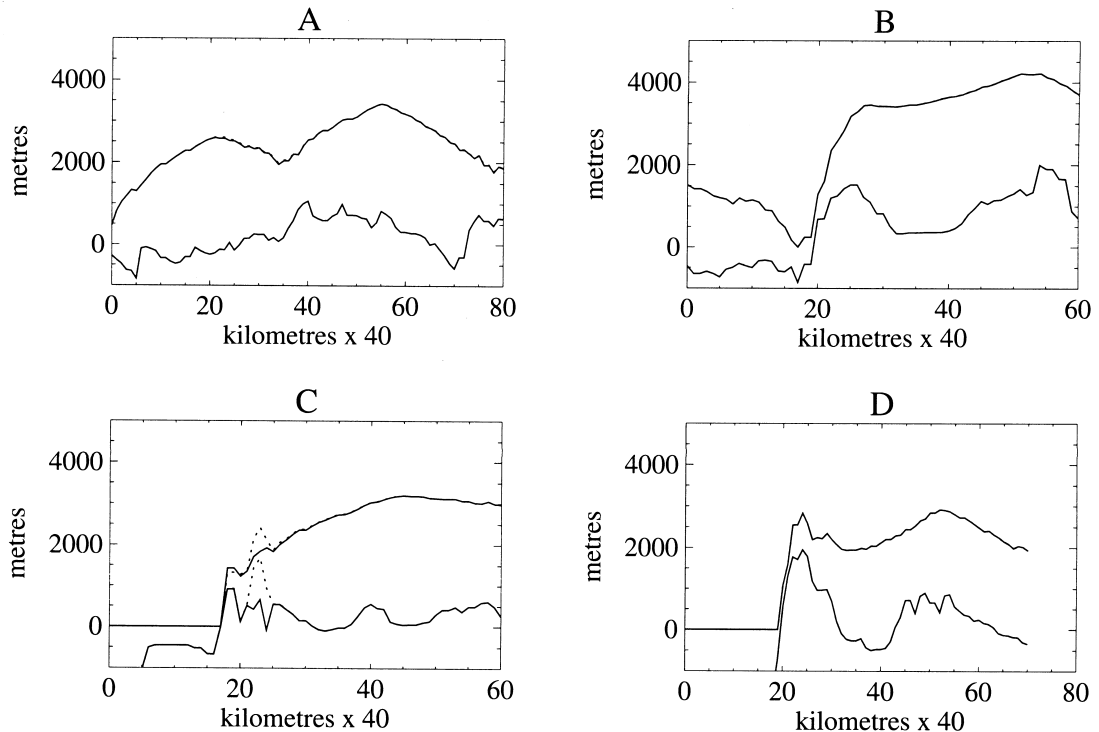
Fig. 5. The impact on the ice surface and bedrock elevations of lowering the Dry Valleys region by 1 km, shown using the same four transects used in Fig. 3. The removal of Dry Valleys bedrock is displayed in Fig. 5C, which also shows the resultant loss of the present ice centre that overlies the present region.
