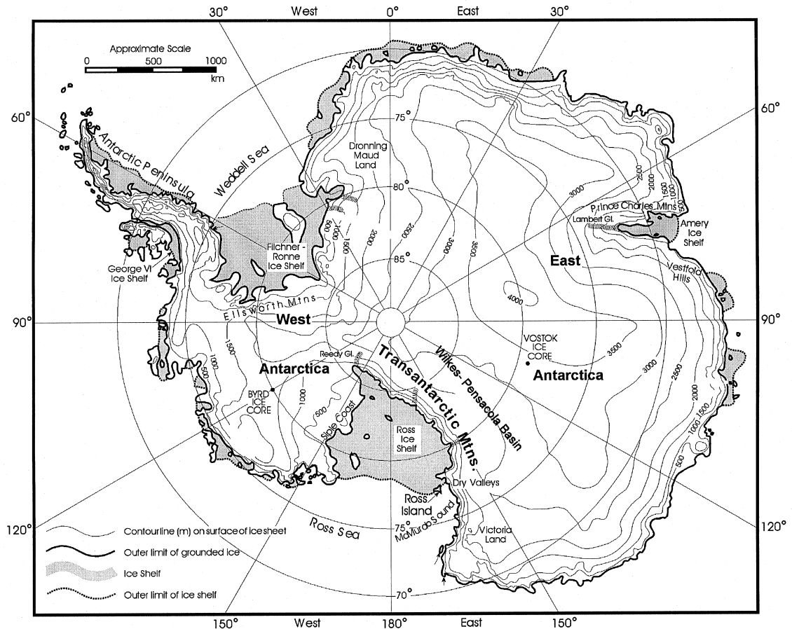
Fig. 1. The present ice surface of Antarctica, showing the major regions mentioned in the paper, including Victoria Land, the Dry Valleys, and the Wilkes–Pensacola Basin. The central ranges of the Transantarctic Mountains, comprising the Queen Alexandra, Queen Elizabeth and Queen Maud Ranges, are situated under the ‘Transantarctic’ of the Transantarctic Mountains caption.
