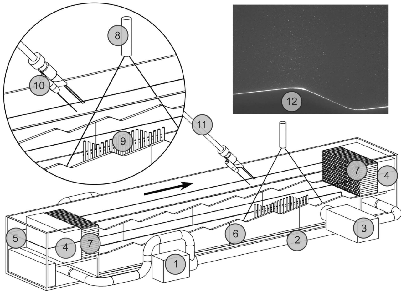
Figure 1. Experimental setup. The numbers correspond to (1) pump, (2) water recirculation line, (3) fast shutter camera used for particle image velocimetry (PIV), (4) polyester filter foam, (5) water surface, (6) ripple stencil, (7) polycarbonate honeycomb flow rectifier, (8) line laser for projecting vertical laser sheet for PIV, (9) pressure ports on support plate, (10) sensor head with injection needle and two fiber-optic fluorescence sensors, (11) rod controlled by precision gears, and (12) sample PIV image of neutrally buoyant particles taken by (3) and illuminated by (8).
