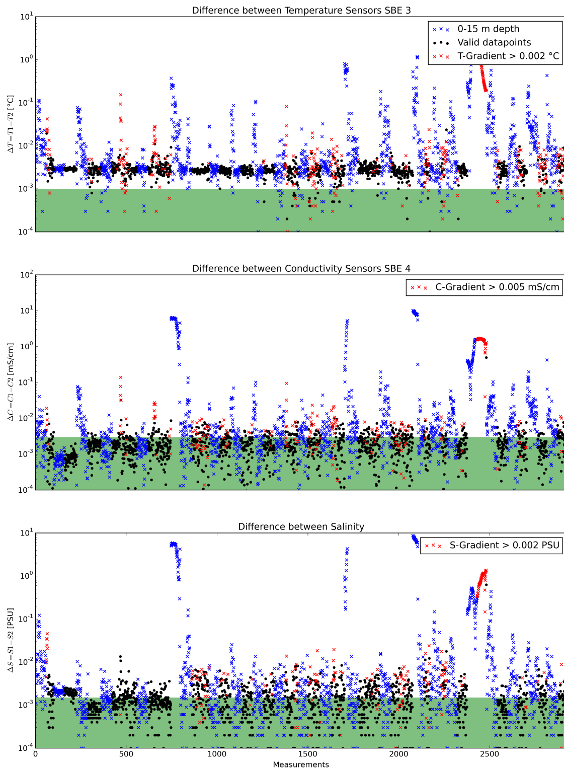
Figure 2: Data accuracy of sensor pairs HE447
