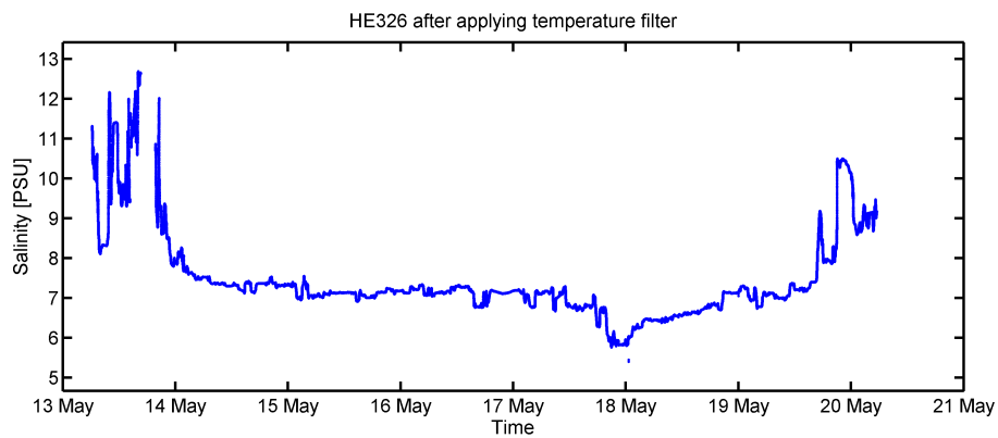
Figure 7: Salinity after temperature filter.
