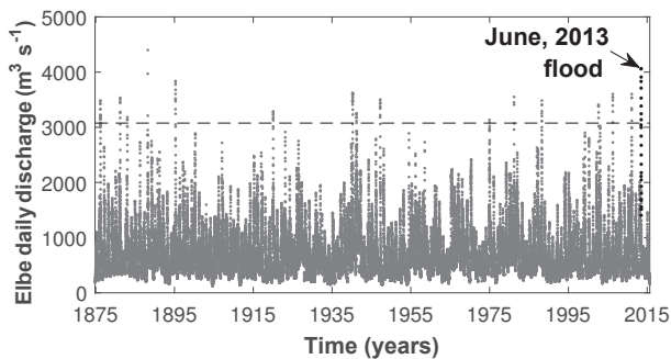
Figure 2. Daily discharge from the Elbe River between 1874 and 2015. The dashed black line indicates the level of 10-year flood, as listed in Table 2. The June 2013 flood is highlighted in black and indicated with an arrow.
