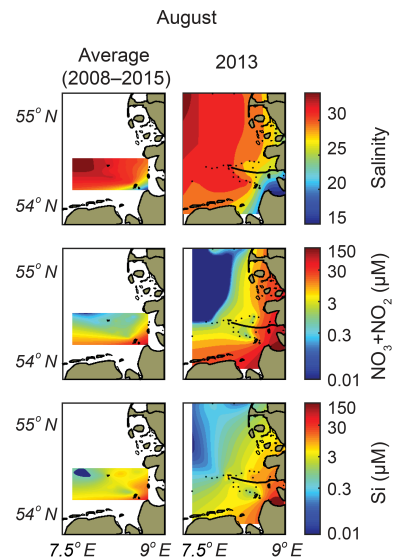
Figure 12. Same description as in Fig. 10, for the month of August. The left panels show average parameter distributions in August, based on 7 years of data (2008–2015, excluding 2013) from BAH AWI stations (Table 1); the right panels show interpolated parameters from 6 to 12 August, 2013, measured at BAH AWI, BSH, FerryBox and HPA stations (Tables 1 and 4).
