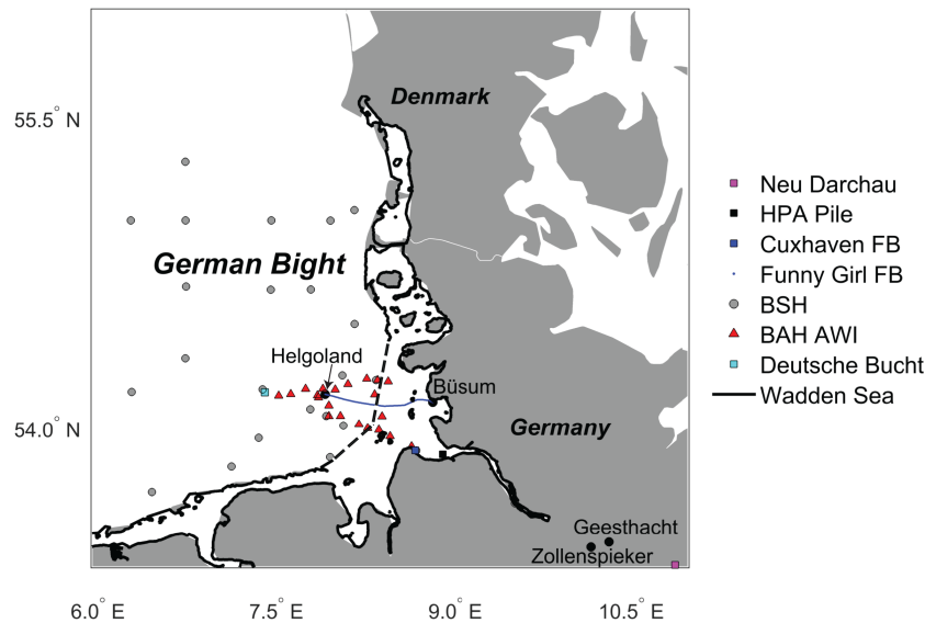
Figure 1. Map of German Bight, Elbe estuary, Wadden Sea and the continental regions around them. Stations are indicated with different symbols: Neu Darchau discharge gauging station (magenta square), operated by the German Federal Waterways and Shipping Administration (WSV); HPA pile (black square), operated by Bundesamt für Seeschifffahrt und Hydrographie (BSH) and Helmholtz-Zentrum Geesthacht (HZG); Cuxhaven FerryBox (FB, blue square), operated by HZG; M/V Funny Girl FB transect (blue line) between Büsum and Helgoland, operated by HZG; BSH discrete sampling stations (grey circles); Biological Station Helgoland at the Alfred Wegener Institute (BAH AWI) discrete sampling stations (red triangles); Deutsche Bucht MARNET monitoring station, operated by BSH (cyan square). The Wadden Sea outline was obtained as a shape file from Claus et al. (2016), and the dashed line represents the imaginary boundary of the shapefile rather than the Wadden Sea.
