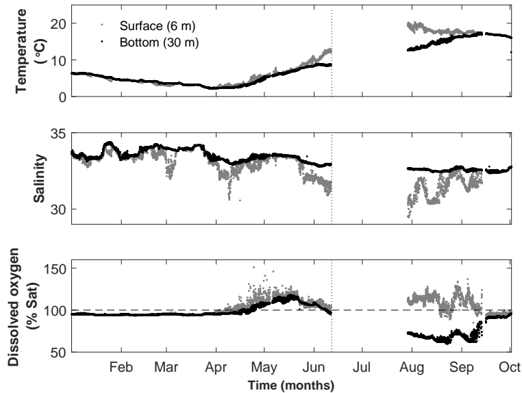
Figure 13. Surface (6 m, gray) and bottom (30 m, black) temperature, salinity and dissolved oxygen (% saturation) measured at the Deutsche Bucht station (Fig. 1, Table 1), part of the MARNET monitoring network. The data cover a time frame between January and October 2013. The onset of the June flood is marked by a vertical line.
