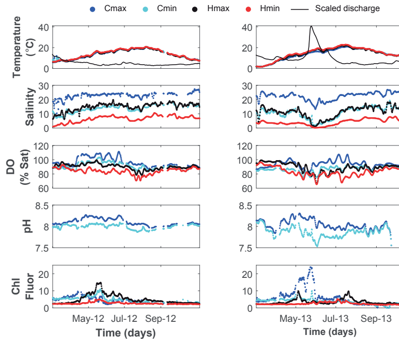
Figure 5. Temperature, salinity, DO (% saturation), pH and chlorophyll (fluorescence) measured at Cuxhaven and HPA pile in the Elbe estuary, for 2012 (left panels) and 2013 (right panels). The colors represent the data identified for each parameter, and at each station, at the times of salinity maxima (Cmax at Cuxhaven, blue; Hmax at HPA pile, black) and salinity minima (Cmin at Cuxhaven, cyan; Hmin at HPA pile, red). As a reference, the Elbe River discharge (originally measured in \text{m}^3 \text{s}^{-1} ) at Neu Darchau station (Fig. 1) was scaled by dividing it by 100 and was included in the temperature plots.
