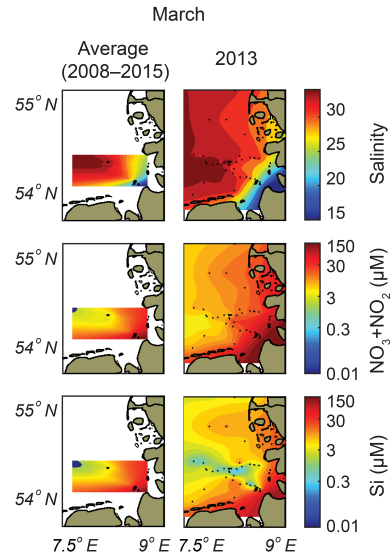
Figure 10. Maps of interpolated (Kriging method of interpolation) salinity, nitrate + nitrite ( \text{NO}_3 + \text{NO}_2 , \mu\text{M} ) and silicate ( \text{Si} , \mu\text{M} ) for the month of March. The left panels show average parameter distributions in March, based on 7 years of data (2008–2015, excluding 2013) from BAH AWI stations (Table 1); the right panels show interpolated parameters from 15 to 27 March 2013, measured at BAH AWI, BSH, FerryBox and HPA stations (Tables 1 and 4).
