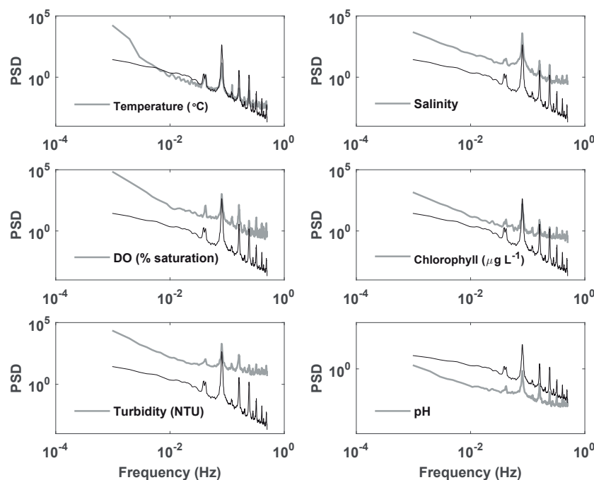
Figure 4. Power spectral density (PSD) plots (gray) of six parameters measured at the Cuxhaven FerryBox station (temperature, salinity, DO, chlorophyll, turbidity and pH). Also shown on each panel in black is the PSD for sea level measured at a station near Cuxhaven.
