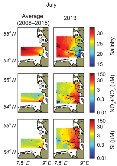
Figure 11. Same description as in Fig. 10, for the month of July. The left panels show average parameter distributions in July, based on 7 years of data (2008–2015, excluding 2013) from BAH AWI stations (Table 1); the right panels show interpolated parameters from 2 to 11 July 2013, measured at BAH AWI, BSH, FerryBox and HPA stations (Tables 1 and 4).
