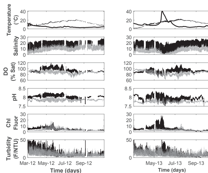
Figure 3. Hourly measurements of temperature, salinity, DO (% saturation), pH, chlorophyll (fluorescence) and turbidity (F/NTU), measured at Cuxhaven (725 river km, black line) and HPA pile (710 river km, gray line) in the Elbe estuary, for 2012 (left panels) and 2013 (right panels). As a reference, the Elbe discharge ( \text{m}^3 \text{ s}^{-1} ) at Neu Darchau station (thick black line), scaled by dividing it by 100, was also included in the temperature plots.
