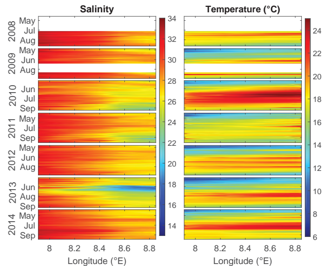
Figure 8. Salinity (left) and temperature (right) between Büsum and Helgoland for each summer between 2008 and 2014, collected by the M/V Funny Girl FerryBox. The ferry transect is shown in Fig. 1.
