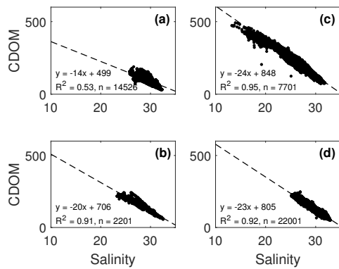
Figure 7. Salinity vs. CDOM fluorescence from M/V Funny Girl for the period between 2012 and 2014 (summer seasons): (a) 2012, (b) before the 2013 flood, (c) during and after the 2013 flood and (d) 2014.
