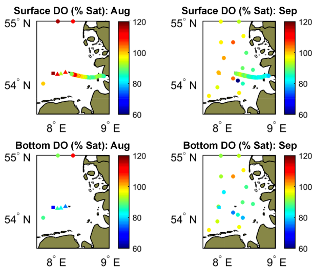
Figure 14. Dissolved oxygen (% saturation) in surface and bottom waters measured in August and September 2013. The surface and bottom dissolved oxygen were measured at available discrete stations from AWI and BSH stations, along with FerryBox (M/V Funny Girl ) and Deutsche Bucht MARNET station. The dates of coverage are listed in Table 4.
