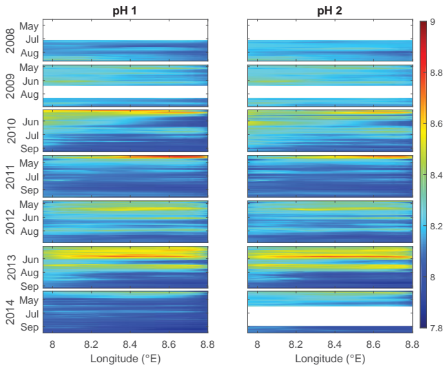
Figure 9. pH ferry data between Büsum and Helgoland for each summer between 2008 and 2014. There were two pH probes available on the ferry M/V Funny Girl . The white sections represent times when data were not available.
