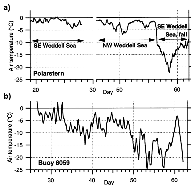
Fig. 3. Air temperatures recorded on board Polarstern along the cruise track in 1997 (a) and by a drifting buoy (Argos ID 8059) at about 40^{\circ}\text{W} , 73.2^{\circ}\text{S} in the southeast Weddell Sea (b).
