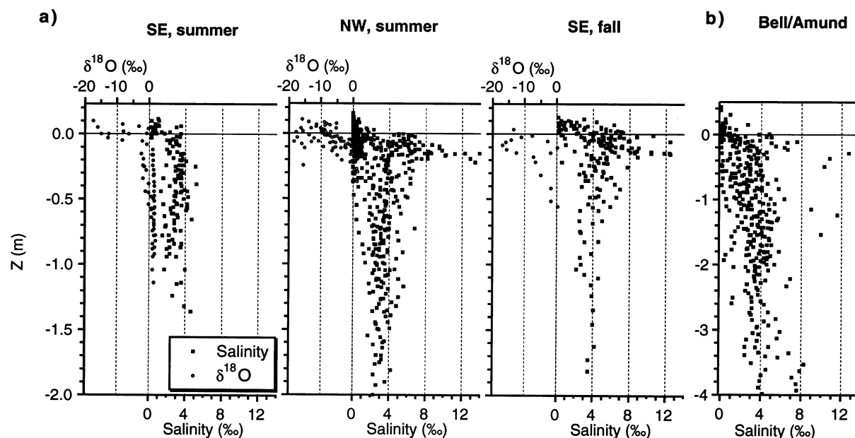
Fig. 7. Salinity and \delta^{18}\text{O} profiles of all surface and main cores obtained in 1994 and 1997 plotted at centre position of individual core segments with respect to the water level ( z = 0.0 m).
