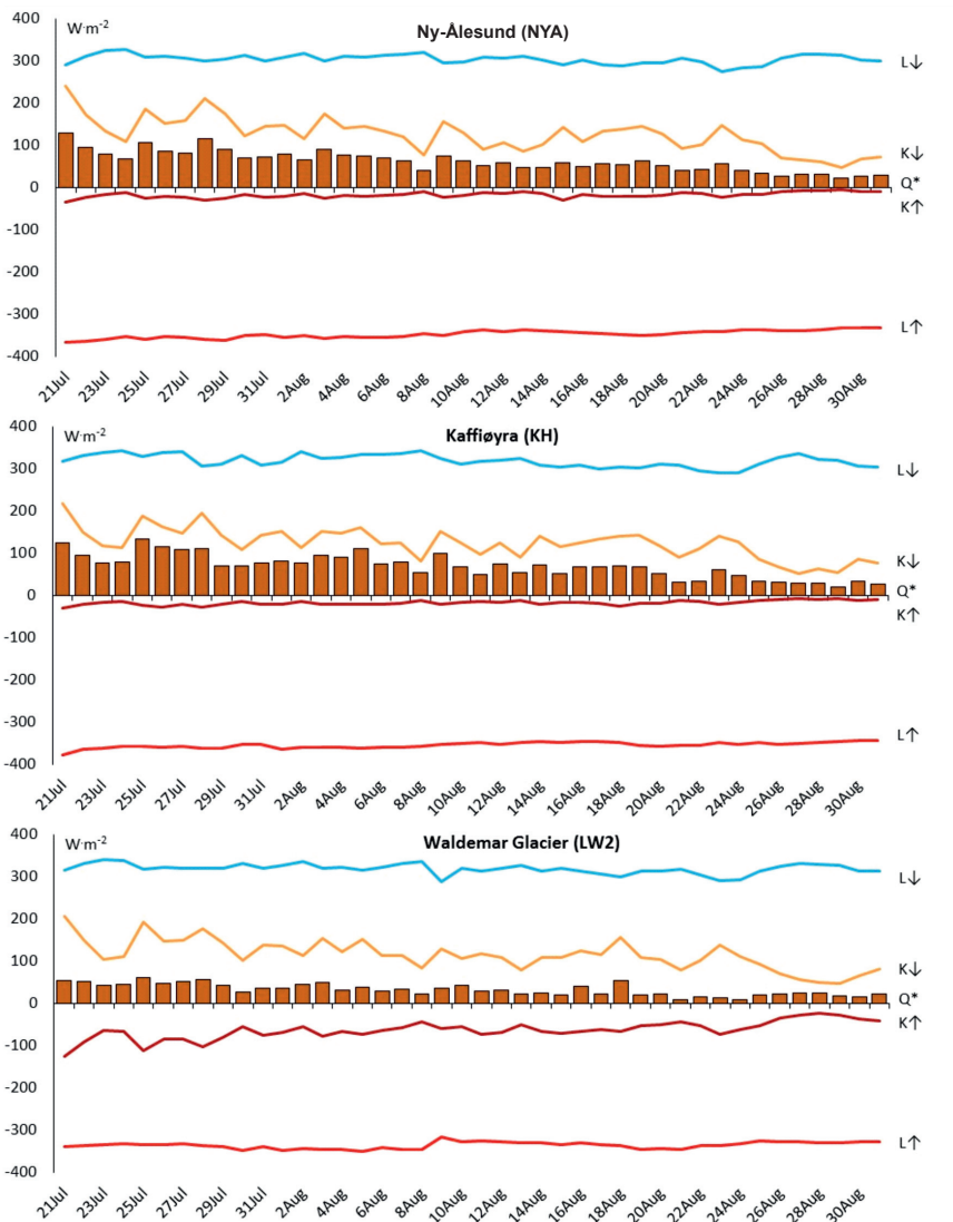
Fig. 4. Mean course of radiation balance fluxes on Ny-Ålesund, Kaffiøyra and Waldemar Glacier in the period 21 July – 31 August in the years 2010–2014. Symbol explanations on page 62.
