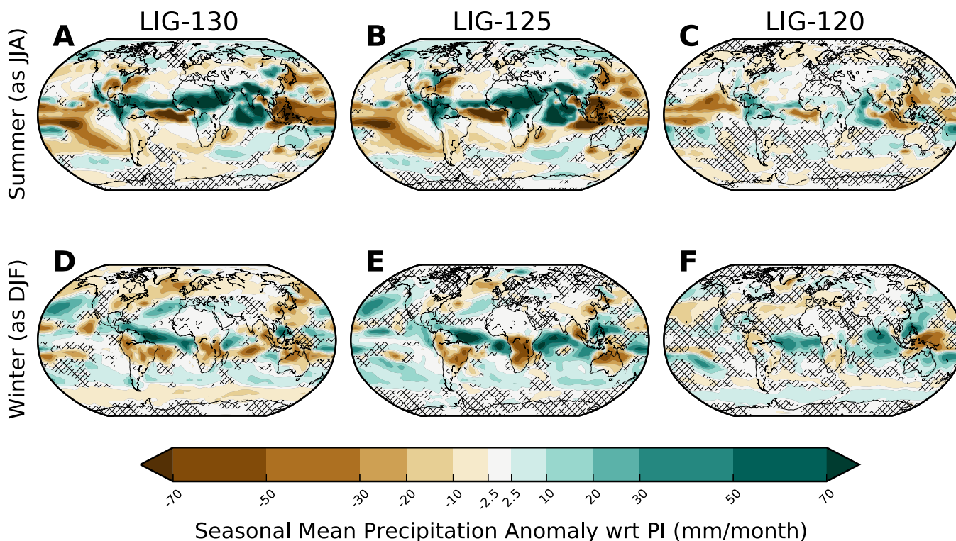
Figure 5. Anomalous summer and winter precipitation amounts relative to PI.
