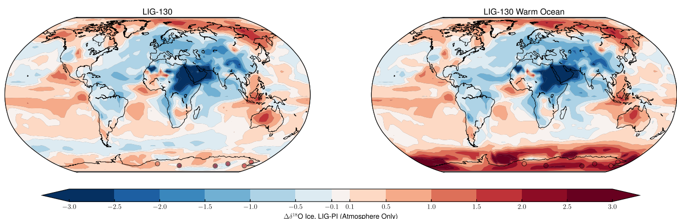
Figure 10. Results of a sensitivity test, warming the Southern Ocean by 2^\circ\text{C} . The model-data mismatch between the ice core measurements and the simulation reduces considerably.
