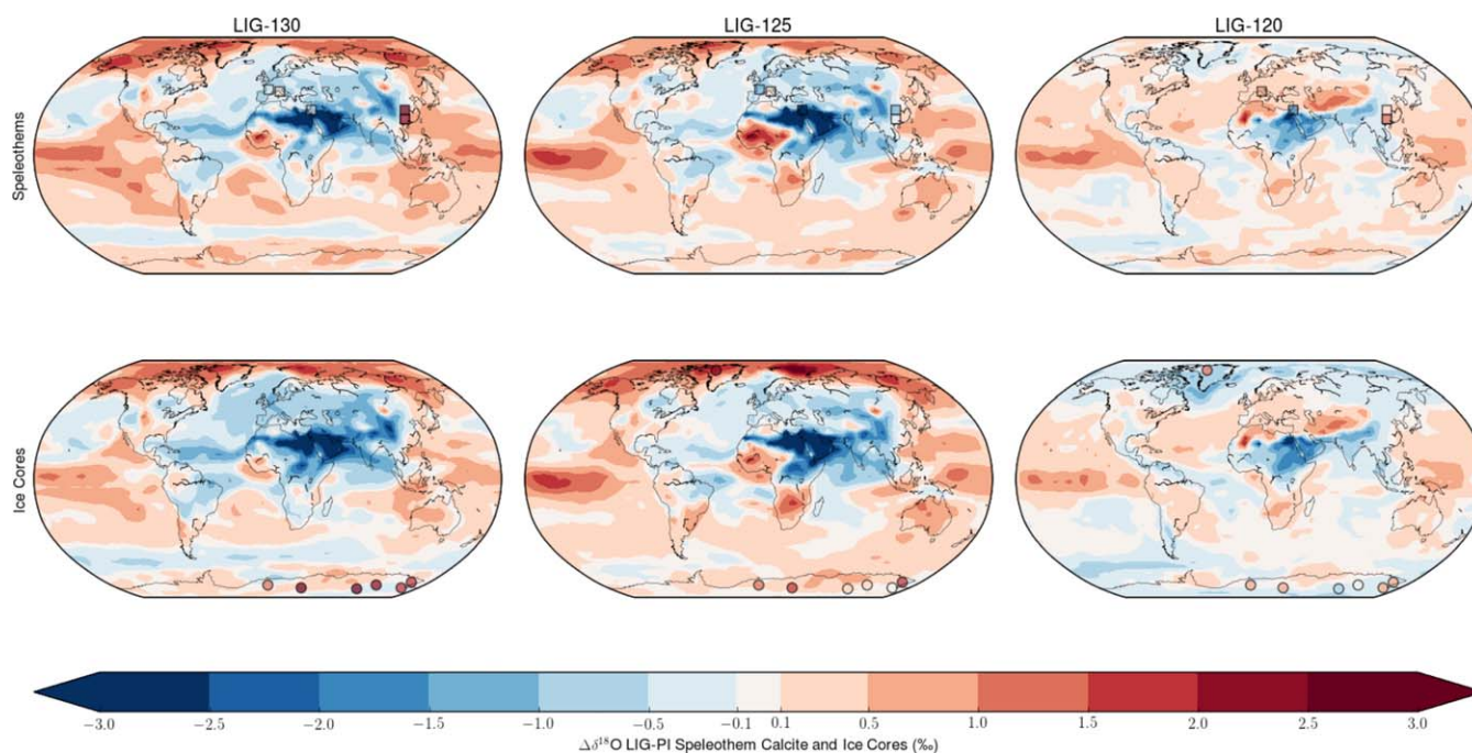
Figure 8. Comparison of six Antarctic ice cores (circles), one Greenland ice core (circles), and several speleothem records (squares) to isotopic values simulated by ECHAM5/MPIOM-wiso. In order to compensate for potential age uncertainties, each comparison is made against a 1000 year average for the paleoclimate record (for LIG-130, ages from 130.5 to 129.5 ka B.P. were chosen in the ice core, etc.).
