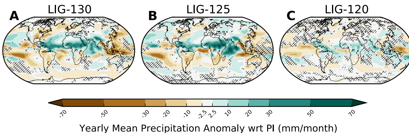
Figure 4. As Figure 2, but showing yearly averaged total precipitation.
