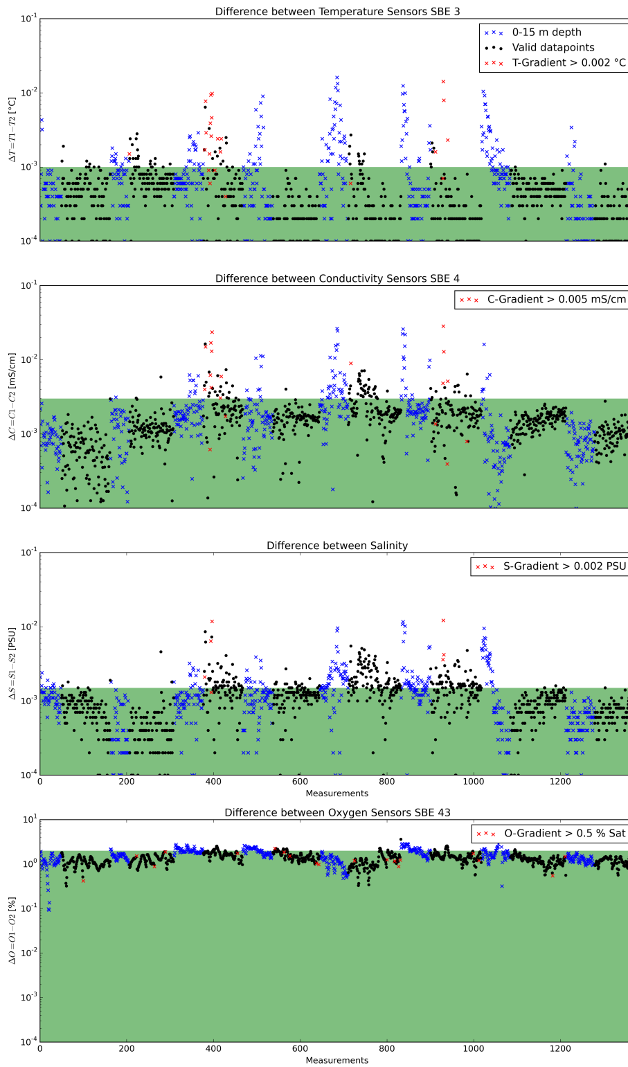
Figure 2: Data accuracy of sensor pairs HE496
