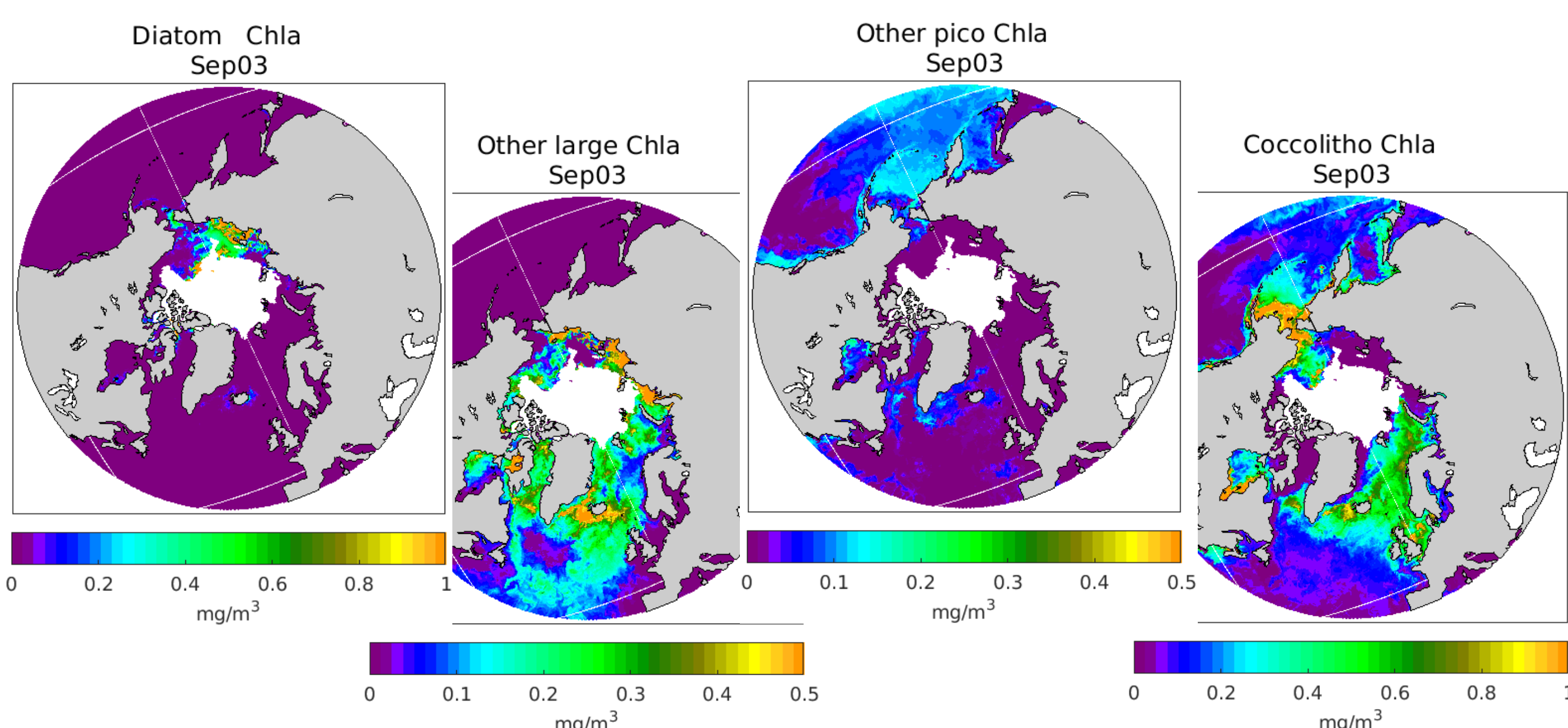
Figure: Spatial distribution of the model simulated Arctic chlorophyll “a” for diatoms, other large phytoplankton, pico-phytoplankton (including small diatoms) and coccolithophores in September 2003.
