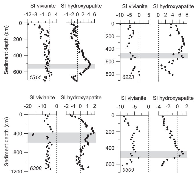
Fig. 7. PHREEQC calculations of pore water saturation indices (SI) for vivianite and hydroxyapatite at sites GeoB 1514, 6223, 6308 and 9309. Grey bar indicates sulphidic zone within the SMT.
