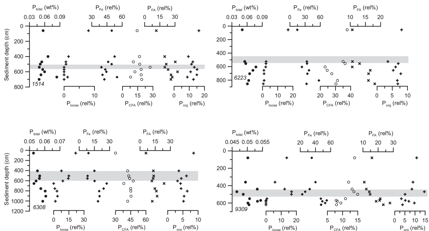
Fig. 6. Contents of different extracted P fractions ( P_{\text{loose}} = hydroxyapatite, octocalcium-phosphate; P_{\text{Fe}} = Fe-bound P; P_{\text{CFA}} = carbonate fluorapatite; P_{\text{FA}} = fluorapatite; P_{\text{org}} = organic P) in rel% of P_{\text{total}} at the four studied sites.
