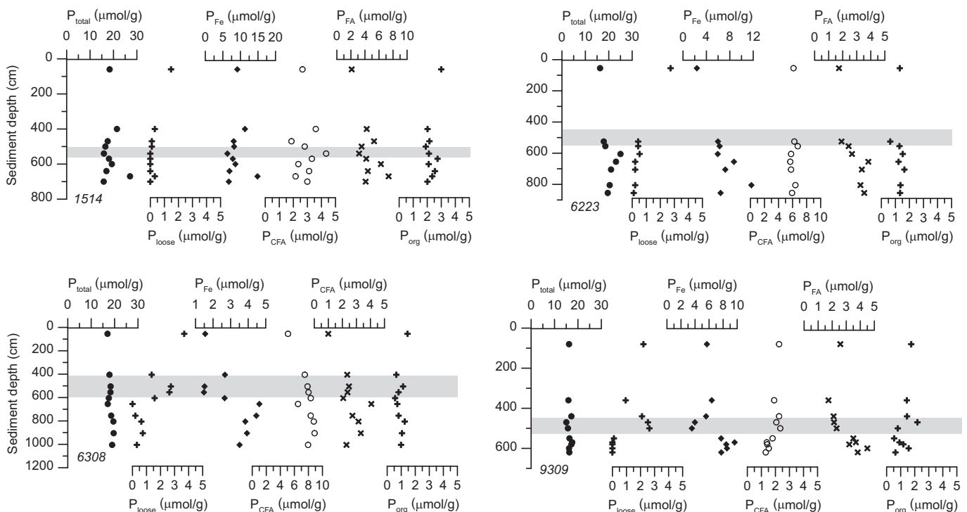
Fig. 5. Contents of different extracted P fractions ( P_{loose} = hydroxyapatite, octocalcium-phosphate; P_{Fe} = Fe-bound P; P_{CFA} = carbonate fluorapatite; P_{FA} = fluorapatite; P_{org} = organic P) in \mu\text{mol/g} of dry sediment at the four studied sites.
