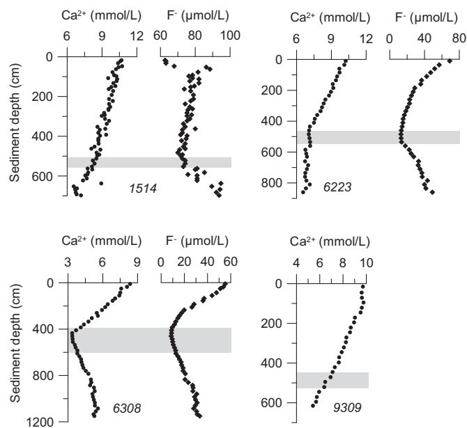
Fig. 3. Pore water concentrations of \text{Ca}^{2+} (mmol/l) and \text{F}^- ( \mu\text{mol/l} ) in cores GeoB 1514, 6223, 6308 and 9309 (no \text{F}^- data available for 9309). Grey bar indicates sulphidic zone within the SMT.
