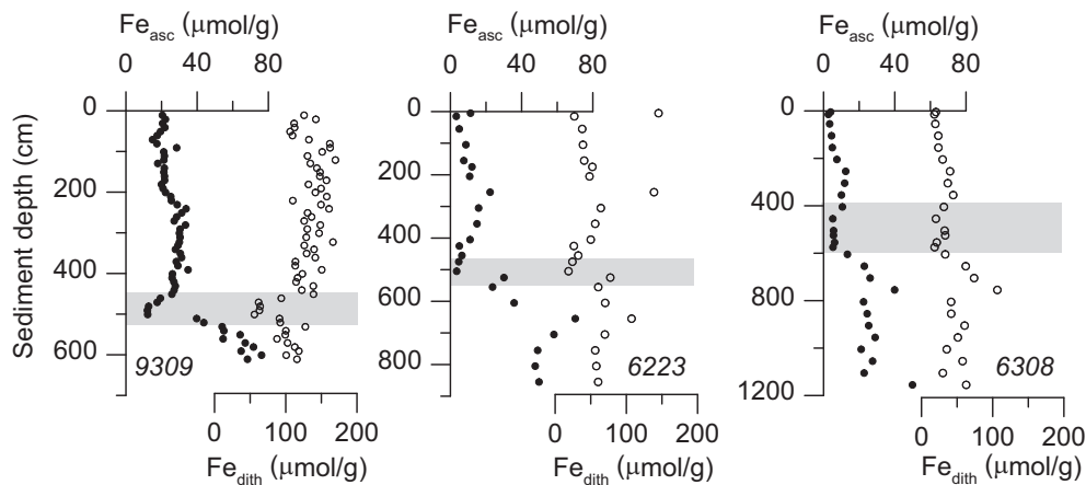
Fig. 4. Contents of Fe_{asc} (amorphous/poorly crystalline Fe (oxyhydr)oxides; filled circles) and Fe_{dith} (crystalline Fe oxides; open circles) fractions (no data for GeoB 1514) in \mu\text{mol/g} of dry sediment. Grey bar indicates sulphidic zone within the SMT.
