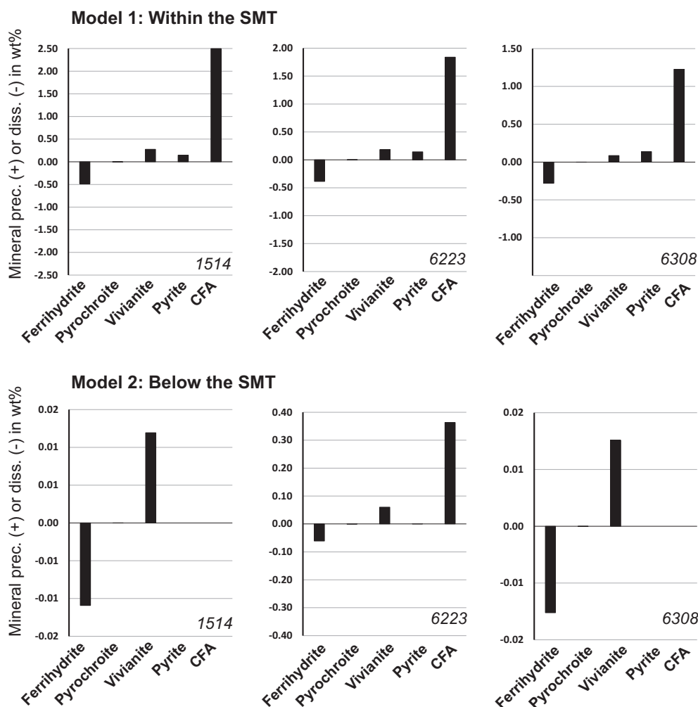
Fig. 8. Estimated amounts of mineral dissolution and precipitation in the inverse models performed in PHREEQC for sites GeoB 1514, 6223 and 6308.
