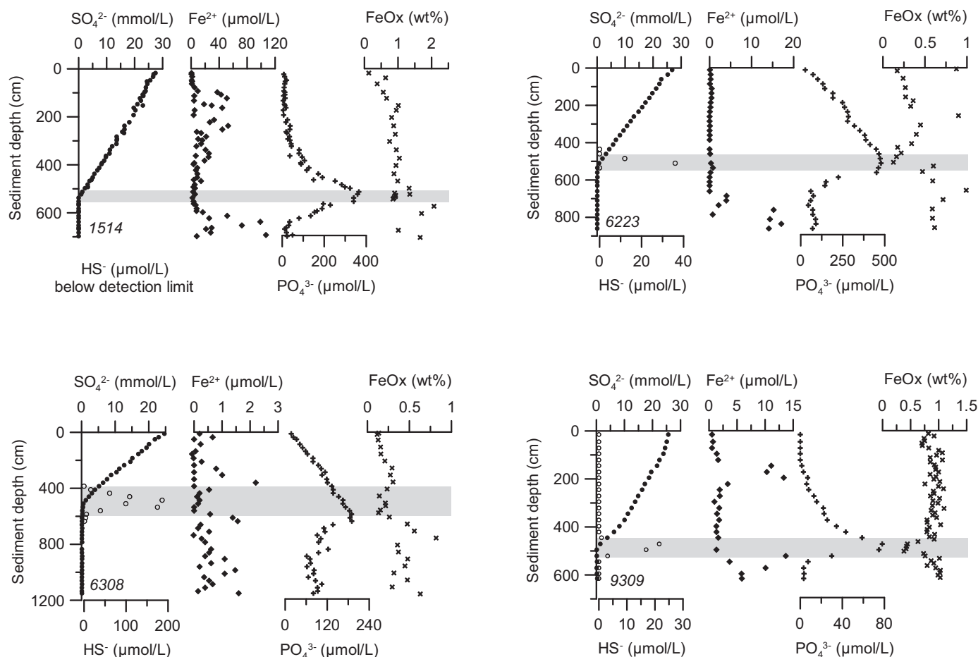
Fig. 2. Pore water concentrations of \text{SO}_4^{2-} (mmol/l), \text{HS}^- ( \mu\text{mol/l} ), \text{Fe}^{2+} ( \mu\text{mol/l} ), \text{PO}_4^{3-} ( \mu\text{mol/l} ) and Fe (oxyhydr)oxides (FeOx, sum of \text{Fe}_{\text{asc}} and \text{Fe}_{\text{dith}} fractions) (wt% of dry sediment) in cores GeoB 1514, 6223, 6308 and 9309. Grey bar indicates sulphidic zone within the SMT.
