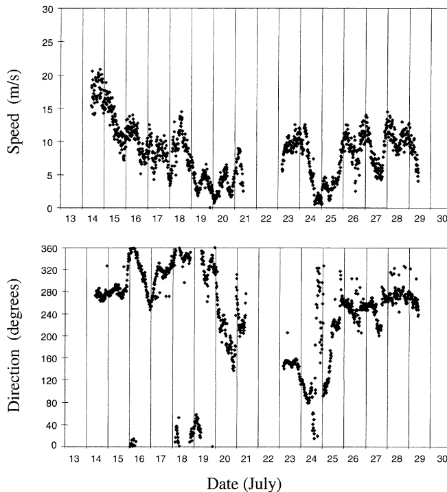
Fig. 4 Wind speed and direction over the Alkor Deep during KATTEX I
