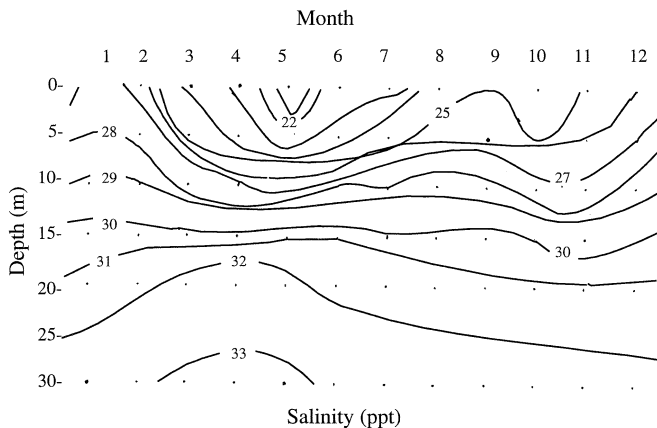
Fig. 2 Long-term monthly means of salinity measured at LV Læsø Trindel (from Svansson 1975)
